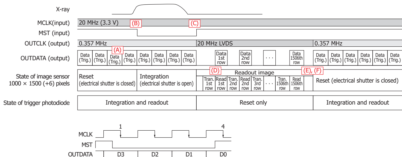
Total timing chart
