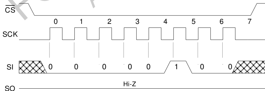
Figure 14. WRDI Bus Configuration
