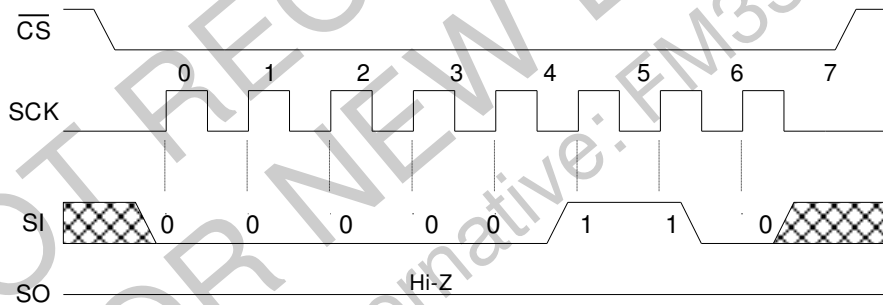
Figure 13. WREN Bus Configuration
