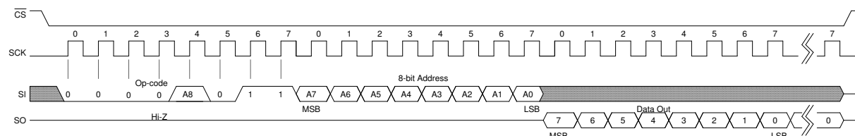
Figure 10. Memory Read
