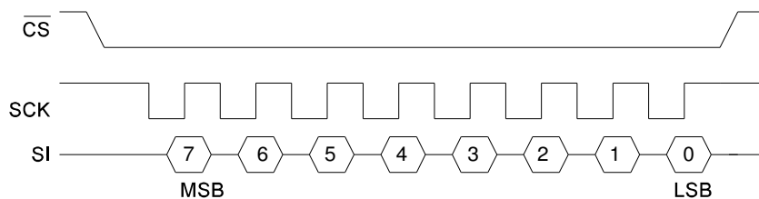
Figure 4. SPI Modes 0 & 3
