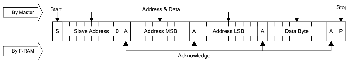
Figure 5. Byte Write
