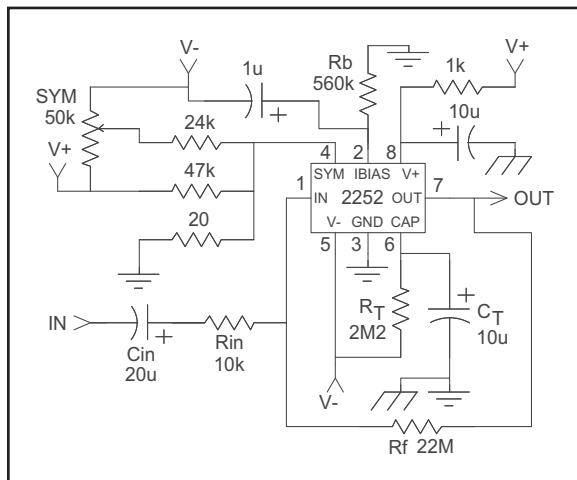
Figure 4. Typical Application Circuit (±15V)
