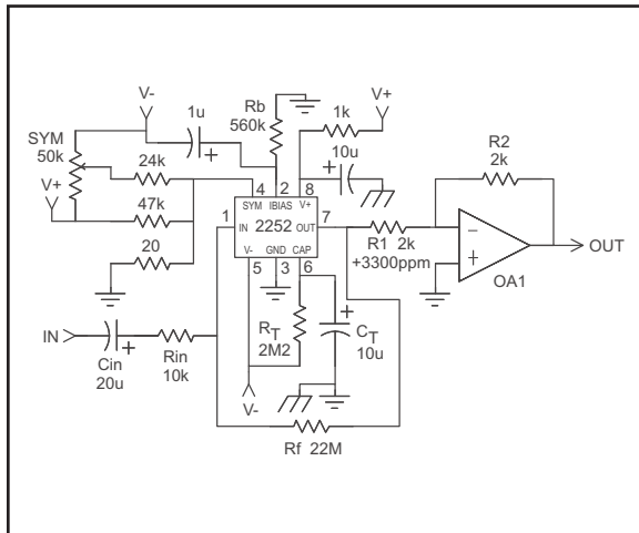
Figure 13. Temperature Compensating the 2252
