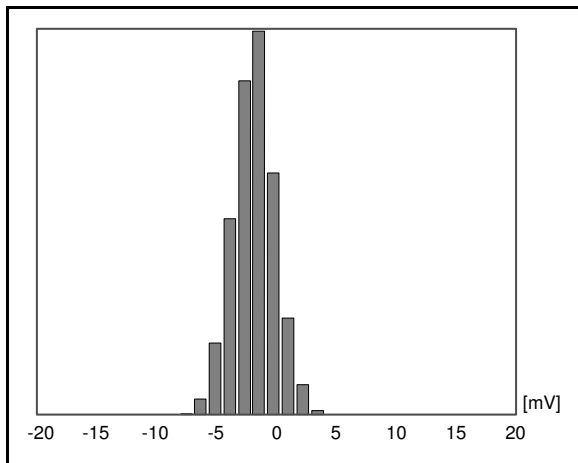
Figure 10. Representative Output Offset Voltage Distribution, 0dB Gain
