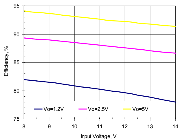
Figure 4. Efficiency vs. Input Voltage. Iout=5A, Fsw=500kHz
