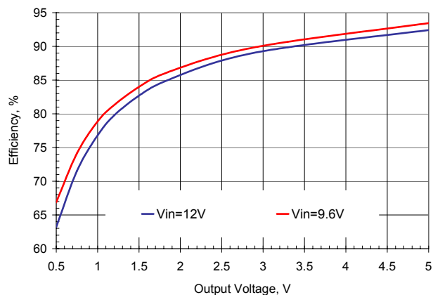
Figure 3. Efficiency vs. Output Voltage, Iout=5A, Fsw=500kHz
