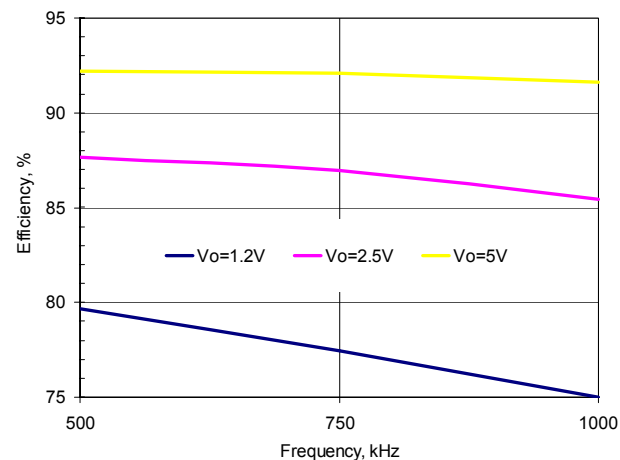
Figure 5. Efficiency vs. Switching Frequency. Iout=5A
