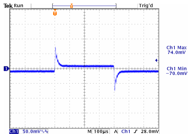
Figure 12. Vin=12V, Vout=5.0V
