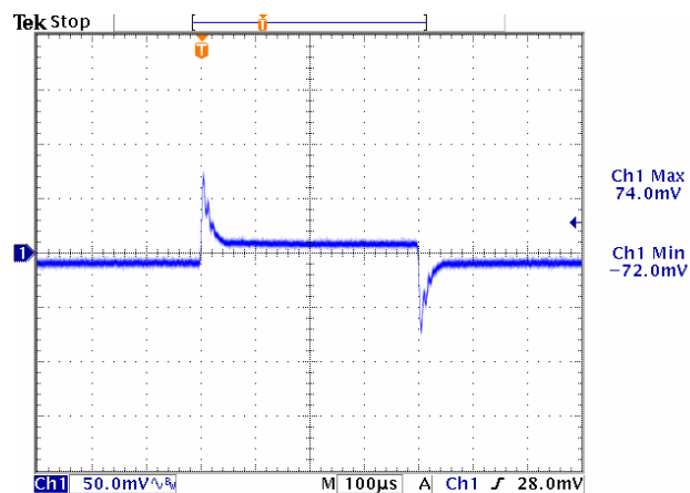
Figure 13. Vin=12V, Vout=2.5V
