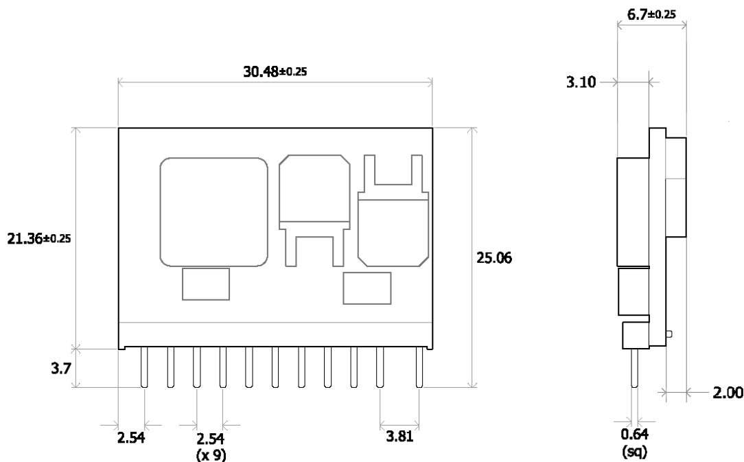
Figure 46. Mechanical Drawing
