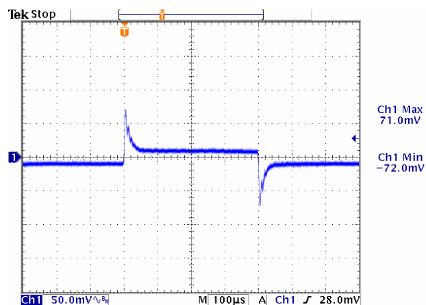
Figure 14. Vin=12V, Vout=1.0V
