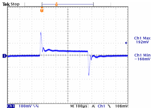
Figure 12. Vin=12V, Vout=5.0V
