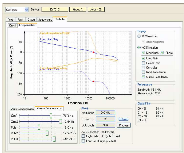
Figure 47. PWM Controller Window
