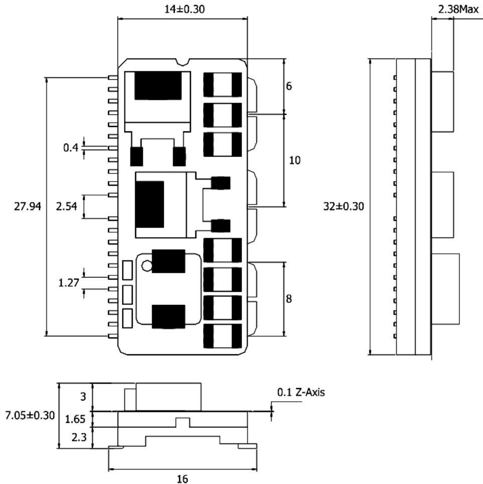
Figure 57. Mechanical Drawing
