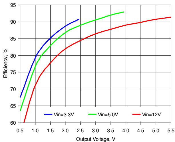
Figure 5. Efficiency vs. Output Voltage, Iout=10A, Fsw=500kHz
