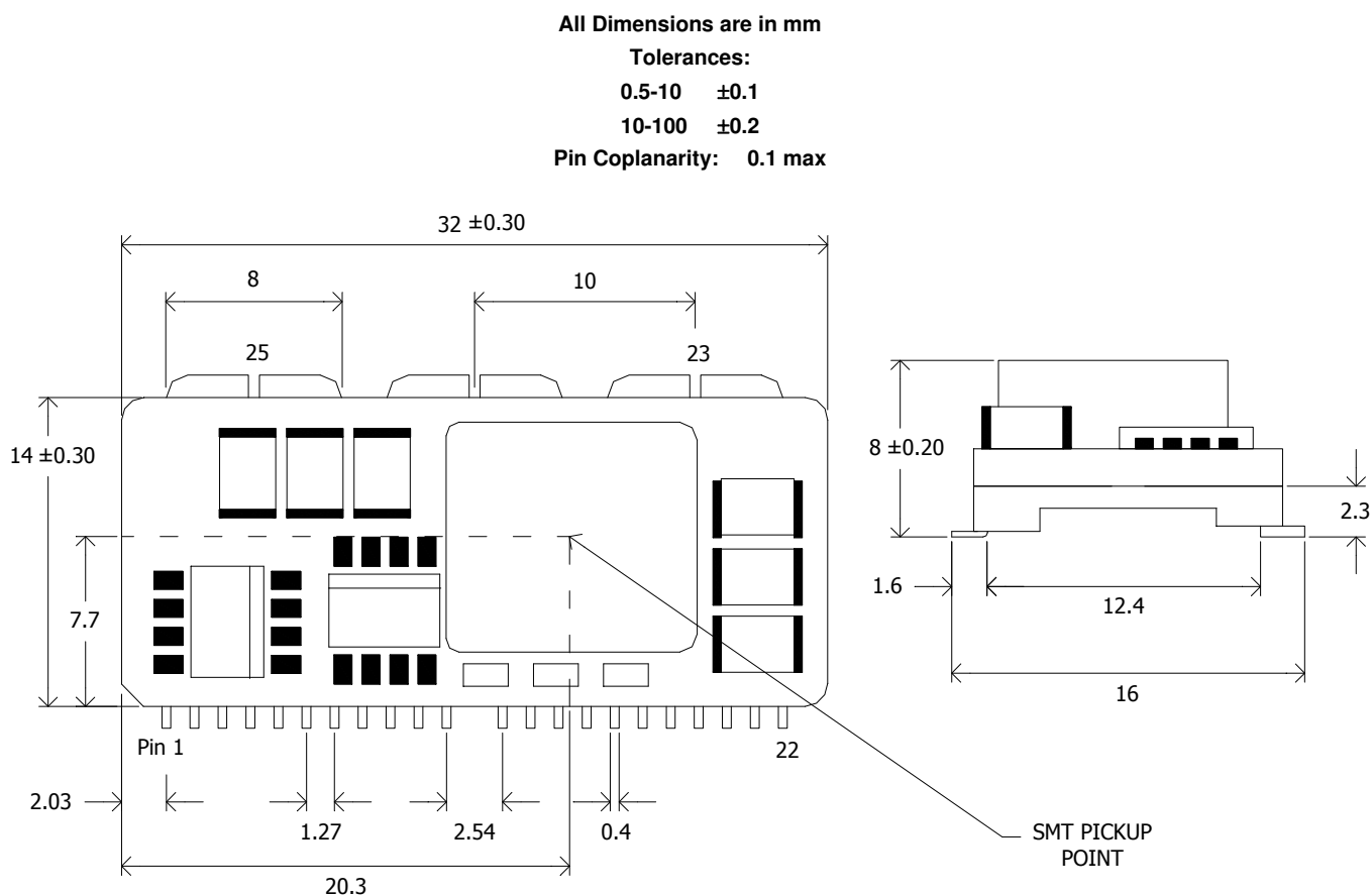
Figure 57. Mechanical Drawing
