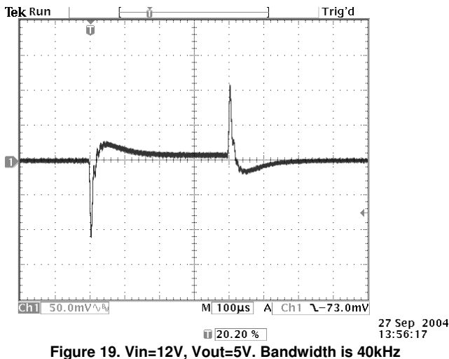
Figure 19. Vin=12V, Vout=5V. Bandwidth is 40kHz
