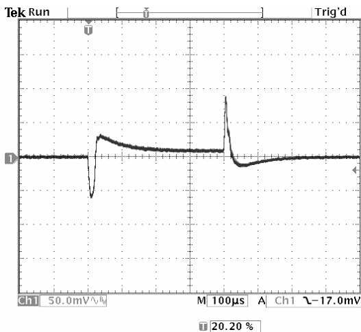
Figure 18. Vin=12V, Vout=1V. Bandwidth is 40kHz
