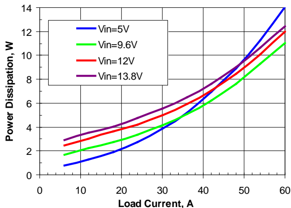
Figure 9. Power Dissipation vs. Load. Vout=1.8V
