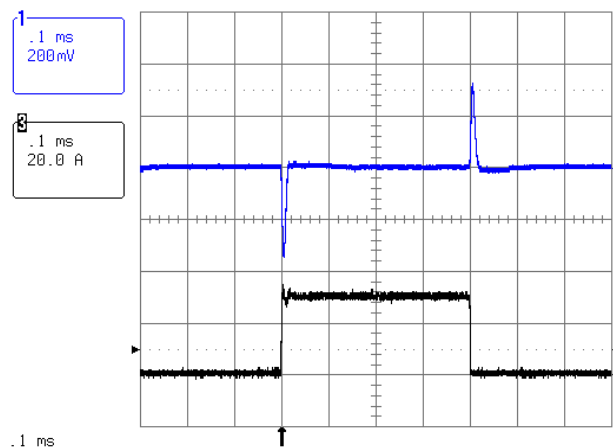
Figure 12. Transient Response to Dynamic Load Change from 0% to 50% of full load ( V_{in} = 12\text{ V} , V_o = 1.5\text{ V} ). Ch1 – Vout, Ch3 – Iout
