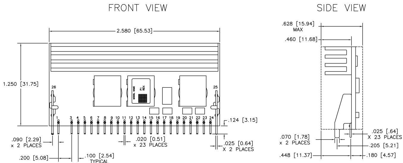
Figure 11. Mechanical Drawing
