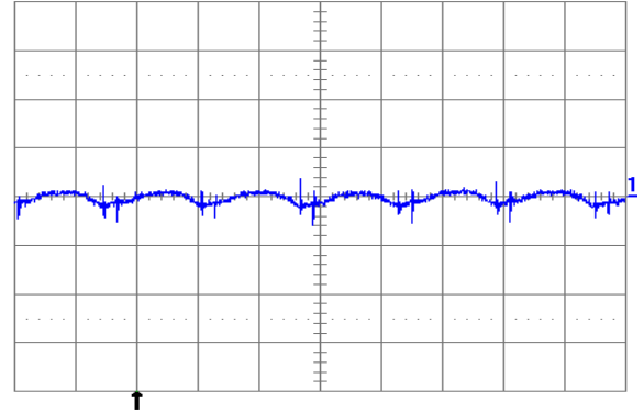
Fig. 1.5V.6: Output voltage ripple (20mV/div.) at full rated load current into a resistive load with external capacitance 100\mu F ceramic and V_{in} = 12V for V_{out} = 1.5V . Time scale: 2 \mu s /div.
