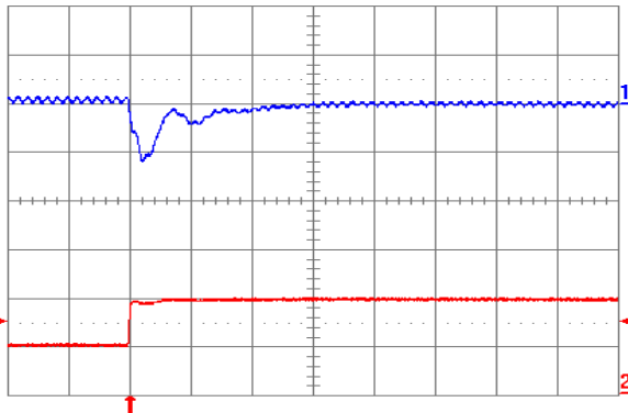
Fig. 1.2V.7: Output voltage response (YNV05T10012) to positive load current step change from 2.5A to 5A with slew rate of 5A/ \mu s at V_{in} = 5V. Top trace: output voltage (100mV/div.); Bottom trace: load current (5A/div.). C_o = 100 \mu F ceramic + 1 \mu F ceramic. Time scale: 20 \mu s/div.
