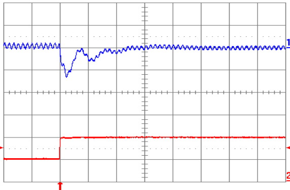
Fig. 2.5V.7: Output voltage response (YNV05T10025) to positive load current step change from 2.5A to 5A with slew rate of 5A/ \mu s at V_{in} = 5V. Top trace: output voltage (100mV/div.); Bottom trace: load current (5A/div.). C_o = 100 \mu F ceramic + 1 \mu F ceramic. Time scale: 20 \mu s/div.
