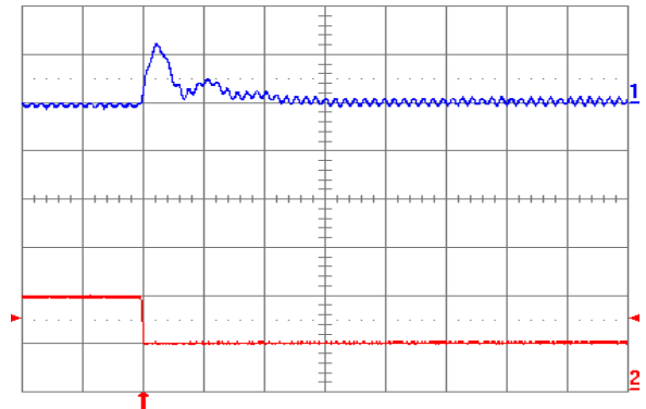
Fig. 1.5V.8: Output voltage response (YNV05T10015) to negative load current step change from 5A to 2.5A with slew rate of -5A/ \mu s at V_{in} = 5V . Top trace: output voltage (100mV/div.); Bottom trace: load current (5A/div.). C_o = 100\mu F ceramic + 1 \mu F ceramic. Time scale: 20 \mu s/div.
