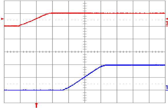
Fig. 2.0V.5: Turn-on transient (YNV05T10020) with application of V_{in} at full rated load current (resistive) and 47 \mu F external capacitance at V_{in} = 5V. Top trace: V_{in} (5V/div.); Bottom trace: output voltage (1V/div.); Time scale: 2ms/div.
