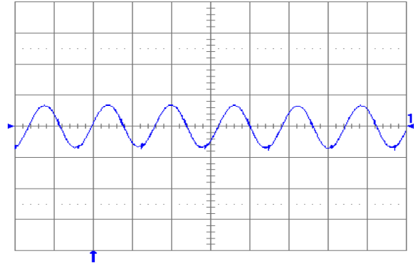
Fig. 1.5V.6: Output voltage ripple (20mV/div.) at full rated load current into a resistive load with external capacitance 47 \mu F ceramic + 1 \mu F ceramic and V_{in} = 5V (YNV05T10015). Time scale: 2 \mu s/div.
