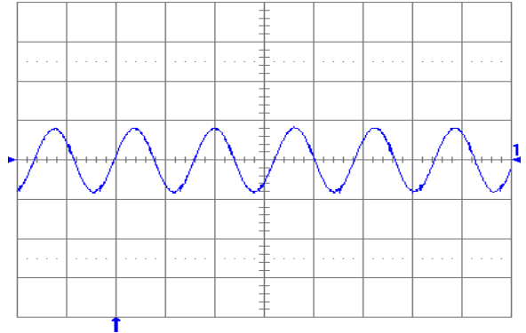
Fig. 1.8V.6: Output voltage ripple (20mV/div.) at full rated load current into a resistive load with external capacitance 47 \mu F ceramic + 1 \mu F ceramic and V_{in} = 5V (YNV05T10018). Time scale: 2 \mu s/div.
