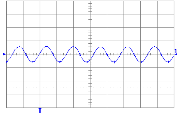
Fig. 1.2V.6: Output voltage ripple (20mV/div.) at full rated load current into a resistive load with external capacitance 47 \mu F ceramic + 1 \mu F ceramic and V_{in} = 5V (YNV05T10012). Time scale: 2 \mu s/div.
