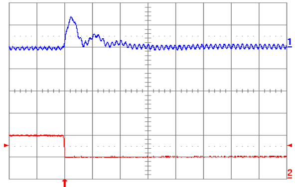
Fig. 2.0V.8: Output voltage response (YNV05T10020) to negative load current step change from 5A to 2.5A with slew rate of -5A/ \mu s at V_{in} = 5V. Top trace: output voltage (100mV/div.); Bottom trace: load current (5A/div.). C_o = 100 \mu F ceramic + 1 \mu F ceramic. Time scale: 20 \mu s/div.
