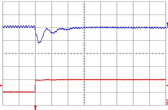
Fig. 1.5V.7: Output voltage response (YNV05T10015) to positive load current step change from 2.5A to 5A with slew rate of 5A/ \mu s at V_{in} = 5V . Top trace: output voltage (100mV/div.); Bottom trace: load current (5A/div.). C_o = 100\mu F ceramic + 1 \mu F ceramic. Time scale: 20 \mu s/div.
