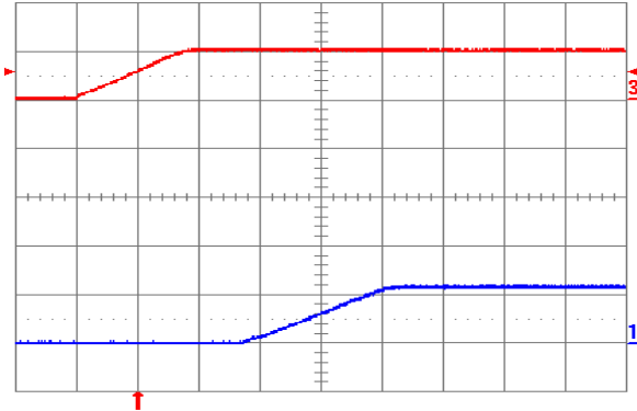
Fig. 1.2V.5: Turn-on transient (YNV05T10012) with application of V_{in} at full rated load current (resistive) and 47 \mu F external capacitance at V_{in} = 5V. Top trace: V_{in} (5V/div.); Bottom trace: output voltage (1V/div.); Time scale: 2ms/div.
