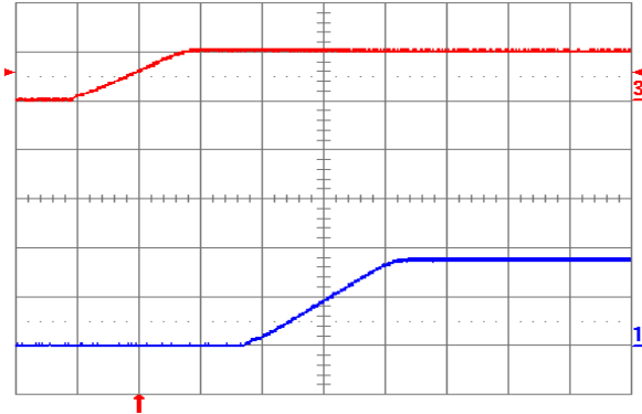
Fig. 1.8V.5: Turn-on transient (YNV05T10018) with application of V_{in} at full rated load current (resistive) and 47 \mu F external capacitance at V_{in} = 5V. Top trace: V_{in} (5V/div.); Bottom trace: output voltage (1V/div.); Time scale: 2ms/div.
