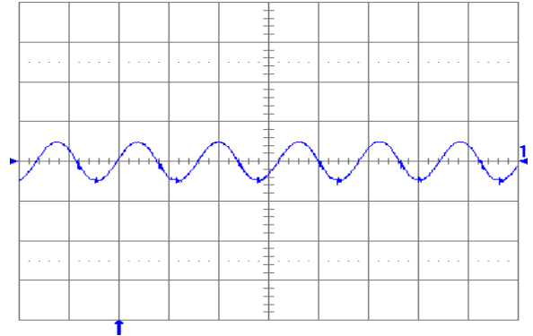
Fig. 0.9V.6: Output voltage ripple (20mV/div.) at full rated load current into a resistive load with external capacitance 47 \mu F ceramic + 1 \mu F ceramic and V_{in} = 5V (YNV05T10009). Time scale: 2 \mu s/div.
