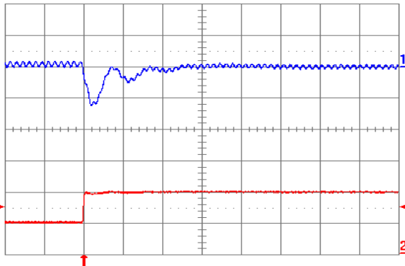
Fig. 1.8V.7: Output voltage response (YNV05T10018) to positive load current step change from 2.5A to 5A with slew rate of 5A/ \mu s at V_{in} = 5V. Top trace: output voltage (100mV/div.); Bottom trace: load current (5A/div.). C_o = 100 \mu F ceramic + 1 \mu F ceramic. Time scale: 20 \mu s/div.
