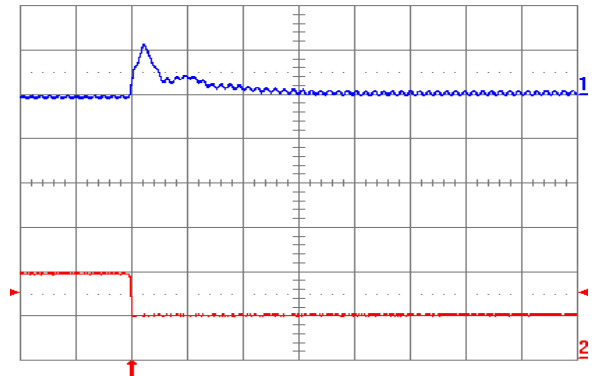
Fig. 0.9V.8: Output voltage response (YNV05T10009) to negative load current step change from 5A to 2.5A with slew rate of -5A/ \mu s at V_{in} = 5V. Top trace: output voltage (100mV/div.); Bottom trace: load current (5A/div.). C_o = 100 \mu F ceramic + 1 \mu F ceramic. Time scale: 20 \mu s/div.
