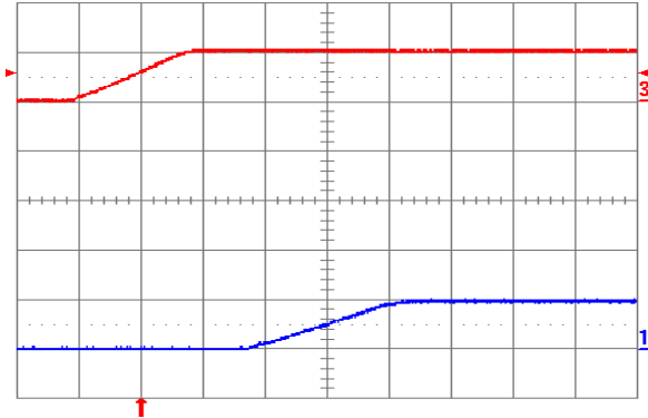
Fig. 1.0V.5: Turn-on transient (YNV05T10010) with application of V_{in} at full rated load current (resistive) and 47 \mu F external capacitance at V_{in} = 5V. Top trace: V_{in} (5V/div.); Bottom trace: output voltage (1V/div.); Time scale: 2ms/div.
