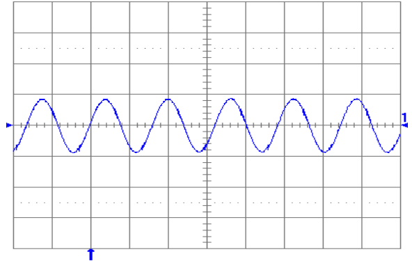
Fig. 2.0V.6: Output voltage ripple (20mV/div.) at full rated load current into a resistive load with external capacitance 47 \mu F ceramic + 1 \mu F ceramic and V_{in} = 5V (YNV05T10020). Time scale: 2 \mu s/div.
