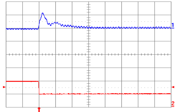
Fig. 1.2V.8: Output voltage response (YNV05T10012) to negative load current step change from 5A to 2.5A with slew rate of -5A/ \mu s at V_{in} = 5V. Top trace: output voltage (100mV/div.); Bottom trace: load current (5A/div.). C_o = 100 \mu F ceramic + 1 \mu F ceramic. Time scale: 20 \mu s/div.
