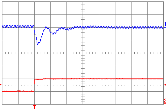
Fig. 2.0V.7: Output voltage response (YNV05T10020) to positive load current step change from 2.5A to 5A with slew rate of 5A/ \mu s at V_{in} = 5V. Top trace: output voltage (100mV/div.); Bottom trace: load current (5A/div.). C_o = 100 \mu F ceramic + 1 \mu F ceramic. Time scale: 20 \mu s/div.
