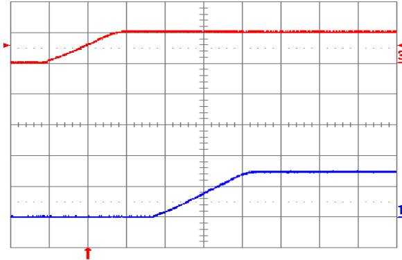
Fig. 1.5V.5: Turn-on transient (YNV05T10015) with application of V_{in} at full rated load current (resistive) and 47 \mu F external capacitance at V_{in} = 5V . Top trace: V_{in} (5V/div.); Bottom trace: output voltage (1V/div.); Time scale: 2ms/div.
