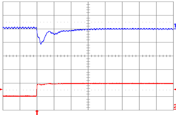
Fig. 1.0V.7: Output voltage response (YNV05T10010) to positive load current step change from 2.5A to 5A with slew rate of 5A/ \mu s at V_{in} = 5V. Top trace: output voltage (100mV/div.); Bottom trace: load current (5A/div.). C_o = 100 \mu F ceramic + 1 \mu F ceramic. Time scale: 20 \mu s/div.
