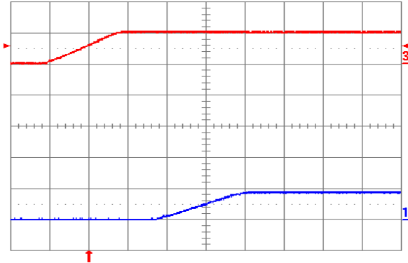
Fig. 0.9V.5: Turn-on transient (YNV05T10009) with application of V_{in} at full rated load current (resistive) and 47 \mu F external capacitance at V_{in} = 5V. Top trace: V_{in} (5V/div.); Bottom trace: output voltage (1V/div.); Time scale: 2ms/div.
