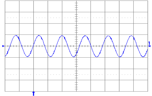
Fig. 2.5V.6: Output voltage ripple (20mV/div.) at full rated load current into a resistive load with external capacitance 47 \mu F ceramic + 1 \mu F ceramic and V_{in} = 5V (YNV05T10025). Time scale: 2 \mu s/div.
