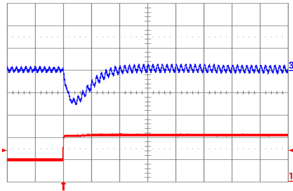
Fig. 5.0V.7: Output voltage response for V_{out} = 5.0 V to positive load current step change from 5 A to 10 A with slew rate of 5 A/ \mu s at V_{in} = 12 V. Top trace: output voltage (100 mV/div.); Bottom trace: load current (5 A/div.). C_o = 100 \mu F ceramic. Time scale: 20 \mu s/div.
