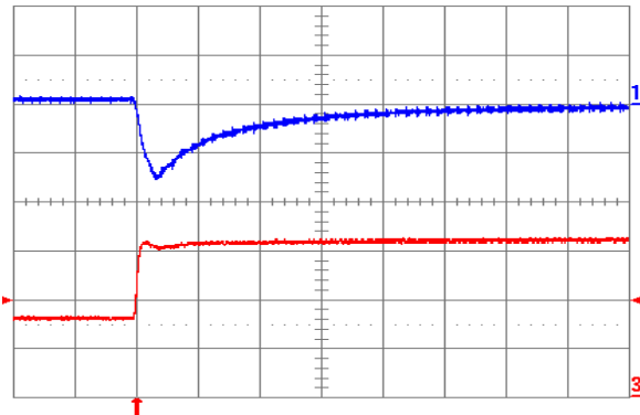
Fig. 0.7525V.7: Output voltage response for V_{out} = 0.7525 V to positive load current step change from 8 A to 16 A with slew rate of 5 \text{ A}/\mu\text{s} at V_{in} = 5 V. Top trace: output voltage (100 mV/div.); Bottom trace: load current (5 A/div.). C_o = 100 \mu\text{F} ceramic. Time scale: 20 \mu\text{s} /div.
