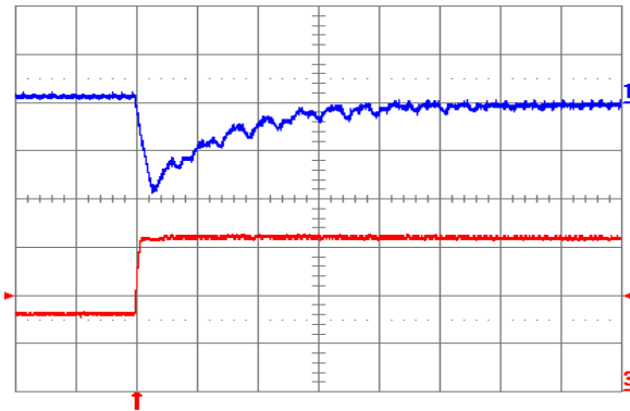
Fig. 3.3V.7: Output voltage for V_{out} = 3.3 V to positive load current step change from 8 A to 16 A with slew rate of 5 A/ \mu s at V_{in} = 5 V. Top trace: output voltage (100 mV/div.); Bottom trace: load current (5 A/div.). C_o = 100 \mu F ceramic. Time scale: 20 \mu s/div.
