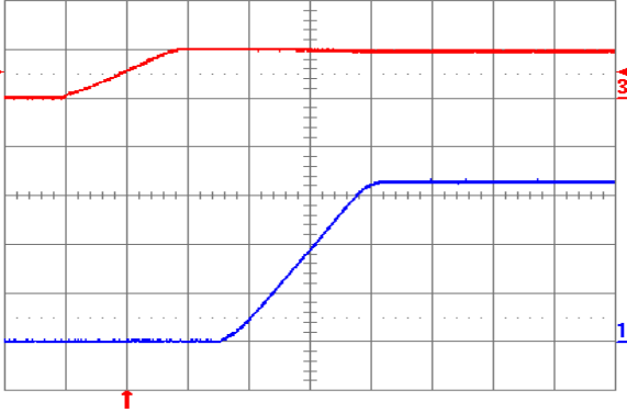
Fig. 3.3V.5: Turn-on transient for V_{out} = 3.3 V with application of V_{in} at full rated load current (resistive) and 100 \mu F external capacitance at V_{in} = 5 V. Top trace: V_{in} (5 V/div.); Bottom trace: output voltage (1 V/div.); Time scale: 2 ms/div.
