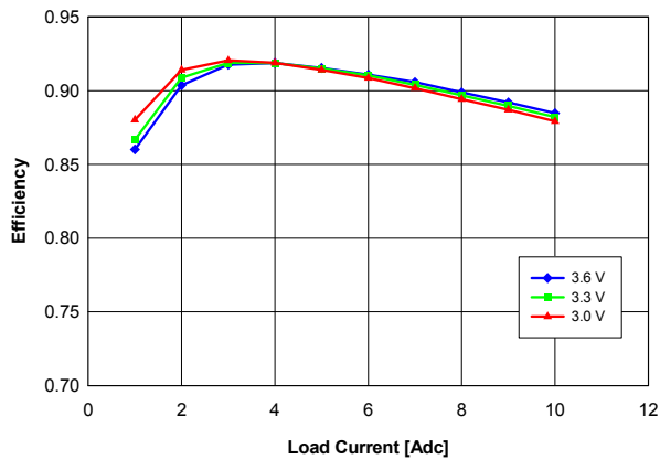
Fig. 1.2V.4: Efficiency vs. load current and input voltage for V_{out} = 1.2 V converter mounted vertically with air flowing at a rate of 200 LFM (1 m/s) and T_a = 25 °C.
