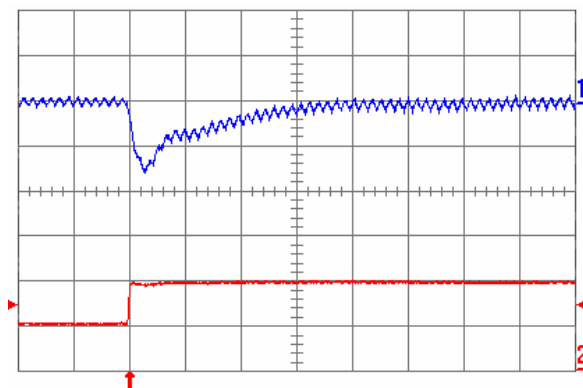
Fig. 1.8V.7: Output voltage response for V_{out} = 1.8 V to positive load current step change from 5 A to 10 A with slew rate of 5 A/ \mu s at V_{in} = 5 V. Top trace: output voltage (100 mV/div.); Bottom trace: load current (5 A/div.). C_o = 100 \mu F ceramic + 1 \mu F ceramic. Time scale: 20 \mu s/div.
