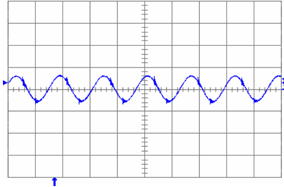
Fig. 1.2V.6: Output voltage ripple (20 mV/div.) at full rated load current into a resistive load with external capacitance 100 \mu F ceramic + 1 \mu F ceramic and V_{in} = 5 V for V_{out} = 1.2 V. Time scale: 2 \mu s/div.
