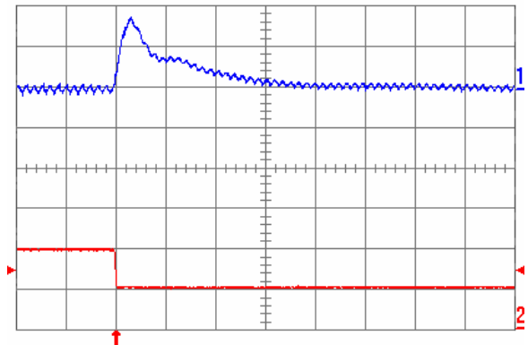
Fig. 1.5V.8: Output voltage response for V_{out} = 1.5 V to negative load current step change from 10 A to 5 A with slew rate of -5 A/ \mu s at V_{in} = 5 V. Top trace: output voltage (100 mV/div.); Bottom trace: load current (5 A/div.). C_o = 100 \mu F ceramic + 1 \mu F ceramic. Time scale: 20 \mu s/div.
