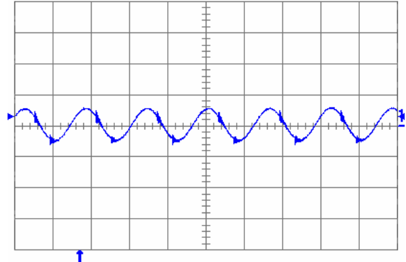
Fig. 1.0V.6: Output voltage ripple (20 mV/div.) at full rated load current into a resistive load with external capacitance 100 \mu\text{F} ceramic + 1 \mu\text{F} ceramic and V_{in} = 5 V for V_{out} = 1.0 V. Time scale: 2 \mu\text{s} /div.
