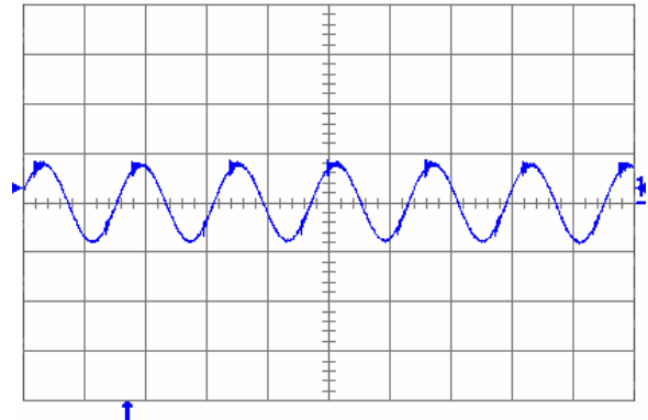
Fig. 3.3V.6: Output voltage ripple (20 mV/div.) at full rated load current into a resistive load with external capacitance 100 \mu F ceramic + 1 \mu F ceramic and V_{in} = 5 V for V_{out} = 3.3 V. Time scale: 2 \mu s/div.
