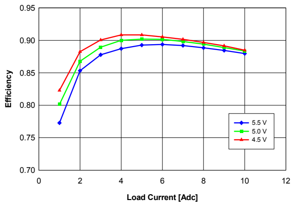
Fig. 1.2V.3: Efficiency vs. load current and input voltage for V_{out} = 1.2\text{ V} converter mounted vertically with air flowing at a
