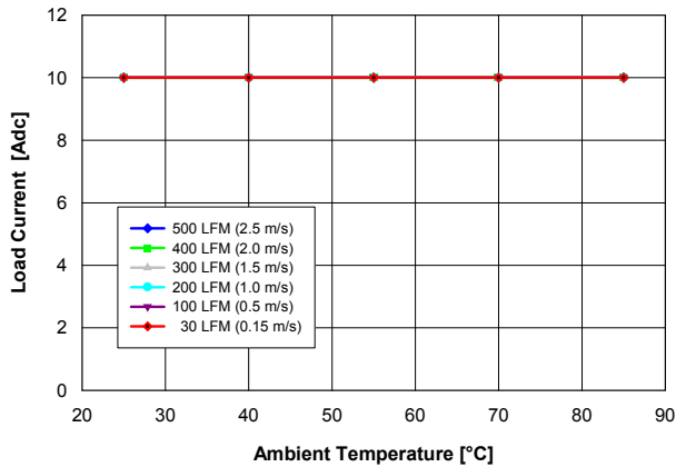
Fig. 3.3V.1: Available load current vs. ambient temperature and airflow rates for V_{out} = 3.3 V converter mounted vertically with V_{in} = 5 V, and maximum MOSFET temperature \leq 120 °C.
