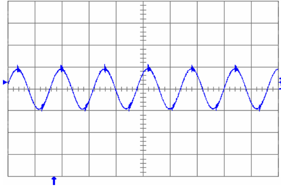
Fig. 2.5V.6: Output voltage ripple (20 mV/div.) at full rated load current into a resistive load with external capacitance 100 \mu F ceramic + 1 \mu F ceramic and V_{in} = 5 V for V_{out} = 2.5 V. Time scale: 2 \mu s/div.
