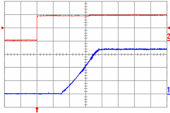
Fig. 0.7525V.5: Turn-on transient for V_{out} = 0.7525 V with the application of Enable signal at full rated load current (resistive) and 100 \mu F external capacitance at V_{in} = 5 V. Top trace: Enable signal (2 V/div.); Bottom trace: output voltage (200 mV/div.); Time scale: 2 ms/div.
