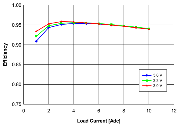
Fig. 2.5V.4: Efficiency vs. load current and input voltage for V_{out} = 2.5 V converter mounted vertically with air flowing at a rate of 200 LFM (1 m/s) and T_a = 25 °C.
