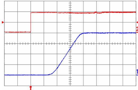
Fig. 2.0V.5: Turn-on transient for V_{out} = 2.0 V with the application of Enable signal at full rated load current (resistive) and 100\ \mu\text{F} external capacitance at V_{in} = 5 V. Top trace: Enable signal (2 V/div.); Bottom trace: output voltage (500 mV/div.); Time scale: 2 ms/div.
