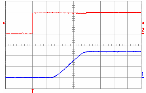
Fig. 1.2V.5: Turn-on transient for V_{out} = 1.2 V with the application of Enable signal at full rated load current (resistive) and 100 \mu F external capacitance at V_{in} = 5 V. Top trace: Enable signal (2 V/div.); Bottom trace: output voltage (500 mV/div.); Time scale: 2 ms/div.
