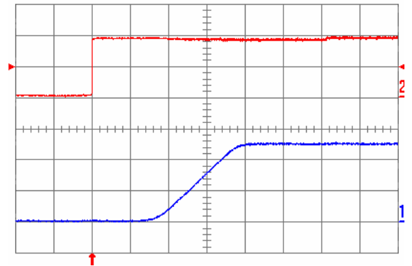
Fig. 2.5V.5: Turn-on transient for V_{out} = 2.5 V with the application of Enable signal at full rated load current (resistive) and 100 \mu F external capacitance at V_{in} = 5 V. Top trace: Enable signal (2 V/div.); Bottom trace: output voltage (1 V/div.); Time scale: 2 ms/div.
