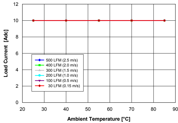
Fig. 1.2V.2: Available load current vs. ambient temperature and airflow rates for V_{out} = 1.2 V converter mounted horizontally with V_{in} = 5 V, and maximum MOSFET temperature \leq 120 °C.
