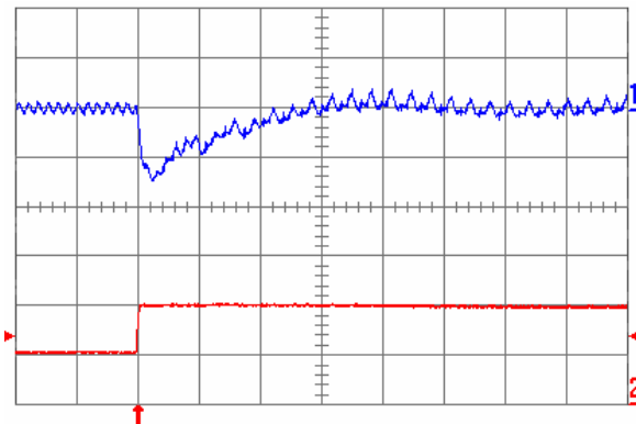
Fig. 3.3V.7: Output voltage for V_{out} = 3.3 V to positive load current step change from 5 A to 10 A with slew rate of 5 A/ \mu s at V_{in} = 5 V. Top trace: output voltage (100 mV/div.); Bottom trace: load current (5 A/div.). C_o = 100 \mu F ceramic + 1 \mu F ceramic. Time scale: 20 \mu s/div.
