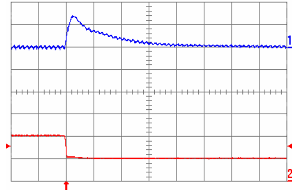
Fig. 0.7525V.8: Output voltage response for V_{out} = 0.7525 V to negative load current step change from 10 A to 8 A with slew rate of -5 A/ \mu s at V_{in} = 5 V. Top trace: output voltage (100 mV/div.); Bottom trace: load current (5 A/div.). C_o = 100 \mu F ceramic + 1 \mu F ceramic. Time scale: 20 \mu s/div.
