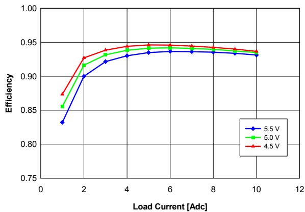
Fig. 2.5V.3: Efficiency vs. load current and input voltage for V_{out} = 2.5\text{ V} converter mounted vertically with air flowing at a rate of 200 LFM (1 m/s) and T_a = 25^\circ\text{C} .
