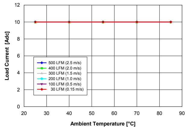
Fig. 2.0V.1: Available load current vs. ambient temperature and airflow rates for V_{out} = 2.0 V converter mounted vertically with V_{in} = 5 V, and maximum MOSFET temperature \leq 120 °C.
