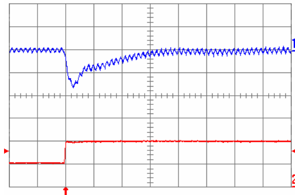
Fig. 2.0V.7: Output voltage response for V_{out} = 2.0 V to positive load current step change from 5 A to 10 A with slew rate of 5 A/ \mu\text{s} at V_{in} = 5 V. Top trace: output voltage (100 mV/div.); Bottom trace: load current (5 A/div.). C_o = 100\ \mu\text{F} ceramic + 1\ \mu\text{F} ceramic. Time scale: 20 \mu\text{s} /div.
