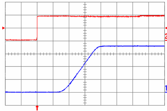
Fig. 1.8V.5: Turn-on transient for V_{out} = 1.8 V with the application of Enable signal at full rated load current (resistive) and 100 \mu F external capacitance at V_{in} = 5 V. Top trace: Enable signal (2 V/div.); Bottom trace: output voltage (500 mV/div.); Time scale: 2 ms/div.
