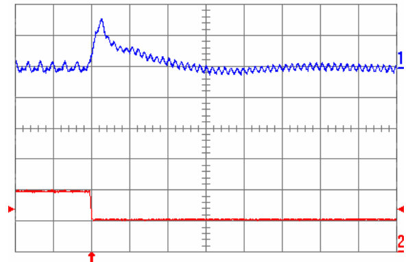
Fig. 3.3V.8: Output voltage response for V_{out} = 3.3 V to negative load current step change from 10 A to 5 A with slew rate of -5 A/ \mu s at V_{in} = 5 V. Top trace: output voltage (100 mV/div.); Bottom trace: load current (5 A/div.). C_o = 100 \mu F ceramic + 1 \mu F ceramic. Time scale: 20 \mu s/div.
