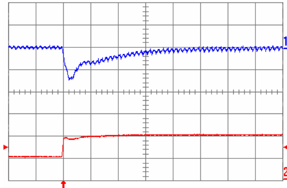
Fig. 1.0V.7: Output voltage response V_{out} = 1.0 V to positive load current step change from 5 A to 10 A with slew rate of 5 \text{ A}/\mu\text{s} at V_{in} = 5 V. Top trace: output voltage (100 mV/div.); Bottom trace: load current (5 A/div.). C_o = 100 \mu\text{F} ceramic + 1 \mu\text{F} ceramic. Time scale: 20 \mu\text{s} /div.
