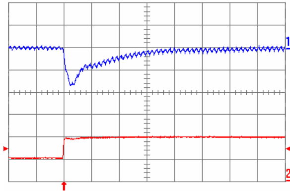
Fig. 1.5V.7: Output voltage response for V_{out} = 1.5 V to positive load current step change from 5 A to 10 A with slew rate of 5 A/ \mu s at V_{in} = 5 V. Top trace: output voltage (100 mV/div.); Bottom trace: load current (5 A/div.). C_o = 100 \mu F ceramic + 1 \mu F ceramic. Time scale: 20 \mu s/div.
