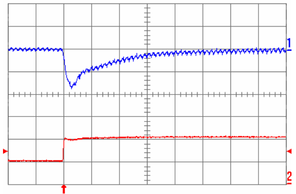
Fig. 1.2V.6: Output voltage response for V_{out} = 1.2 V to positive load current step change from 5 A to 10 A with slew rate of 5 A/ \mu s at V_{in} = 5 V. Top trace: output voltage (100 mV/div.); Bottom trace: load current (5 A/div.). C_o = 100 \mu F ceramic + 1 \mu F ceramic. Time scale: 20 \mu s/div.
