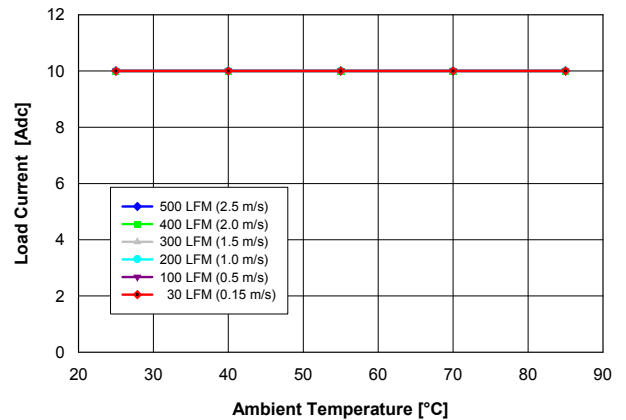
Fig. 3.3V.2: Available load current vs. ambient temperature and airflow rates for V_{out} = 3.3 V converter mounted horizontally with V_{in} = 5 V, and maximum MOSFET temperature \leq 120 °C.
