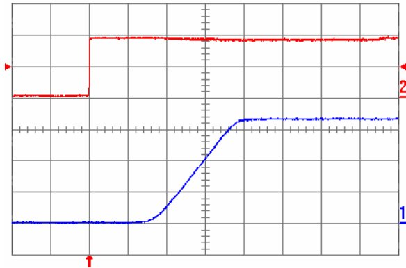
Fig. 3.3V.5: Turn-on transient for V_{out} = 3.3 V with the application of Enable signal at full rated load current (resistive) and 100 \mu F external capacitance at V_{in} = 5 V. Top trace: Enable signal (2 V/div.); Bottom trace: output voltage (1 V/div.); Time scale: 2 ms/div.
