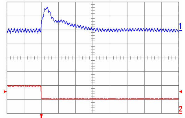
Fig. 2.0V.8: Output voltage response for V_{out} = 2.0 V to negative load current step change from 10 A to 5 A with slew rate of -5 A/ \mu\text{s} at V_{in} = 5 V. Top trace: output voltage (100 mV/div.); Bottom trace: load current (5 A/div.). C_o = 100\ \mu\text{F} ceramic + 1\ \mu\text{F} ceramic. Time scale: 20 \mu\text{s} /div.
