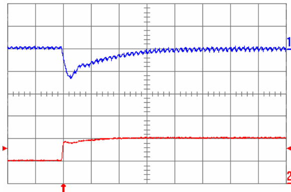
Fig. 0.7525V.7: Output voltage response for V_{out} = 0.7525 V to positive load current step change from 5 A to 10 A with slew rate of 5 A/ \mu s at V_{in} = 5 V. Top trace: output voltage (100 mV/div.); Bottom trace: load current (5 A/div.). C_o =
