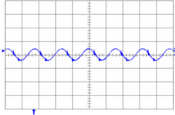
Fig. 0.7525V.6: Output voltage ripple (20 mV/div.) at full rated load current into a resistive load with external capacitance 100 \mu F ceramic + 1 \mu F ceramic and V_{in} = 5 V for V_{out} = 0.7525 V. Time scale: 2 \mu s/div.
