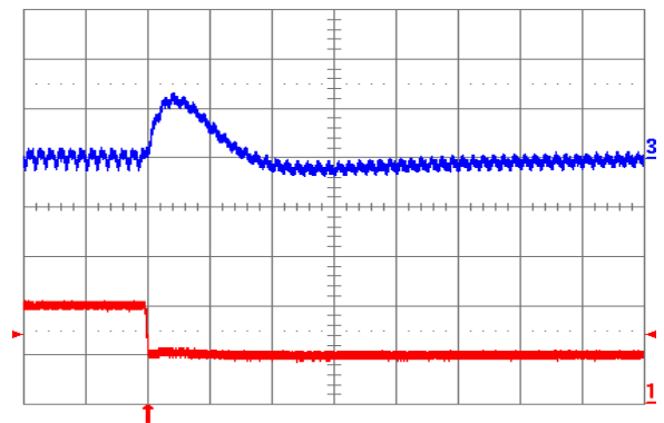
Fig. 2.5V.8: Output voltage response (YNL12S10025) to negative load current step change from 10 A to 5 A with slew rate of -5 A/ \mu s at V_{in} = 12 V. Top trace: output voltage (100 mV/div.); Bottom trace: load current (5 A/div.). C_o = 100 \mu F ceramic. Time scale: 20 \mu s/div.
