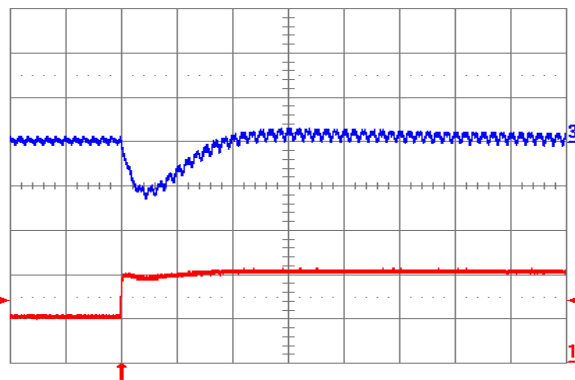
Fig. 1.8V.7: Output voltage response (YNL12S10018) to positive load current step change from 5 A to 10 A with slew rate of 5 A/ \mu s at V_{in} = 12 V. Top trace: output voltage (100 mV/div.); Bottom trace: load current (5 A/div.). C_o = 100 \mu F ceramic. Time scale: 20 \mu s/div.
