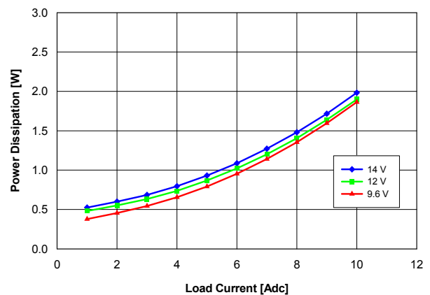
Fig. 1.8V.4: Power loss vs. load current and input voltage for YNL12S10018 converter mounted vertically with air flowing at a rate of 200 LFM (1 m/s) and T_a = 25\text{ }^{\circ}\text{C} .
