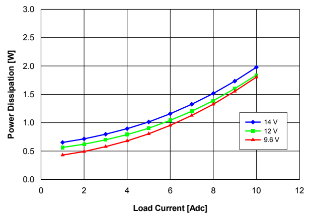
Fig. 2.5V.4: Power loss vs. load current and input voltage for YNL12S10025 converter mounted vertically with air flowing at a rate of 200 LFM (1 m/s) and T_a = 25 °C.
