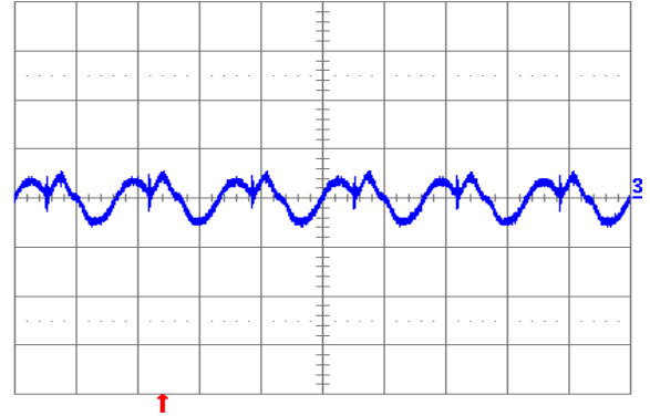
Fig. 1.5V.6: Output voltage ripple (20 mV/div.) at full rated load current into a resistive load with external capacitance 100 \mu F ceramic + 1 \mu F ceramic and V_{in} = 12 V (YNL12S10015). Time scale: 2 \mu s/div.
