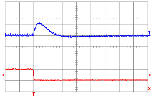
Fig. 1.0V.8: Output voltage response (YNL12S10010) to negative load current step change from 10 A to 5 A with slew rate of -5 A/ \mu\text{s} at V_{in} = 12\text{ V} . Top trace: output voltage (100 mV/div.); Bottom trace: load current (5 A/div.). C_o = 100\text{ }\mu\text{F} ceramic. Time scale: 20 \mu\text{s} /div.
