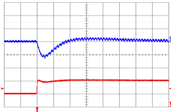
Fig. 1.2V.7: Output voltage response (YNL12S10012) to positive load current step change from 5 A to 10 A with slew rate of 5 A/ \mu\text{s} at V_{in} = 12\text{ V} . Top trace: output voltage (100 mV/div.); Bottom trace: load current (5 A/div.). C_o = 100\text{ }\mu\text{F} ceramic. Time scale: 20 \mu\text{s} /div.
