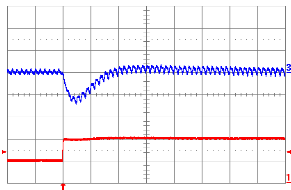
Fig. 3.3V.7: Output voltage response (YNL12S10033) to positive load current step change from 5 A to 10 A with slew rate of 5 A/ \mu\text{s} at V_{in} = 12\text{ V} . Top trace: output voltage (100 mV/div.); Bottom trace: load current (5 A/div.). C_o = 100\text{ }\mu\text{F} ceramic. Time scale: 20 \mu\text{s} /div.
