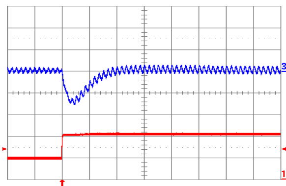
Fig. 5.0V.7: Output voltage response (YNL12S10050) to positive load current step change from 5 A to 10 A with slew rate of 5 A/ \mu s at V_{in} = 12 V. Top trace: output voltage (100 mV/div.); Bottom trace: load current (5 A/div.). C_o = 100 \mu F ceramic. Time scale: 20 \mu s/div.
