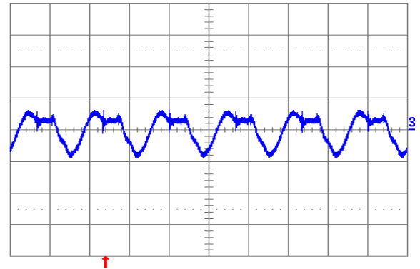
Fig. 2.5V.6: Output voltage ripple (20 mV/div.) at full rated load current into a resistive load with external capacitance 100 \mu F ceramic + 1 \mu F ceramic and V_{in} = 12 V (YNL12S10025). Time scale: 2 \mu s/div.
