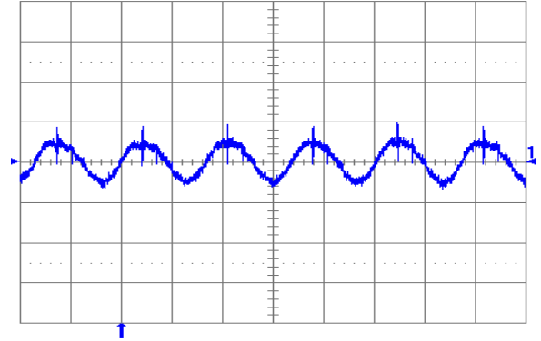
Fig. 2.0V.6: Output voltage ripple (20 mV/div.) at full rated load current into a resistive load with external capacitance 100 \mu F ceramic + 1 \mu F ceramic and V_{in} = 12 V (YNL12S10020). Time scale: 2 \mu s/div.
