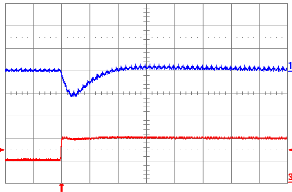
Fig. 1.0V.7: Output voltage response (YNL12S10010) to positive load current step change from 5 A to 10 A with slew rate of 5 A/ \mu\text{s} at V_{in} = 12\text{ V} . Top trace: output voltage (100 mV/div.); Bottom trace: load current (5 A/div.). C_o = 100\text{ }\mu\text{F} ceramic. Time scale: 20 \mu\text{s} /div.
