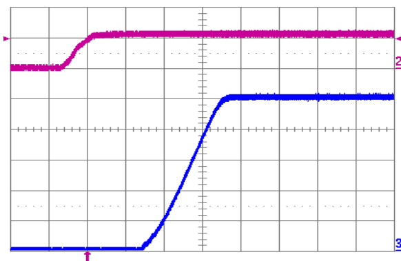
Fig. 5.0V.5: Turn-on transient (YNL12S10050) with application of V_{in} at full rated load current (resistive) and 100 \mu F external capacitance at V_{in} = 12 V. Top trace: V_{in} (10 V/div.); Bottom trace: output voltage (1 V/div.); Time scale: 2 ms/div.
