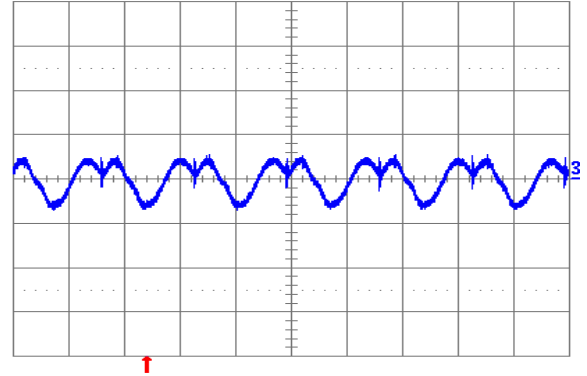
Fig. 1.8V.6: Output voltage ripple (20 mV/div.) at full rated load current into a resistive load with external capacitance 100 \mu F ceramic + 1 \mu F ceramic and V_{in} = 12 V (YNL12S10018). Time scale: 2 \mu s/div.
