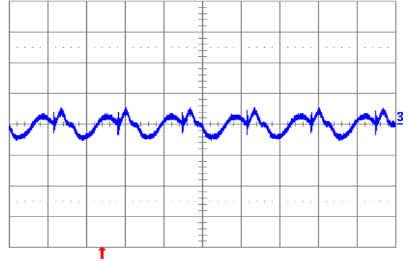
Fig. 1.2V.6: Output voltage ripple (20 mV/div.) at full rated load current into a resistive load with external capacitance 100 \mu\text{F} ceramic + 1 \mu\text{F} ceramic and V_{in} = 12\text{ V} (YNL12S10012). Time scale: 2 \mu\text{s} /div.
