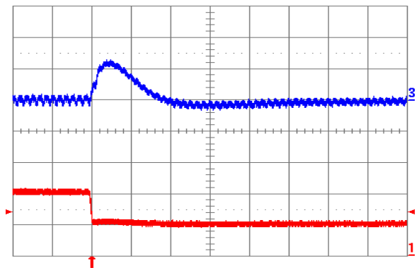
Fig. 1.8V.8: Output voltage response (YNL12S10018) to negative load current step change from 10 A to 5 A with slew rate of -5 A/ \mu s at V_{in} = 12 V. Top trace: output voltage (100 mV/div.); Bottom trace: load current (5 A/div.). C_o = 100 \mu F ceramic. Time scale: 20 \mu s/div.
