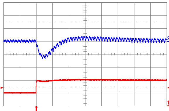
Fig. 2.5V.7: Output voltage response (YNL12S10025) to positive load current step change from 5 A to 10 A with slew rate of 5 A/ \mu s at V_{in} = 12 V. Top trace: output voltage (100 mV/div.); Bottom trace: load current (5 A/div.). C_o = 100 \mu F ceramic. Time scale: 20 \mu s/div.
