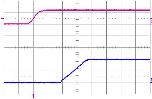
Fig. 2.0V.5: Turn-on transient (YNL12S10020) with application of V_{in} at full rated load current (resistive) and 100 \mu F external capacitance at V_{in} = 12 V. Top trace: V_{in} (10 V/div.); Bottom trace: output voltage (1 V/div.); Time scale: 2 ms/div.
