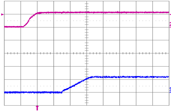
Fig. 1.2V.5: Turn-on transient (YNL12S10012) with application of V_{in} at full rated load current (resistive) and 100 \mu\text{F} external capacitance at V_{in} = 12\text{ V} . Top trace: V_{in} (10 V/div.); Bottom trace: output voltage (1 V/div.); Time scale: 2 ms/div.
