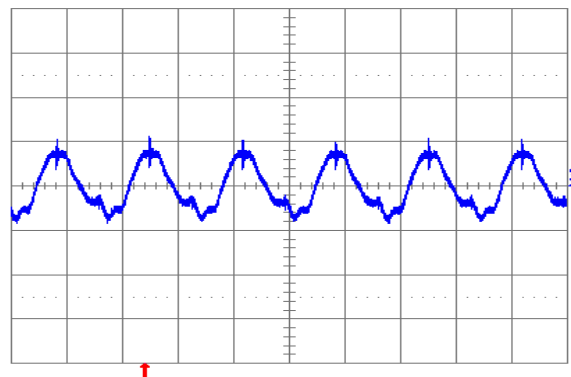
Fig. 5.0V.6: Output voltage ripple (20 mV/div.) at full rated load current into a resistive load with external capacitance 100 \mu F ceramic + 1 \mu F ceramic and V_{in} = 12V (YNL12S10050). Time scale: 2 \mu s/div.
