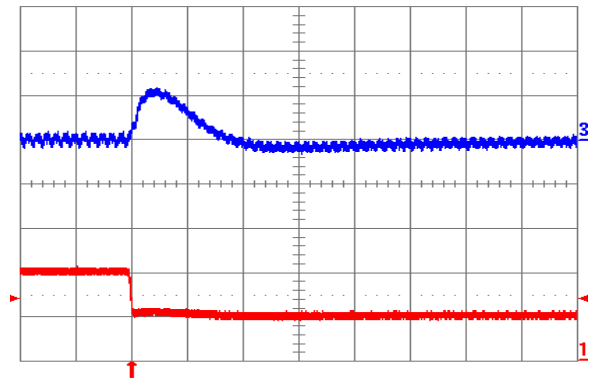
Fig. 1.5V.8: Output voltage response (YNL12S10015) to negative load current step change from 10 A to 5 A with slew rate of -5 A/ \mu s at V_{in} = 12 V. Top trace: output voltage (100 mV/div.); Bottom trace: load current (5 A/div.). C_o = 100 \mu F ceramic. Time scale: 20 \mu s/div.
