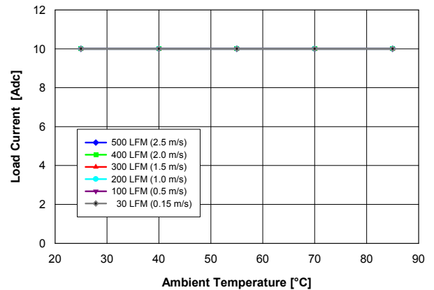
Fig. 2.5V.2: Available load current vs. ambient temperature and airflow rates for YNL12S10025 converter mounted horizontally with V_{in} = 12 V, and maximum MOSFET temperature \leq 110 °C.
