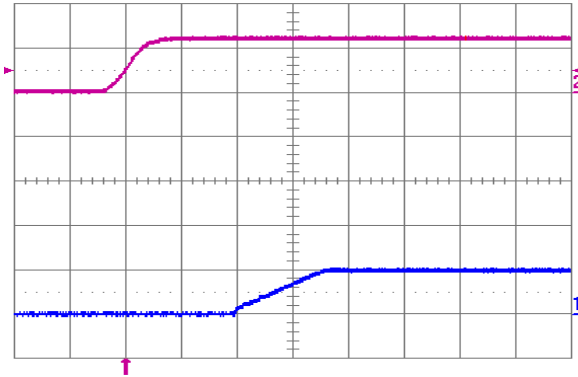
Fig. 1.0V.5: Turn-on transient (YNL12S10010) with application of V_{in} at full rated load current (resistive) and 100 \mu\text{F} external capacitance at V_{in} = 12\text{ V} . Top trace: V_{in} (10 V/div.); Bottom trace: output voltage (1 V/div.); Time scale: 2 ms/div.
