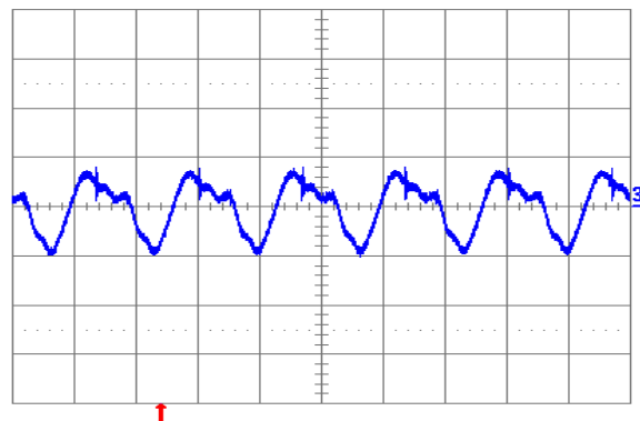
Fig. 3.3V.6: Output voltage ripple (20 mV/div.) at full rated load current into a resistive load with external capacitance 100 \mu\text{F} ceramic + 1 \mu\text{F} ceramic and V_{in} = 12\text{ V} (YNL12S10033). Time scale: 2 \mu\text{s} /div.
