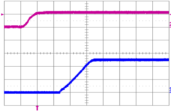
Fig. 2.5V.5: Turn-on transient (YNL12S10025) with application of V_{in} at full rated load current (resistive) and 100 \mu F external capacitance at V_{in} = 12 V. Top trace: V_{in} (10 V/div.); Bottom trace: output voltage (1 V/div.); Time scale: 2 ms/div.
