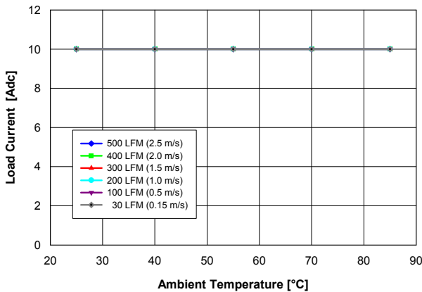
Fig. 2.5V.1: Available load current vs. ambient temperature and airflow rates for YNL12S10025 converter mounted vertically with V_{in} = 12 V, and maximum MOSFET temperature \leq 110 °C.
