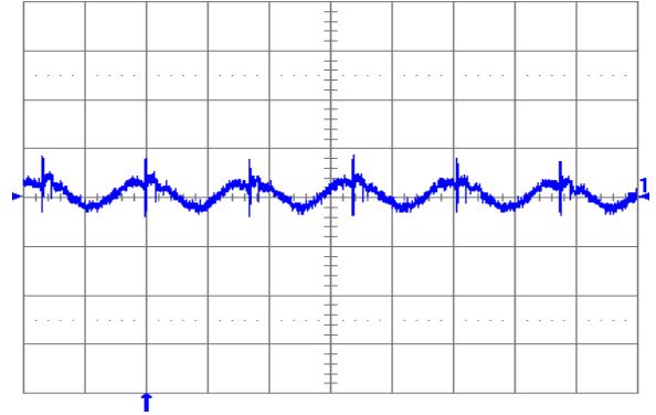
Fig. 1.0V.6: Output voltage ripple (20 mV/div.) at full rated load current into a resistive load with external capacitance 100 \mu\text{F} ceramic + 1 \mu\text{F} ceramic and V_{in} = 12\text{ V} (YNL12S10010). Time scale: 2 \mu\text{s} /div.
