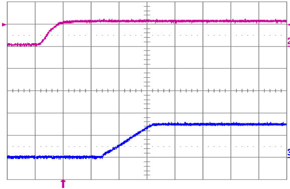
Fig. 1.5V.5: Turn-on transient (YNL12S10015) with application of V_{in} at full rated load current (resistive) and 100 \mu F external capacitance at V_{in} = 12 V. Top trace: V_{in} (10 V/div.); Bottom trace: output voltage (1 V/div.); Time scale: 2 ms/div.
