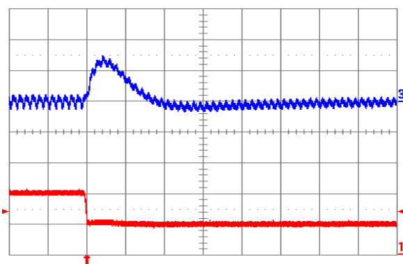
Fig. 3.3V.8: Output voltage response (YNL12S10033) to negative load current step change from 10 A to 5 A with slew rate of -5 A/ \mu\text{s} at V_{in} = 12\text{ V} . Top trace: output voltage (100 mV/div.); Bottom trace: load current (5 A/div.). C_o = 100\text{ }\mu\text{F} ceramic. Time scale: 20 \mu\text{s} /div.
