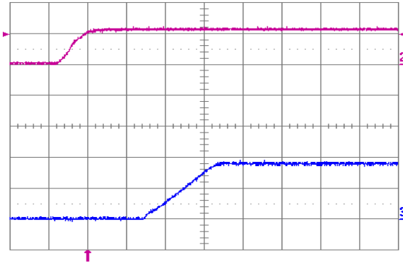
Fig. 1.8V.5: Turn-on transient (YNL12S10018) with application of V_{in} at full rated load current (resistive) and 100 \mu F external capacitance at V_{in} = 12 V. Top trace: V_{in} (10 V/div.); Bottom trace: output voltage (1 V/div.); Time scale: 2 ms/div.
