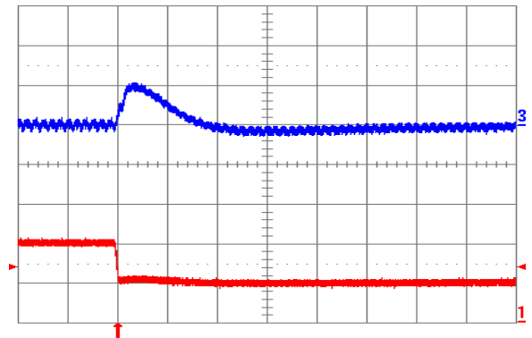
Fig. 1.2V.8: Output voltage response (YNL12S10012) to negative load current step change from 10 A to 5 A with slew rate of -5 A/ \mu\text{s} at V_{in} = 12\text{ V} . Top trace: output voltage (100 mV/div.); Bottom trace: load current (5 A/div.). C_o = 100\text{ }\mu\text{F} ceramic. Time scale: 20 \mu\text{s} /div.
