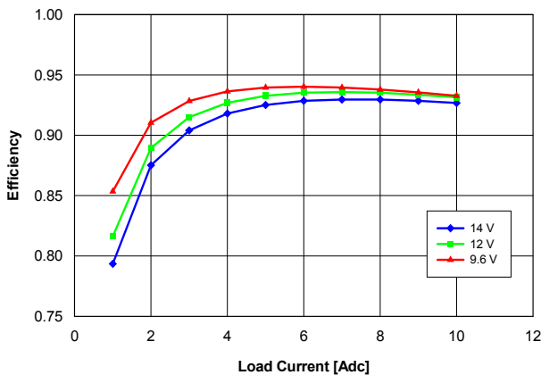
Fig. 2.5V.3: Efficiency vs. load current and input voltage for YNL12S10025 converter mounted vertically with air flowing at a rate of 200 LFM (1 m/s) and T_a = 25 °C.
