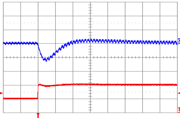
Fig. 1.5V.7: Output voltage response (YNL12S10015) to positive load current step change from 5 A to 10 A with slew rate of 5 A/ \mu s at V_{in} = 12 V. Top trace: output voltage (100 mV/div.); Bottom trace: load current (5 A/div.). C_o = 100 \mu F ceramic. Time scale: 20 \mu s/div.
