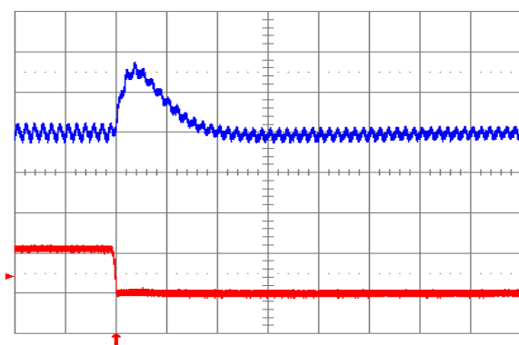
Fig. 5.0V.8: Output voltage response (YNL12S10050) to negative load current step change from 10 A to 5 A with slew rate of -5 A/ \mu s at V_{in} = 12 V. Top trace: output voltage (100 mV/div.); Bottom trace: load current (5 A/div.). C_o = 100 \mu F ceramic. Time scale: 20 \mu s/div.
