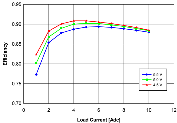
Fig. 1.2V.3: Efficiency vs. load current and input voltage for YNL05S10012 converter mounted vertically with air flowing at a rate of 200 LFM (1 m/s) and T_a = 25 °C.
