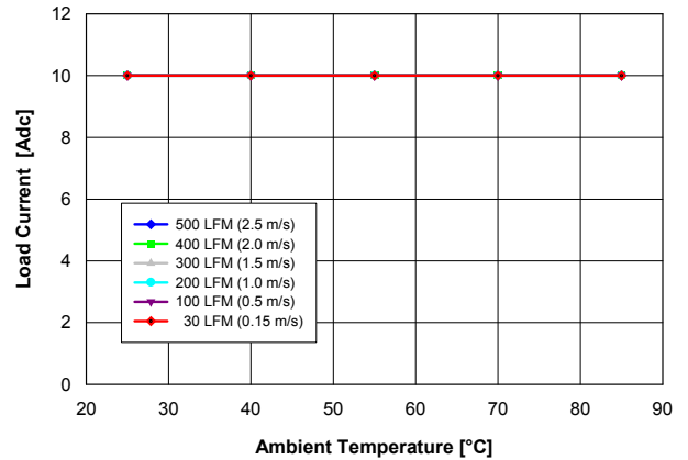
Fig. 1.2V.2: Available load current vs. ambient temperature and airflow rates for YNL05S10012 converter mounted horizontally with V_{in} = 5 V, and maximum MOSFET temperature \leq 110 °C.
