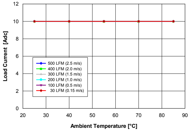
Fig. 1.2V.1: Available load current vs. ambient temperature and airflow rates YNL05S10012 converter mounted vertically with V_{in} = 5 V, and maximum MOSFET temperature \leq 110 °C.
