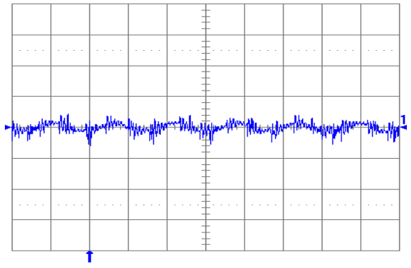
Fig. 1.5V.6: Output voltage ripple (20 mV/div.) at full rated load current into a resistive load with external capacitance 47 \mu F ceramic + 1 \mu F ceramic and V_{in} = 5 V (YNL05S10015). Time scale: 2 \mu s/div.
