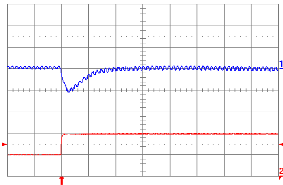
Fig. 2.5V.7: Output voltage response (YNL05S10025) to positive load current step change from 5 A to 10 A with slew rate of 5 A/ \mu s at V_{in} = 5 V. Top trace: output voltage (100 mV/div.); Bottom trace: load current (5 A/div.). C_o = 47 \mu F ceramic + 1 \mu F ceramic. Time scale: 20 \mu s/div.
