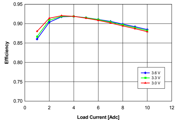
Fig. 1.2V.4: Efficiency vs. load current and input voltage for YNL05S10012 converter mounted vertically with air flowing at a rate of 200 LFM (1 m/s) and T_a = 25 °C.
