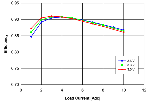
Fig. 1.0V.4: Efficiency vs. load current and input voltage for YNL05S10010 converter mounted vertically with air flowing at a rate of 200 LFM (1 m/s) and T_a = 25 °C.
