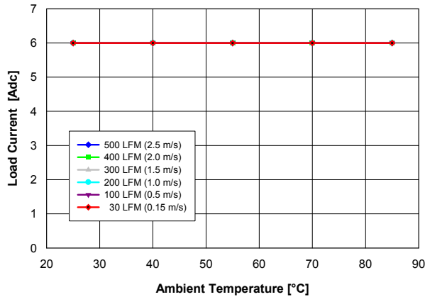
Fig. 3.3V.1: Available load current vs. ambient temperature and airflow rates for V_{out} = 3.3 V converter mounted vertically with V_{in} = 5 V, air flowing from pin 5 to pin 1, and maximum MOSFET temperature \leq 120 °C.
