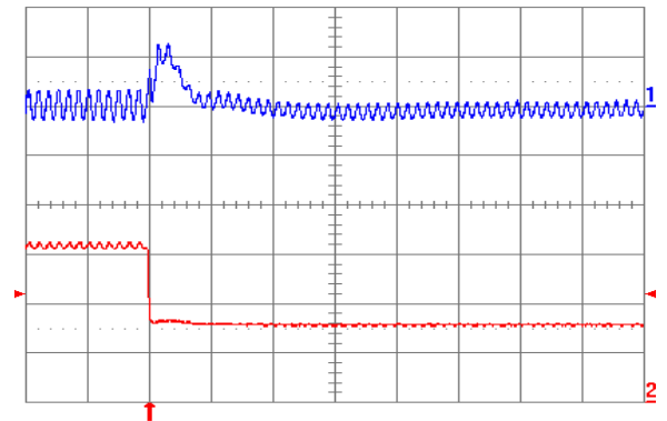
Fig. 2.0V.8: Output voltage response for V_{out} = 2.0 V to negative load current step change from 6 A to 3 A with slew rate of -5 A/ \mu s at V_{in} = 5 V. Top trace: output voltage (100 mV/div.); Bottom trace: load current (2 A/div.). C_o = 47 \mu F ceramic + 1 \mu F ceramic. Time scale: 20 \mu s/div.
