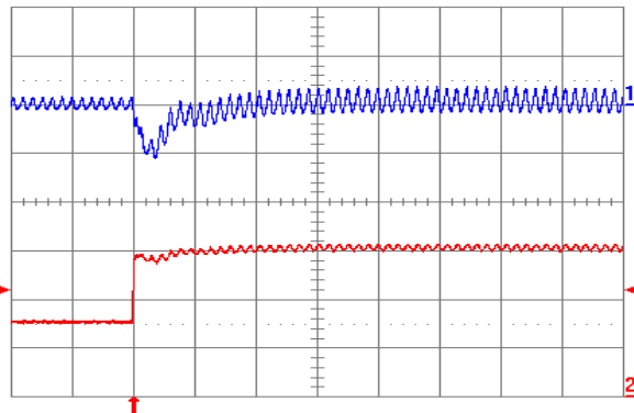
Fig. 1.2V.7: Output voltage response for V_{out} = 1.2 V to positive load current step change from 3 A to 6 A with slew rate of 5 A/ \mu s at V_{in} = 5 V. Top trace: output voltage (100 mV/div.); Bottom trace: load current (2 A/div.). C_o = 47 \mu F ceramic + 1 \mu F ceramic. Time scale: 20 \mu s/div.
