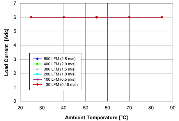
Fig. 1.5V.2: Available load current vs. ambient temperature and airflow rates for V_{out} = 1.5 V converter mounted horizontally with V_{in} = 5 V, air flowing from pin 5 to pin 1, and maximum MOSFET temperature \leq 120 °C.
