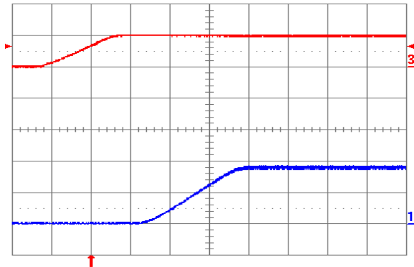
Fig. 1.8V.5: Turn-on transient for V_{out} = 1.8 V with application of V_{in} at full rated load current (resistive) and 47 \mu F external capacitance at V_{in} = 5 V. Top trace: V_{in} (5 V/div.); Bottom trace: output voltage (1 V/div.); Time scale: 2 ms/div.
