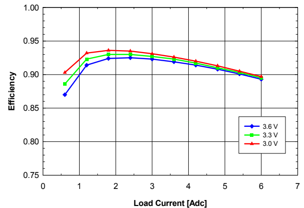
Fig. 1.8V.4: Efficiency vs. load current and input voltage for Vout = 1.8 V converter mounted vertically with air flowing from pin 5 to pin 1 at a rate of 200 LFM (1 m/s) and Ta = 25 °C.
