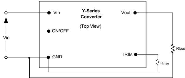
Fig. D: Configuration for programming output voltage.
