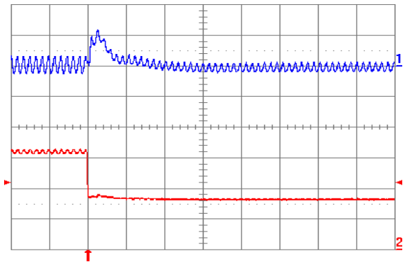
Fig. 1.5V.8: Output voltage response for V_{out} = 1.5 V to negative load current step change from 6 A to 3 A with slew rate of -5 A/ \mu s at V_{in} = 5 V. Top trace: output voltage (100 mV/div.); Bottom trace: load current (2 A/div.). C_o = 47 \mu F ceramic + 1 \mu F ceramic. Time scale: 20 \mu s/div.
