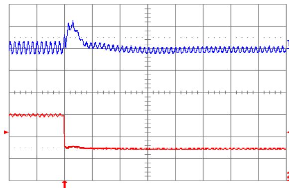
Fig. 1.8V.8: Output voltage response for V_{out} = 1.8 V to negative load current step change from 6 A to 3 A with slew rate of -5 A/ \mu s at V_{in} = 5 V. Top trace: output voltage (100 mV/div.); Bottom trace: load current (2 A/div.). C_o = 47 \mu F ceramic + 1 \mu F ceramic. Time scale: 20 \mu s/div.
