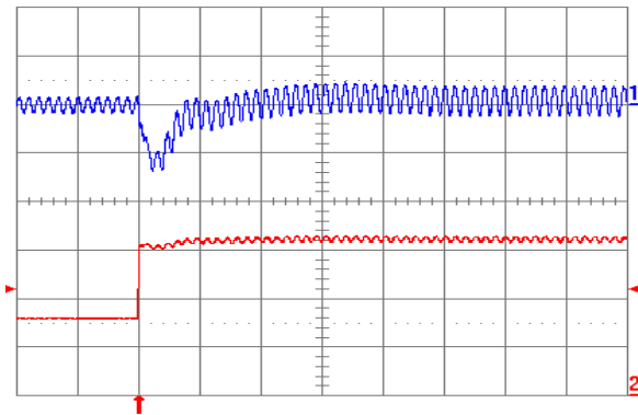
Fig. 2.5V.7: Output voltage response for V_{out} = 2.5 V to positive load current step change from 3 A to 6 A with slew rate of 5 A/ \mu s at V_{in} = 5 V. Top trace: output voltage (100 mV/div.); Bottom trace: load current (2 A/div.). C_o = 47 \mu F ceramic + 1 \mu F ceramic. Time scale: 20 \mu s/div.
