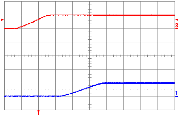
Fig. 1.0V.5: Turn-on transient for V_{out} = 1.0 V with application of V_{in} at full rated load current (resistive) and 47 \mu F external capacitance at V_{in} = 5 V. Top trace: V_{in} (5 V/div.); Bottom trace: output voltage (1 V/div.); Time scale: 2 ms/div.
