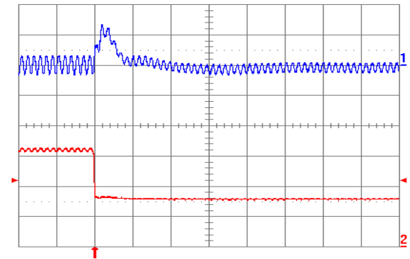
Fig. 2.5V.8: Output voltage response for V_{out} = 2.5 V to negative load current step change from 6 A to 3 A with slew rate of -5 A/ \mu s at V_{in} = 5 V. Top trace: output voltage (100 mV/div.); Bottom trace: load current (2 A/div.). C_o = 47 \mu F ceramic + 1 \mu F ceramic. Time scale: 20 \mu s/div.
