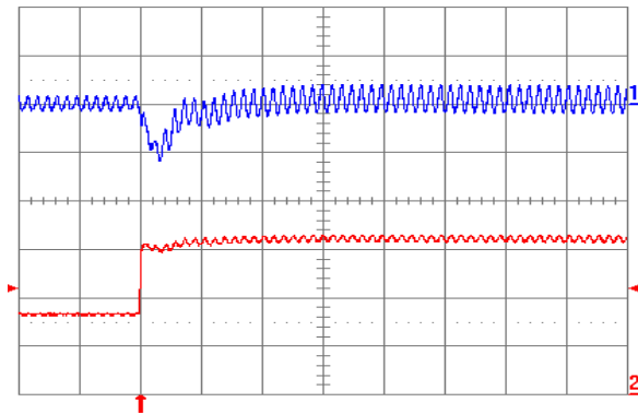
Fig. 1.5V.7: Output voltage response for V_{out} = 1.5 V to positive load current step change from 3 A to 6 A with slew rate of 5 A/ \mu s at V_{in} = 5 V. Top trace: output voltage (100 mV/div.); Bottom trace: load current (2 A/div.). C_o = 47 \mu F ceramic + 1 \mu F ceramic. Time scale: 20 \mu s/div.
