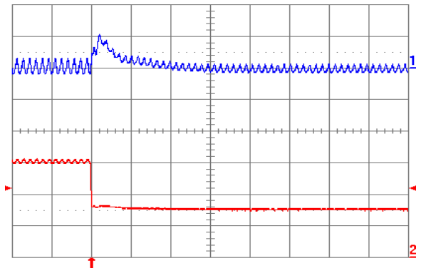
Fig. 1.2V.8: Output voltage response for V_{out} = 1.2 V to negative load current step change from 6 A to 3 A with slew rate of -5 A/ \mu s at V_{in} = 5 V. Top trace: output voltage (100 mV/div.); Bottom trace: load current (2 A/div.). C_o = 47 \mu F ceramic + 1 \mu F ceramic. Time scale: 20 \mu s/div.
