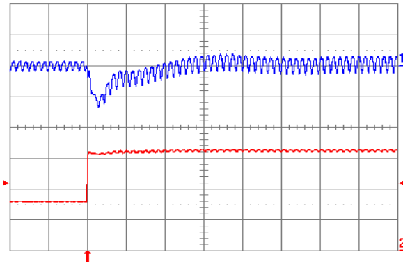
Fig. 3.3V.7: Output voltage response for V_{out} = 3.3 V to positive load current step change from 3 A to 6 A with slew rate of 5 A/ \mu s at V_{in} = 5 V. Top trace: output voltage (100 mV/div.); Bottom trace: load current (2 A/div.). C_o = 47 \mu F ceramic + 1 \mu F ceramic. Time scale: 20 \mu s/div.
