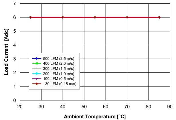
Fig. 3.3V.2: Available load current vs. ambient temperature and airflow rates for V_{out} = 3.3 V converter mounted horizontally with V_{in} = 5 V, air flowing from pin 5 to pin 1, and maximum MOSFET temperature \leq 120 °C.
