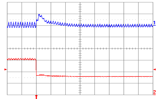
Fig. 1.0V.8: Output voltage response for V_{out} = 1.0 V to negative load current step change from 6 A to 3 A with slew rate of -5 A/ \mu s at V_{in} = 5 V. Top trace: output voltage (100 mV/div.); Bottom trace: load current (2 A/div.). C_o = 47 \mu F ceramic + 1 \mu F ceramic. Time scale: 20 \mu s/div.
