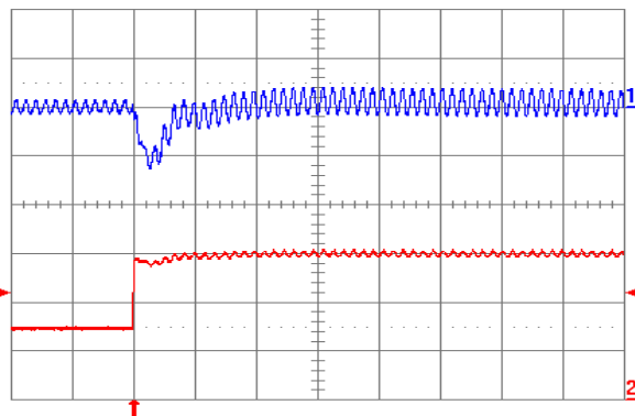
Fig. 1.8V.7: Output voltage response for V_{out} = 1.8 V to positive load current step change from 3 A to 6 A with slew rate of 5 A/ \mu s at V_{in} = 5 V. Top trace: output voltage (100 mV/div.); Bottom trace: load current (2 A/div.). C_o = 47 \mu F ceramic + 1 \mu F ceramic. Time scale: 20 \mu s/div.
