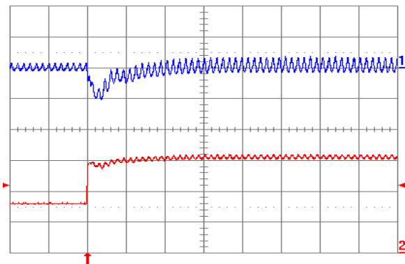
Fig. 1.0V.7: Output voltage response for V_{out} = 1.0 V to positive load current step change from 3 A to 6 A with slew rate of 5 A/ \mu s at V_{in} = 5 V. Top trace: output voltage (100 mV/div.); Bottom trace: load current (2 A/div.). C_o = 47 \mu F ceramic + 1 \mu F ceramic. Time scale: 20 \mu s/div.
