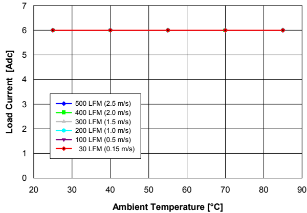
Fig. 1.5V.1: Available load current vs. ambient temperature and airflow rates for V_{out} = 1.5 V converter mounted vertically with V_{in} = 5 V, air flowing from pin 5 to pin 1, and maximum MOSFET temperature \leq 120 °C.
