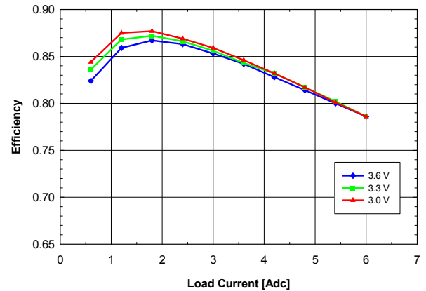
Fig. 0.7525V.4: Efficiency vs. load current and input voltage for V_{out} = 0.7525 V converter mounted horizontally with air flowing from pin 5 to pin 1 at a rate of 200 LFM (1 m/s) and T_a = 25 °C.
