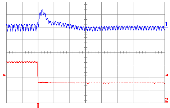
Fig. 3.3V.8: Output voltage response for V_{out} = 3.3 V to negative load current step change from 6 A to 3 A with slew rate of -5 A/ \mu s at V_{in} = 5 V. Top trace: output voltage (100 mV/div.); Bottom trace: load current (2 A/div.). C_o = 47 \mu F ceramic + 1 \mu F ceramic. Time scale: 20 \mu s/div.
