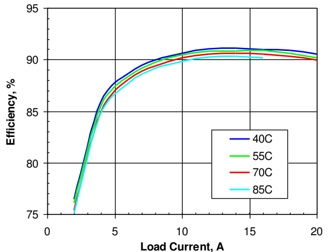
Figure 3. Efficiency vs. load current and ambient temperature for SSQE48T20033 converter mounted vertically with Vin=48V and air flowing from pin 1 to pin 3 at a rate of 200LFM (1.0m/s).
