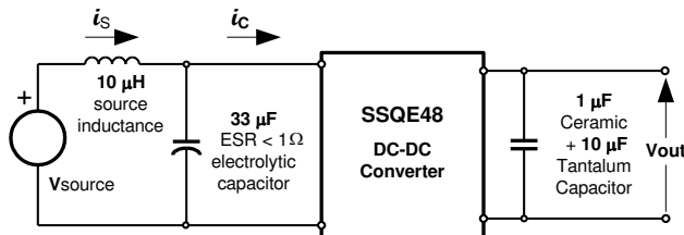
Figure 11. Test setup for measuring input reflected currents, i_c and i_s .
