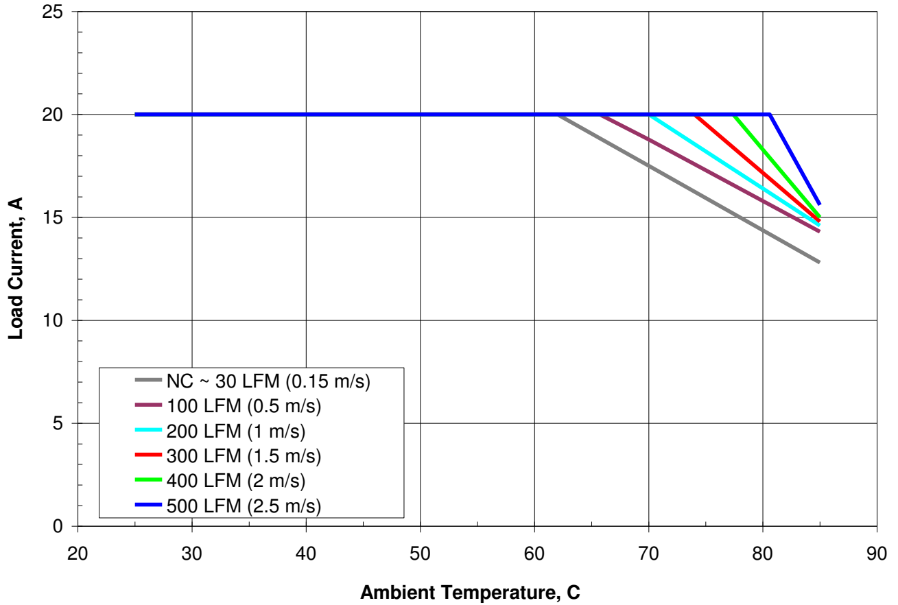
Figure 1. Available load current vs. ambient air temperature and airflow rates for SSQE48T20033 converter mounted vertically with air flowing from pin 1 to pin 3, Vin = 48 V. Note: NC – Natural convection
