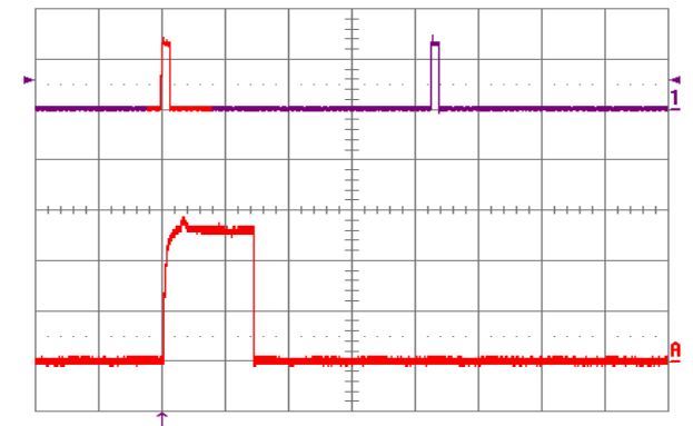
Figure 15. Load current (top trace, 20 A/div., 50 ms/div.) into a 10 \text{ m}\Omega short circuit during restart, at V_{in} = 48 \text{ V} . Bottom trace (10 A/div., 5 ms/div.) is an expansion of the on-time portion of the top trace
