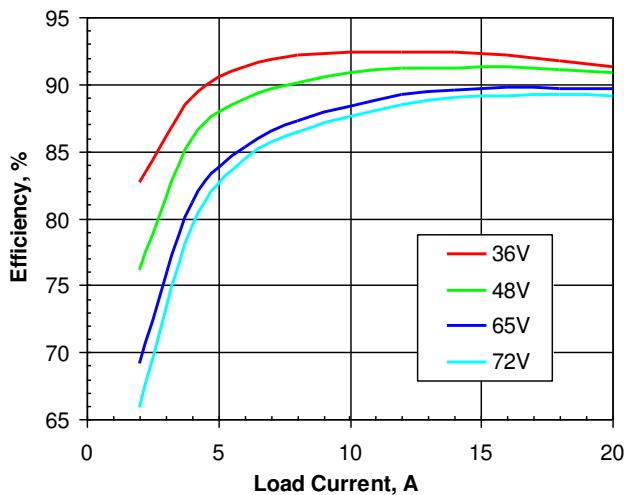
Figure 2. Efficiency vs. load current and input voltage for SSQE48T20033 converter mounted vertically with air flowing from pin 1 to pin 3 at a rate of 300 LFM (1.5 m/s) and Ta=25°C.
