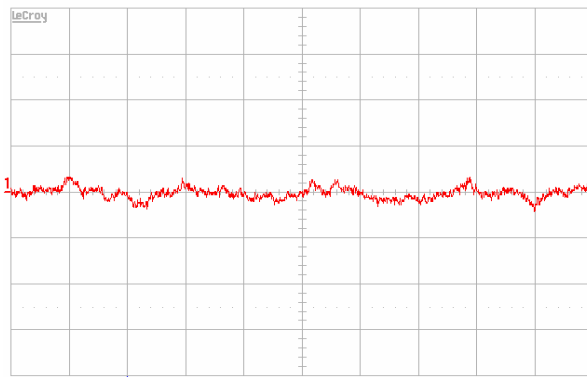
Figure 12. Input reflected-ripple current, i_s (10 mA/div.), measured through 10 \mu\text{H} at the source at full rated load current and V_{in}=48 \text{ V} . Refer to Figure 11 for test setup. Time: 1 \mu\text{s}/\text{div} .
