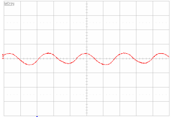
Figure 13. Input reflected ripple-current, i_c (200 mA/div.), measured at input terminals at full rated load current and V_{in}=48 \text{ V} . Refer to Figure 11 for test setup. Time: 1 \mu\text{s}/\text{div} .
