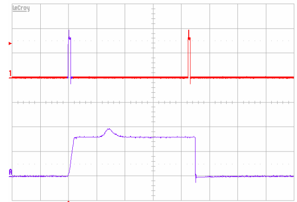
Figure 15. Load current (5 A/div.) into a 10 \text{ m}\Omega short circuit during restart, at V_{in}=48 \text{ V} . Time: 50 \text{ ms}/\text{div} . Bottom trace is an expansion of the on-time portion of the top trace ( 1 \text{ ms}/\text{div} ).
