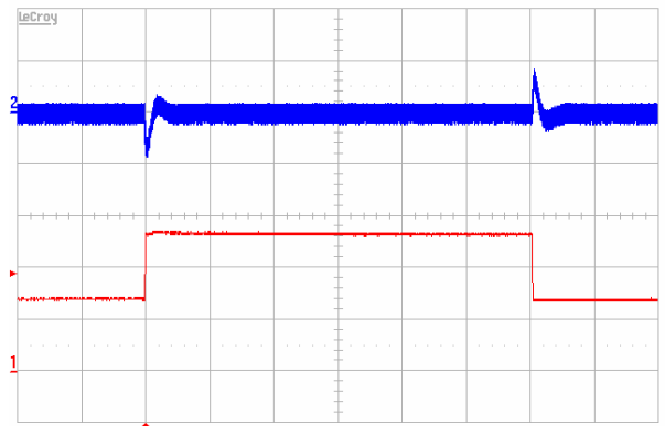
Figure 9. Output voltage response to load current step-change (3.5A–5.25A–3.5A) at V_{in}=48\text{V} . Top trace: Vout (100 mV/div.). Bottom trace: Iout (2 A/div.), Time: (0.2 ms/div.). Current slew rate: 5A/ \mu\text{s} . C_o=470\mu\text{F} POS + 1 \mu\text{F} ceramic..
