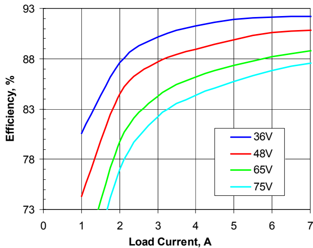
Figure 2. Efficiency vs. load current and input voltage for SSQE48T07050 converter mounted vertically with air flowing from pin 1 to pin 3 at a rate of 300 LFM (1.5 m/s) and T_a = 25^\circ\text{C} .
