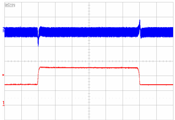
Figure 8. Output voltage response to load current step-change (3.5A–5.25A–3.5A) at V_{in}=48\text{V} . Top trace: Vout (100 mV/div.). Bottom trace: Iout (2 A/div.), Time: (0.2 ms/div.) Current slew rate: 0.1 A/ \mu\text{s} . C_o=1\mu\text{F} ceramic + 10 \mu\text{F} tantalum.
