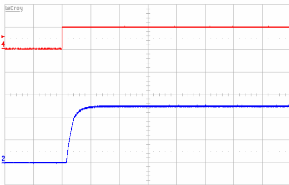
Figure 6. Turn-on transient at full rated load current (resistive) at V_{in} = 48\text{ V} , triggered via ON/OFF pin. Top trace: ON/OFF signal (5 V/div.). Bottom trace: Vout (2V/div), Time: 5 ms/div.
