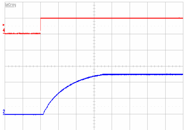
Figure 7. Turn-on transient at full rated load current (resistive) plus 10,000 \mu\text{F} at V_{in} = 48\text{ V} , triggered via ON/OFF pin. Top trace: ON/OFF signal (5V/div) Bottom trace: Vout (2V/div.), Time: 5 ms/div.
