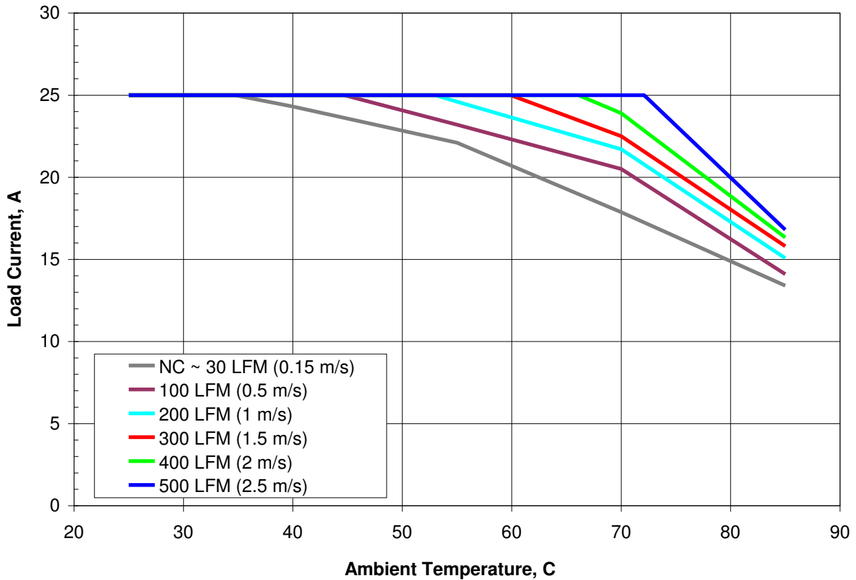
Figure 1. Available load current vs. ambient air temperature and airflow rates for SSQE48T25025 converter mounted vertically with air flowing from pin 1 to pin 3, V_{in} = 48\text{ V} . Note: NC – Natural convection
