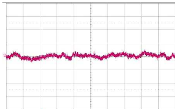
Figure 14. Input reflected-ripple current, i_s (10 mA/div.), measured through 10 μH at the source at full rated load current and V_{in} = 48 V. Refer to Fig. J for test setup. Time scale: 1 μs/div.
