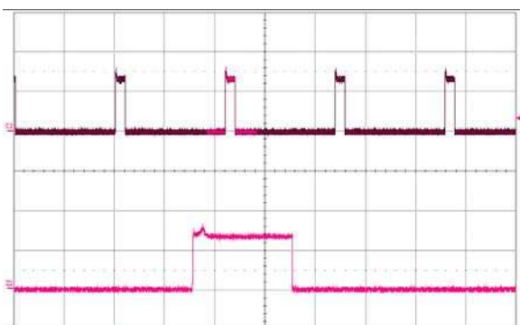
Figure 16. Load current (top trace, 20 A/div., 100 ms/div.) into a 10 mΩ short circuit during restart, at V_{in} = 48 V. Bottom trace (20 A/div., 10 ms/div.) is an expansion of the on-time portion of the top trace.
