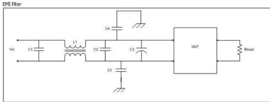
Figure 17. Typical input EMI filter circuit to attenuate conducted emissions.
