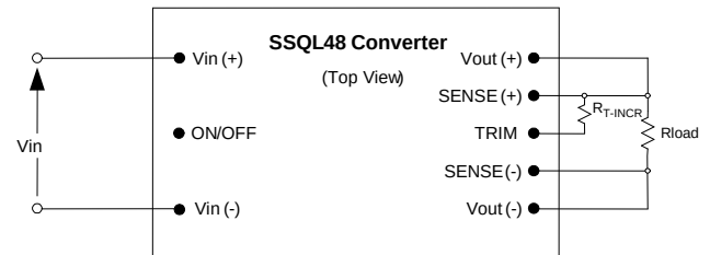
Fig. C: Configuration for increasing output voltage.
