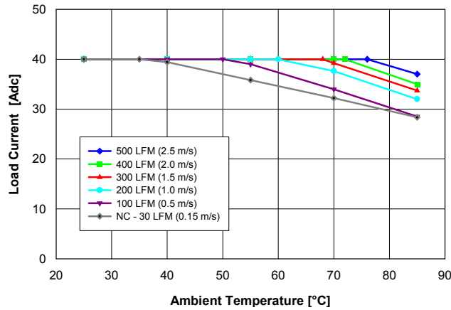
Fig. 1.8V.1: Available load current vs. ambient air temperature and airflow rates for QME48T40018 converter with G height pins mounted vertically with air flowing from pin 1 to pin 3, MOSFET temperature \leq 120 °C, V_{in} = 48 V.
