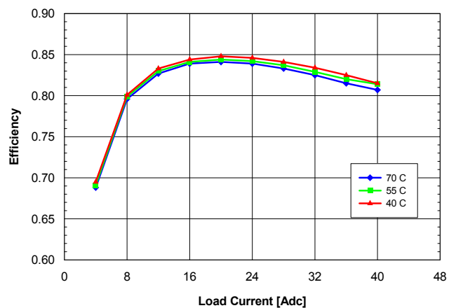
Fig. 1.2V.4: Efficiency vs. load current and ambient temperature for QME48T40012 converter mounted horizontally with V_{in} = 48\text{ V} and air flowing from pin 1 to pin 3 at a rate of 200 LFM (1.0 m/s).
