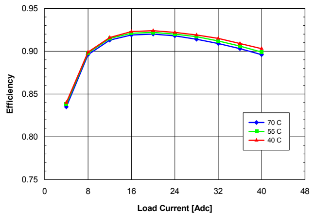
Fig. 3.3V.4: Efficiency vs. load current and ambient temperature for QME48T40033 converter mounted horizontally with V_{in} = 48\text{ V} and air flowing from pin 1 to pin 3 at a rate of 200 LFM (1.0 m/s).
