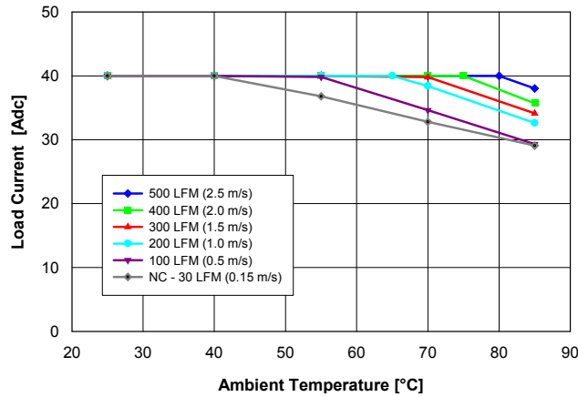
Fig. 1.5V.1: Available load current vs. ambient air temperature and airflow rates for QME48T40015 converter with G height pins mounted vertically with air flowing from pin 1 to pin 3, MOSFET temperature \leq 120 °C, V_{in} = 48 V.
