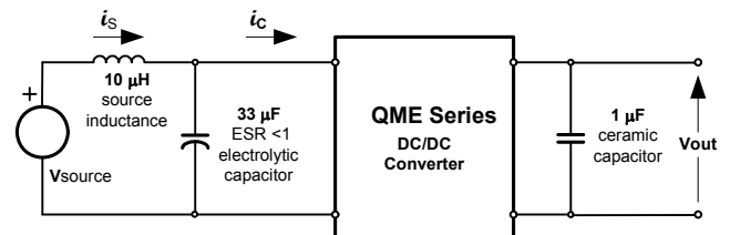
Fig. 3.3V.12: Test setup for measuring input reflected ripple currents, i_c and i_s .
