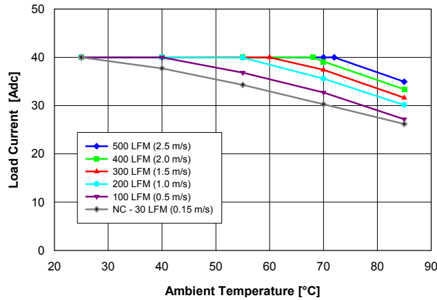
Fig. 2.5V.1: Available load current vs. ambient air temperature and airflow rates for QME48T40025 converter with G height pins mounted vertically with air flowing from pin 1 to pin 3, MOSFET temperature \leq 120\text{ }^{\circ}\text{C} , V_{in} = 48\text{ V} .
