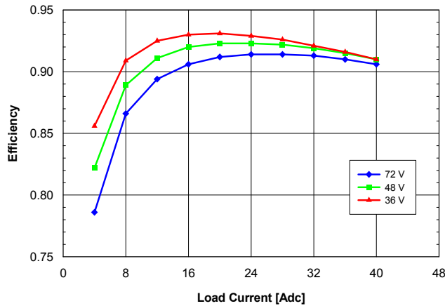
Fig. 3.3V.3: Efficiency vs. load current and input voltage for QME48T40033 converter mounted horizontally with air flowing from pin 1 to pin 3 at a rate of 300 LFM (1.5 m/s) and T_a = 25^{\circ}\text{C} .
