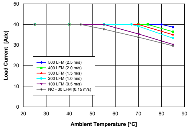
Fig. 1.2V.1: Available load current vs. ambient air temperature and airflow rates for QME48T40012 converter with G height pins mounted vertically with air flowing from pin 1 to pin 3, MOSFET temperature \leq 120\text{ }^{\circ}\text{C} , V_{in} = 48\text{ V} .
