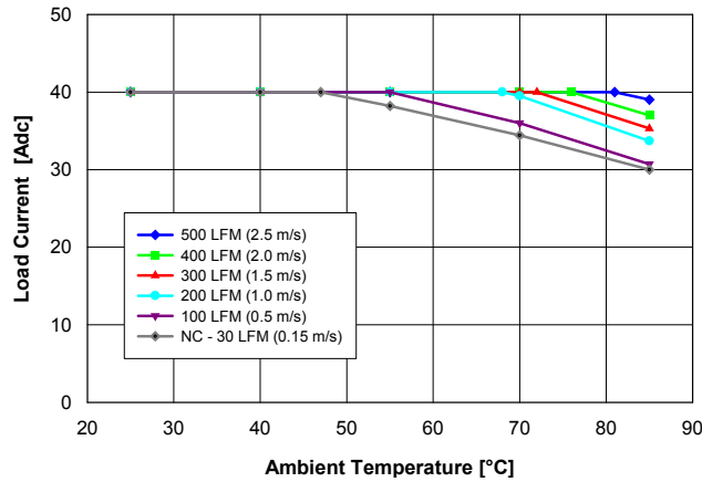
Fig. 1.0V.1: Available load current vs. ambient air temperature and airflow rates for QME48T40010 converter with G height pins mounted vertically with air flowing from pin 1 to pin 3, MOSFET temperature \leq 120 °C, V_{in} = 48 V.
