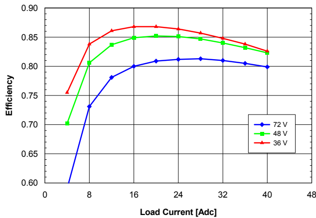
Fig. 1.2V.3: Efficiency vs. load current and input voltage for QME48T40012 converter mounted horizontally with air flowing from pin 1 to pin 3 at a rate of 300 LFM (1.5 m/s) and T_a = 25\text{ }^{\circ}\text{C} .
