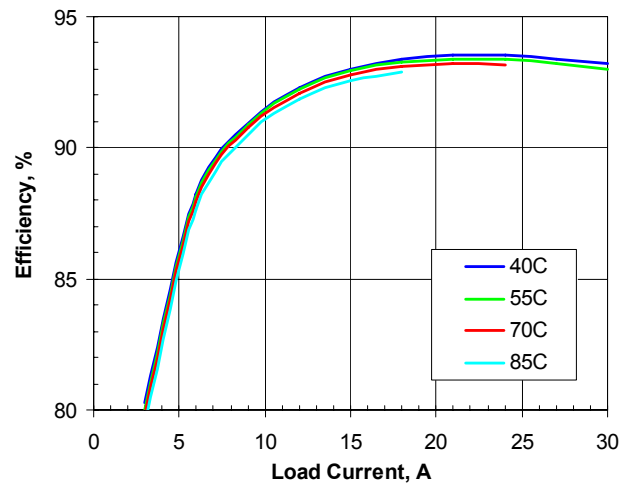
Fig. 3: Efficiency vs. load current and ambient temperature for converter mounted vertically with V_{in} = 48\text{ V} and air flowing from pin 1 to pin 3 at a rate of 200 LFM (1.0 m/s).
