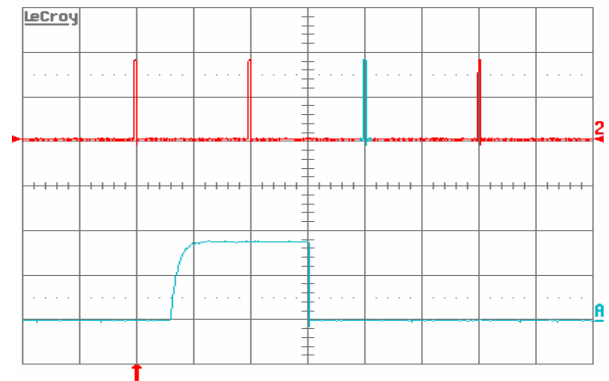
Fig. 15: Load current (top trace, 20 A/div., 100 ms/div.) into a 10 m \Omega short circuit during restart, at V_{in} = 48 V. Bottom trace (20 A/div., 2 ms/div.) is an expansion of the on-time portion of the top trace.
