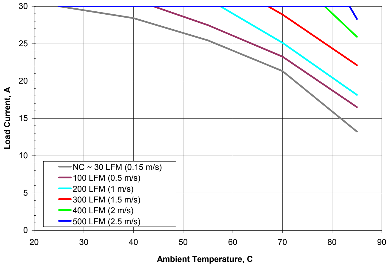
Fig. 1 : Available load current vs. ambient air temperature and airflow rates for converter mounted vertically with air flowing from pin 1 to pin 3, MOSFET temperature \leq 120^{\circ}\text{C} , V_{in} = 48\text{ V} . Note: NC – Natural convection
