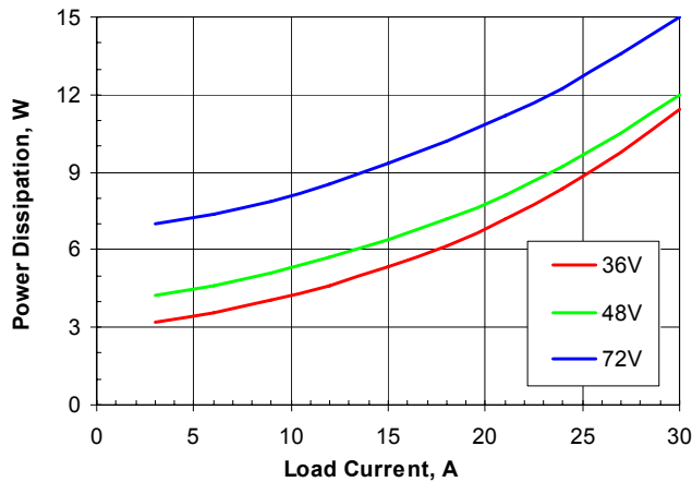
Fig. 4: Power dissipation vs. load current and input voltage for converter mounted vertically with air flowing from pin 1 to pin 3 at a rate of 300 LFM (1.5 m/s) and T_a = 25^\circ\text{C} .
