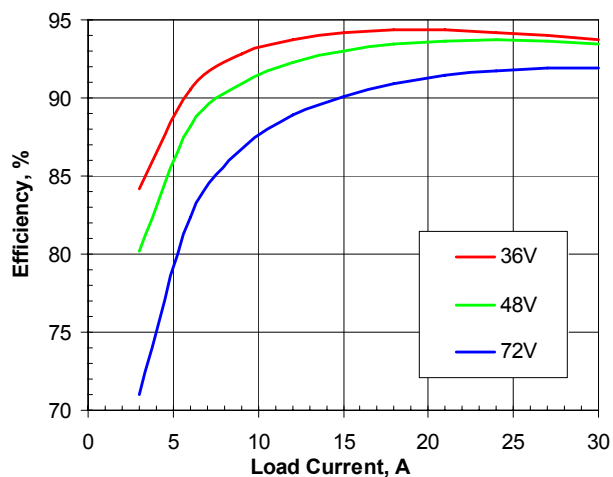
Fig. 2: Efficiency vs. load current and input voltage for converter mounted vertically with air flowing from pin 1 to pin 3 at a rate of 300 LFM (1.5 m/s) and T_a = 25^{\circ}\text{C} .
