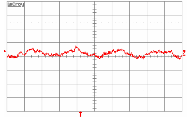
Fig. 13: Input reflected ripple current, i_s (10 mA/div.), measured through 10 \mu H at the source at full rated load current and V_{in} = 48 V. Refer to Fig. 12 for test setup. Time scale: 1 \mu s/div.
