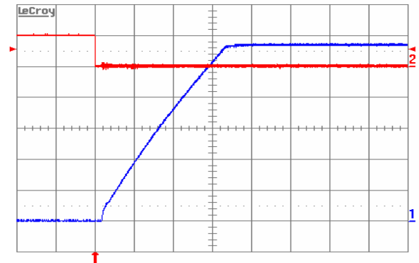
Fig. 7: Turn-on transient at full rated load current (resistive) plus 10,000 \mu\text{F} at V_{in} = 48\text{ V} , triggered via ON/OFF pin. Top trace: ON/OFF signal (5 V/div.). Bottom trace: output voltage (1 V/div.). Time scale: 5 ms/div.
