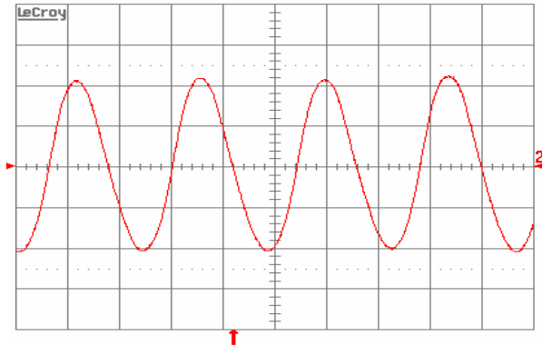
Fig. 12: Input reflected ripple current, i_c (100 mA/div.), measured at input terminals at full rated load current and V_{in} = 48 V. Refer to Fig. 12 for test setup. Time scale: 1 \mu s/div.
