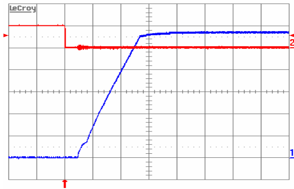
Fig. 6: Turn-on transient at full rated load current (resistive) with no output capacitor at V_{in} = 48\text{ V} , triggered via ON/OFF pin. Top trace: ON/OFF signal (5 V/div.). Bottom trace: output voltage (1 V/div.). Time scale: 2 ms/div.
