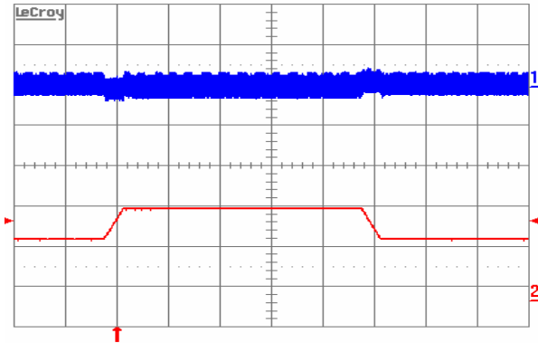
Fig. 8: Output voltage response to load current step-change (15 A – 25 A – 15 A) at V_{in} = 48 V. Top trace: output voltage (100 mV/div.). Bottom trace: load current (10 A/div.). Current slew rate: 0.1 A/ \mu s. C_o = 1 \mu F ceramic. Time scale: 0.2 ms/div.
