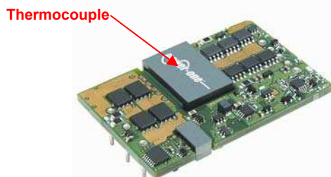
Fig. H: Location of the thermocouple for thermal testing.
