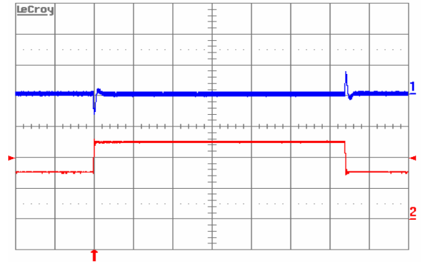
Fig. 9: Output voltage response to load current step-change (15 A – 25 A – 15 A) at V_{in} = 48 V. Top trace: output voltage (200 mV/div.). Bottom trace: load current (10 A/div.). Current slew rate: 5 A/ \mu s. C_o = 470 \mu F POS + 1 \mu F ceramic. Time scale: 0.2 ms/div.
