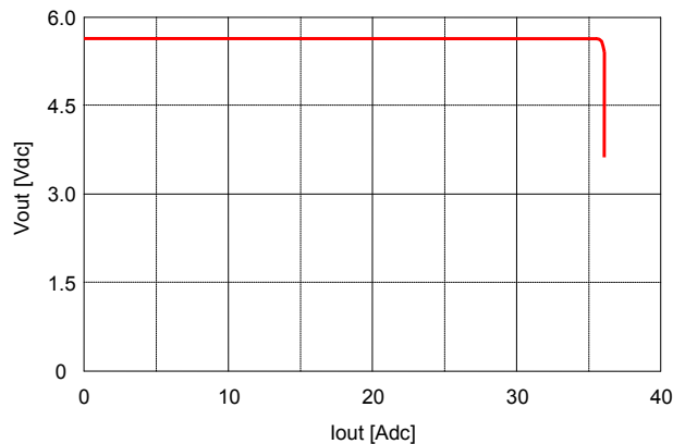
Fig. 14: Output voltage vs. load current showing current limit point and converter shutdown point. Input voltage has almost no effect on current limit characteristic.
