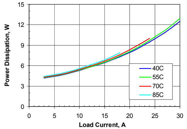
Fig. 5: Power dissipation vs. load current and ambient temperature for converter mounted vertically with V_{in} = 48\text{ V} and air flowing from pin 1 to pin 3 at a rate of 200 LFM (1.0 m/s).
