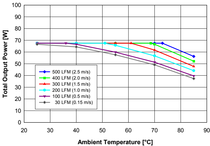
Fig. 1: Available output power vs. ambient air temperature and airflow rates for QD48S012033 converter mounted vertically with air flowing from pin 3 to pin 1, MOSFET temperature \leq 120^{\circ}\text{C} , V_{in} = 48\text{ V} and balanced load on both outputs ( I_{out1} = I_{out2} ).
