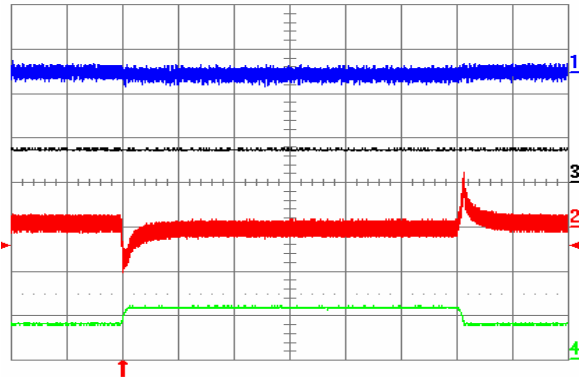
Fig. 21: Output voltage response to lout2 load current step-change of 3.75 A (50%-75%-50%) at lout1 = 7.5 A and V_{in} = 48 V. Ch1 = Vout1 (50 mV/div), Ch2 = Vout2 (50 mV/div), Ch3 = lout1 (10 A/div.), Ch4 = lout2 (10 A/div.). Current slew rate: 0.1 A/ \mu s, C_o = 10 \mu F tantalum + 1 \mu F ceramic. Time scale: 0.5 ms/div.
