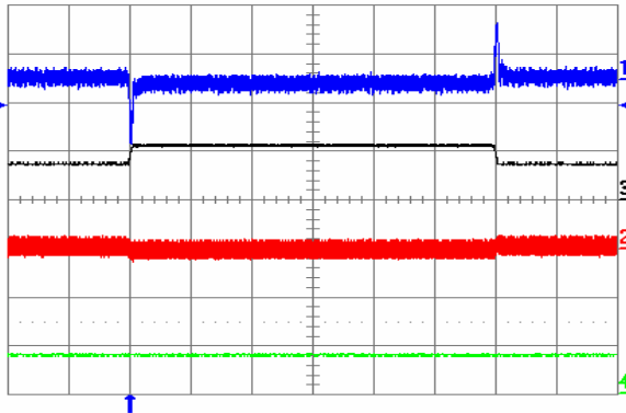
Fig. 20: Output voltage response to lout1 load current step-change of 3.75 A (50%-75%-50%) at lout2 = 7.5 A and V_{in} = 48 V. Ch1 = Vout1 (50 mV/div), Ch2 = Vout2 (50 mV/div), Ch3 = lout1 (10 A/div.), Ch4 = lout2 (10 A/div.). Current slew rate: 0.1 A/ \mu s, C_o = 10 \mu F tantalum + 1 \mu F ceramic. Time scale: 0.5 ms/div.
