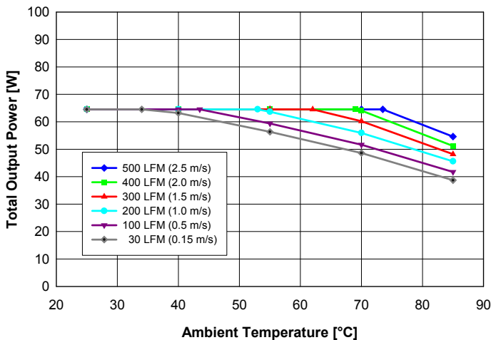
Fig. 1: Available output power vs. ambient air temperature and airflow rates for QD48S018025 converter mounted vertically with air flowing from pin 3 to pin 1, MOSFET temperature \leq 120^{\circ}\text{C} , V_{in} = 48\text{ V} and balanced load on both outputs ( I_{out1} = I_{out2} ).
