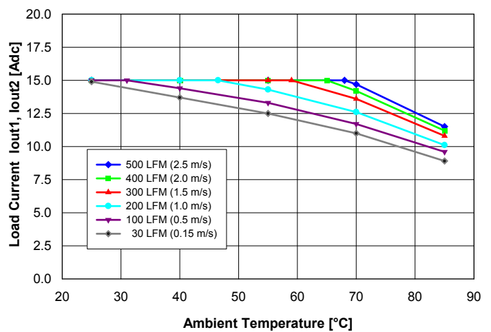
Fig. 11: Available balanced load current (Iout1 = Iout2) vs. ambient temperature and airflow rates for converter mounted horizontally with Vin = 48 V, air flowing from pin 3 to pin 1 and maximum FET temperature ≤ 120°C.
