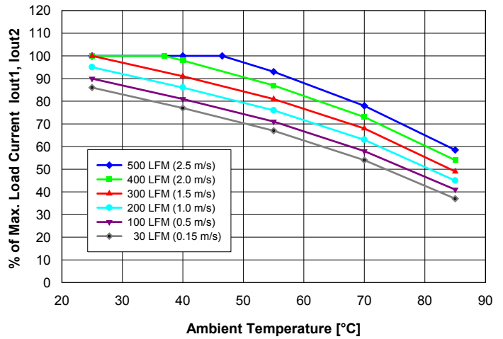
Fig. 15: Available balanced load current (I out1 = 1.5·I out2 ) vs. ambient air temperature and airflow rates for converter mounted vertically with V in = 48 V, air flowing from pin 4 to pin 3 and maximum FET temperature ≤ 120°C.
