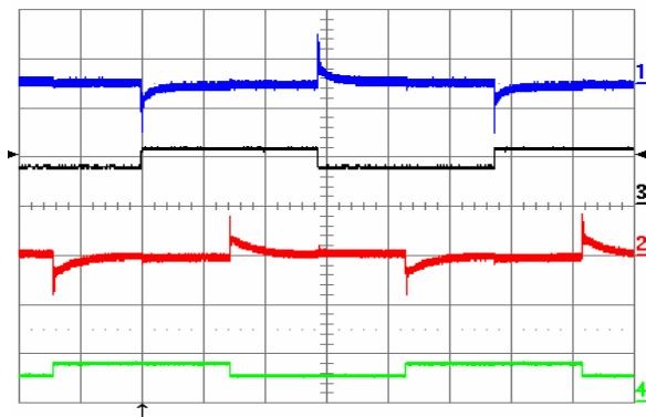
Fig. 29: Output voltage response to both lout1 and lout2 (out of phase) load current step-change of 3.75 A (lout1) and 2.5 A (lout2) (50%-75%-50%) at V_{in} = 48 V. Ch1 = Vout1 (100 mV/div), Ch2 = Vout2 (100 mV/div), Ch3 = lout1 (10 A/div.), Ch4 = lout2 (10 A/div.). Current slew rate: 5 A/ \mu s, C_o = 300 \mu F tantalum + 1 \mu F ceramic. Time scale: 1 ms/div.
