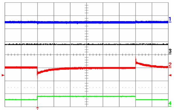
Fig. 27: Output voltage response to Iout2 load current step-change of 2.5 A (50%-75%-50%) at Iout1 = 7.5 A and Vin = 48 V. Ch1 = Vout1 (100 mV/div), Ch2 = Vout2 (100 mV/div), Ch3 = Iout1 (10 A/div.), Ch4 = Iout2 (10 A/div.). Current slew rate: 5 A/μs, Co = 300 μF tantalum + 1 μF ceramic. Time scale: 0.5 ms/div.
