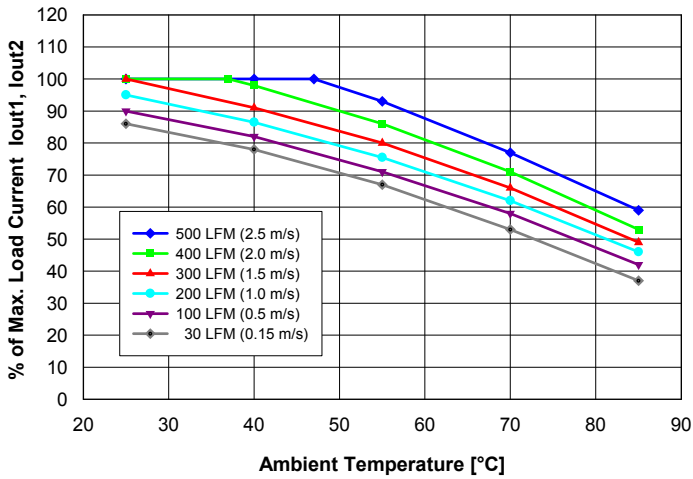
Fig. 14: Available balanced load current (I out1 = 1.5·I out2 ) vs. ambient air temperature and airflow rates for converter mounted vertically with V in = 48 V, air flowing from pin 3 to pin 4 and maximum FET temperature ≤ 120°C.
