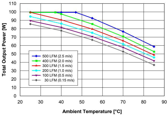
Fig. 12: Available output power for balanced load current (I out1 = 1.5·I out2 ) vs. ambient air temperature and airflow rates for converter mounted vertically with V in = 48 V, air flowing from pin 3 to pin 4 and maximum FET temperature ≤ 120°C.
