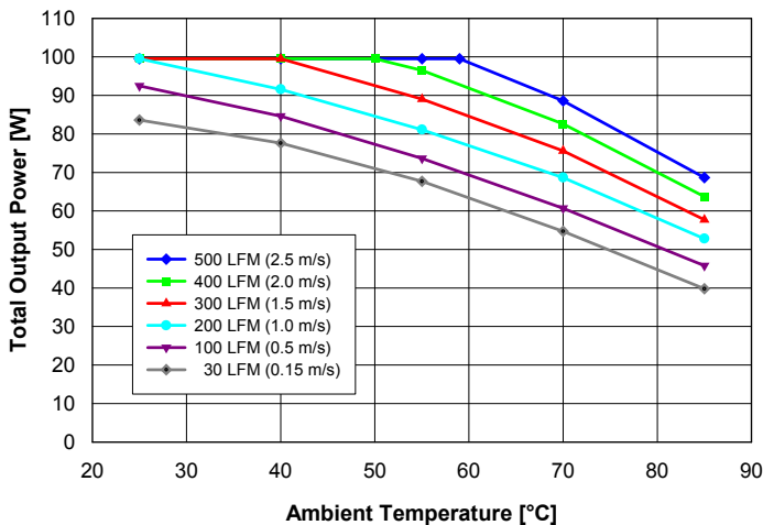
Fig. 1: Available output power vs. ambient air temperature and airflow rates for QD48S033050 converter mounted vertically with air flowing from pin 3 to pin 1, MOSFET temperature \leq 120^{\circ}\text{C} , V_{in} = 48\text{ V} and balanced load on both outputs ( I_{out1} = 1.5 \cdot I_{out2} ).
