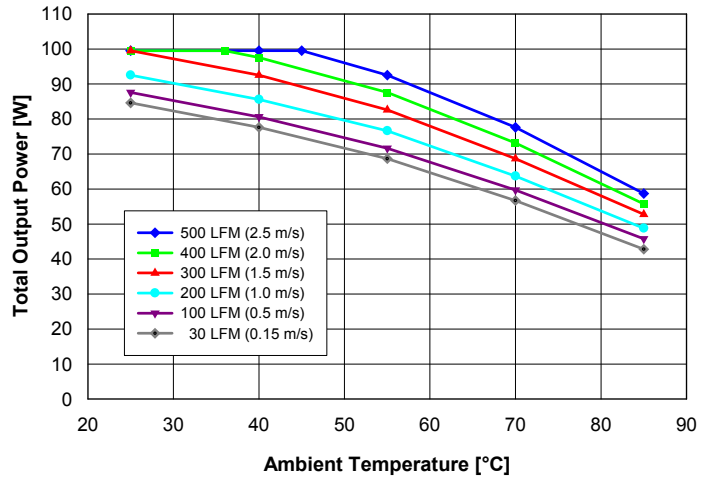
Fig. 9: Available output power for balanced load current ( I_{out1} = 1.5 \cdot I_{out2} ) vs. ambient air temperature and airflow rates for converter mounted horizontally with V_{in} = 48\text{ V} , air flowing from pin 3 to pin 4 and maximum FET temperature \leq 120^\circ\text{C} .
