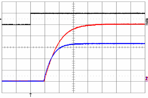
Fig. 23: Turn-on transient waveforms at full rated load current (resistive) and V_{in} = 48\text{ V} , triggered via ON/OFF pin. Top trace: ON/OFF signal (5 V/div.). Bottom traces: V_{out1} (blue, 1 V/div.), V_{out2} (red, 1 V/div.). Time scale: 1 ms/div.
