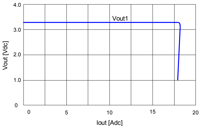
Fig. 30: Output voltage Vout1 vs. load current lout1 showing current limit point and converter shutdown point. When Vout1 is in current limit, Vout2 is not affected until Vout1 reaches the shut-down threshold of 1 V. Input voltage has almost no effect on Vout1 current limit characteristic.
