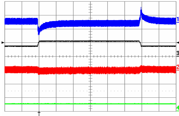
Fig. 24: Output voltage response to Iout1 load current step-change of 3.75 A (50%-75%-50%) at Iout2 = 5 A and Vin = 48 V. Ch1 = Vout1 (50 mV/div), Ch2 = Vout2 (50 mV/div), Ch3 = Iout1 (10 A/div.), Ch4 = Iout2 (10 A/div.). Current slew rate: 0.1 A/μs, Co = 10 μF tantalum + 1 μF ceramic. Time scale: 0.5 ms/div.
