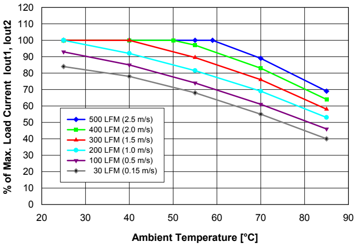
Fig. 10: Available balanced load current ( I_{out1} = 1.5 \cdot I_{out2} ) vs. ambient air temperature and airflow rates for converter mounted vertically with V_{in} = 48\text{ V} , air flowing from pin 3 to pin 1 and maximum FET temperature \leq 120^\circ\text{C} .
