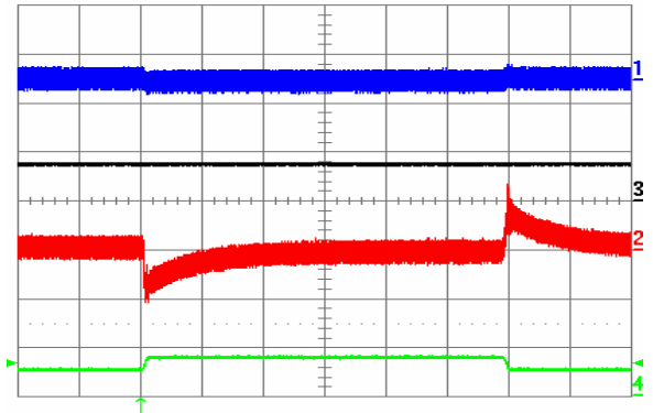
Fig. 25: Output voltage response to Iout2 load current step-change of 2.5 A (50%-75%-50%) at Iout1 = 7.5 A and Vin = 48 V. Ch1 = Vout1 (50 mV/div), Ch2 = Vout2 (50 mV/div), Ch3 = Iout1 (10 A/div.), Ch4 = Iout2 (10 A/div.). Current slew rate: 0.1 A/μs, Co = 10 μF tantalum + 1 μF ceramic. Time scale: 0.5 ms/div.
