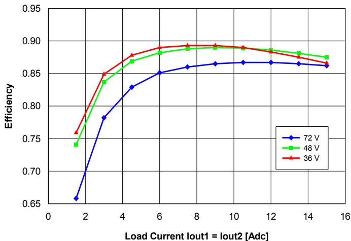
Fig. 21: Efficiency vs. balanced load current ( I_{out1}/I_{out2} = \text{const.} ) and input voltage for converter mounted horizontally with air flowing from pin 3 to pin 4 at a rate of 300 LFM (1.5 m/s) and T_a = 25^\circ\text{C} .
