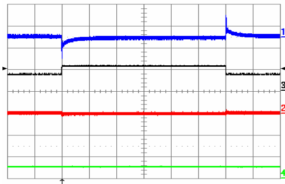
Fig. 26: Output voltage response to Iout1 load current step-change of 3.75 A (50%-75%-50%) at Iout2 = 5 A and Vin = 48 V. Ch1 = Vout1 (100 mV/div), Ch2 = Vout2 (100 mV/div), Ch3 = Iout1 (10 A/div.), Ch4 = Iout2 (10 A/div.). Current slew rate: 5 A/μs, Co = 300 μF tantalum + 1 μF ceramic. Time scale: 0.5 ms/div.
