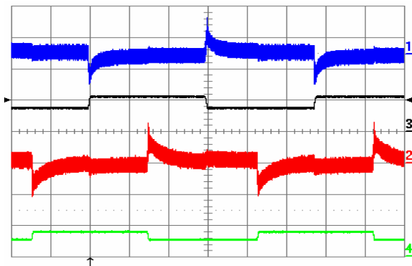
Fig. 28: Output voltage response to both lout1 and lout2 (out of phase) load current step-change of 3.75 A (lout1) and 2.5 A (lout2) (50%-75%-50%) at V_{in} = 48 V. Ch1 = Vout1 (50 mV/div), Ch2 = Vout2 (50 mV/div), Ch3 = lout1 (10 A/div.), Ch4 = lout2 (10 A/div.). Current slew rate: 0.1 A/ \mu s, C_o = 10 \mu F tantalum + 1 \mu F ceramic. Time scale: 1 ms/div.
