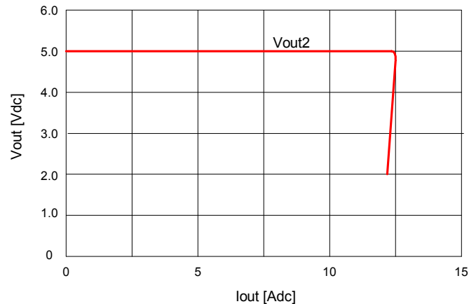
Fig. 31: Output voltage Vout2 vs. load current lout2 showing current limit point and converter shutdown point. When Vout2 is in current limit, Vout1 will follow with less than 1 V difference until Vout2 reaches shut-down threshold of 2 V. Input voltage has almost no effect on Vout2 current limit characteristic.
