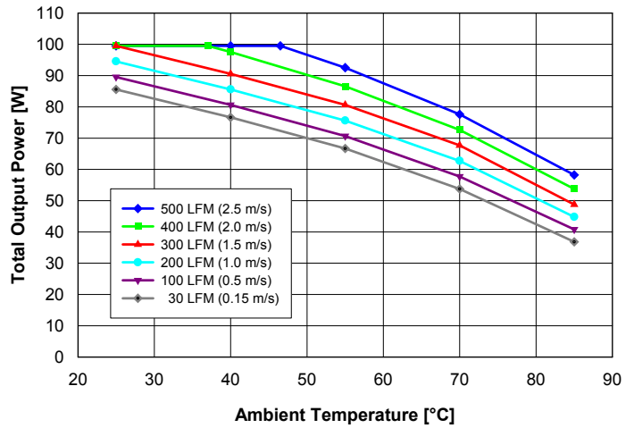
Fig. 13: Available output power for balanced load current (I out1 = 1.5·I out2 ) vs. ambient air temperature and airflow rates for converter mounted vertically with V in = 48 V, air flowing from pin 4 to pin 3 and maximum FET temperature ≤ 120°C.
