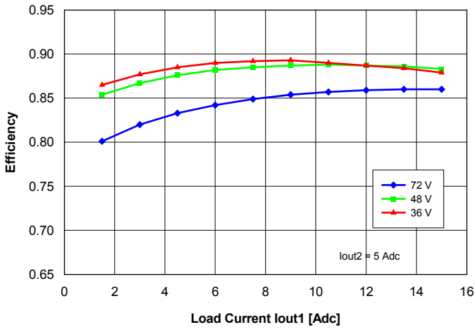
Fig. 16: Efficiency vs. load current Iout1 and input voltage for converter mounted vertically with air flowing from pin 3 to pin 1 at a rate of 300 LFM (1.5 m/s), for Iout2 = 5 A and Ta = 25°C.
