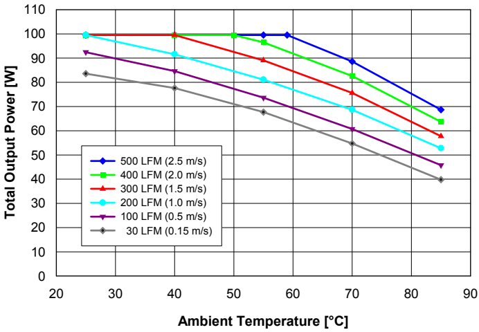
Fig. 8: Available output power for balanced load current ( I_{out1} = 1.5 \cdot I_{out2} ) vs. ambient air temperature and airflow rates for converter mounted vertically with V_{in} = 48\text{ V} , air flowing from pin 3 to pin 1 and maximum FET temperature \leq 120^\circ\text{C} .
