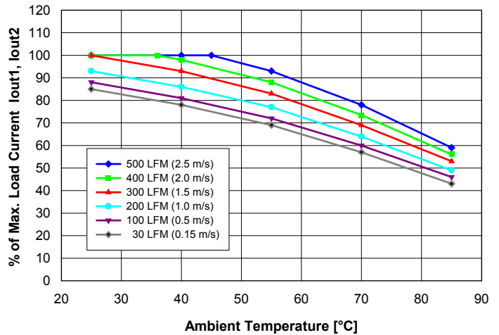
Fig. 11: Available balanced load current ( I_{out1} = 1.5 \cdot I_{out2} ) vs. ambient temperature and airflow rates for converter mounted horizontally with V_{in} = 48\text{ V} , air flowing from pin 3 to pin 4 and maximum FET temperature \leq 120^\circ\text{C} .
