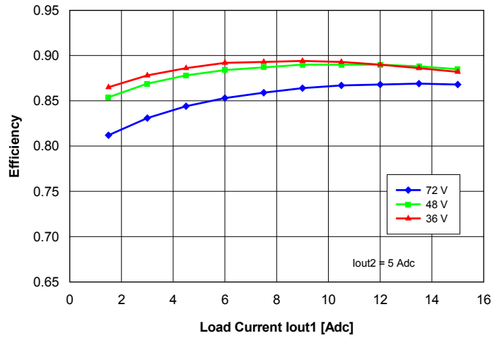
Fig. 17: Efficiency vs. load current Iout1 and input voltage for converter mounted horizontally with air flowing from pin 3 to pin 4 at a rate of 300 LFM (1.5 m/s), for Iout2 = 5 A and Ta = 25°C.
