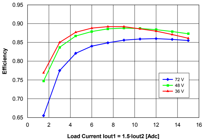
Fig. 20: Efficiency vs. balanced load current ( I_{out1} = 1.5 \cdot I_{out2} ) and input voltage for converter mounted vertically with air flowing from pin 3 to pin 1 at a rate of 300 LFM (1.5 m/s) and T_a = 25^\circ\text{C} .
