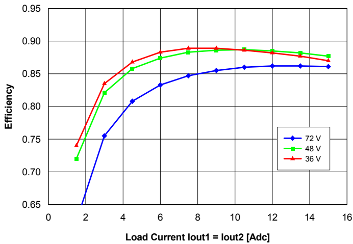
Fig. 16: Efficiency vs. balanced load current ( I_{out1} = I_{out2} ) and input voltage for converter mounted vertically with air flowing from pin 3 to pin 1 at a rate of 300 LFM (1.5 m/s) and T_a = 25^\circ\text{C} .
