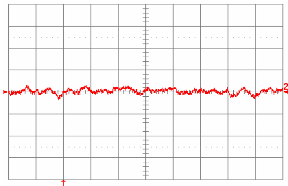
Fig. 33: Input reflected ripple current, i_s (10 mA/div), measured through 10 \mu H at the source at full rated load current on both outputs and V_{in} = 48 V. Refer to Fig. 35 for test setup. Time scale: 1 \mu s/div.
