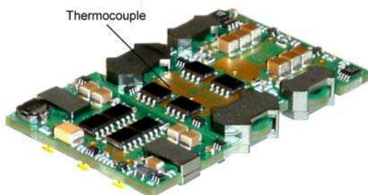
Fig. 34: Location of the thermocouple for thermal testing.
