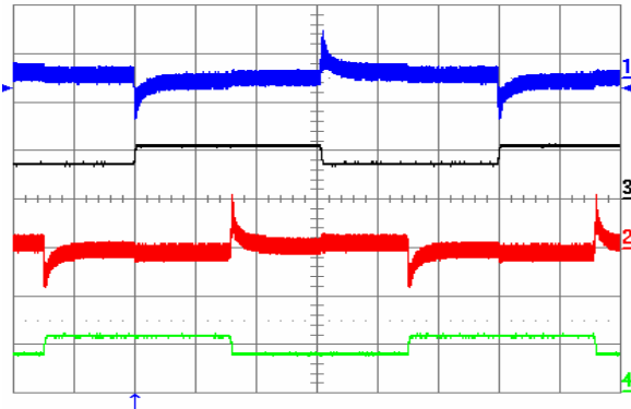
Fig. 24: Output voltage response to both Iout1 and Iout2 (out of phase) load current step-change of 3.75 A (50%-75%-50%) at V_{in} = 48 V. Ch1 = Vout1 (50 mV/div), Ch2 = Vout2 (50 mV/div), Ch3 = Iout1 (10 A/div.), Ch4 = Iout2 (10 A/div.). Current slew rate: 0.1 A/ \mu s, C_o = 10 \mu F tantalum + 1 \mu F ceramic. Time scale: 1 ms/div.
