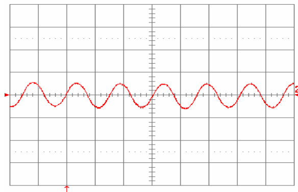
Fig. 32: Input reflected ripple current, i_c (100 mA/div), measured at input terminals at full rated load current on both outputs and V_{in} = 48 V. Refer to Fig. 35 for test setup. Time scale: 1 \mu s/div.
