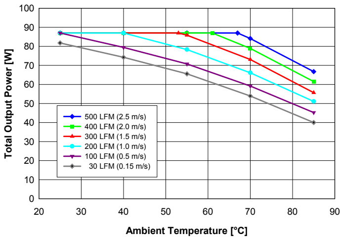
Fig. 1: Available output power vs. ambient air temperature and airflow rates for QD48S025033 converter mounted vertically with air flowing from pin 3 to pin 1, MOSFET temperature \leq 120^{\circ}\text{C} , V_{in} = 48\text{ V} and balanced load on both outputs ( I_{out1} = I_{out2} ).
