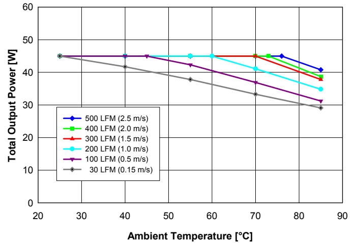
Fig. 9: Available output power for balanced load current ( I_{out1} = I_{out2} ) vs. ambient air temperature and airflow rates for converter with A height pins mounted horizontally with V_{in} = 48\text{ V} , air flowing from pin 3 to pin 1 and maximum FET temperature \leq 120^\circ\text{C} .
