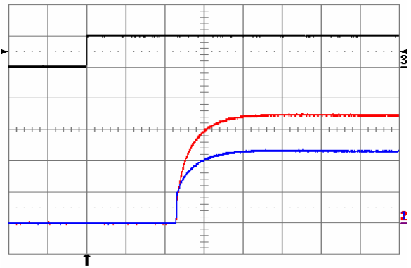
Fig. 19: Turn-on transient waveforms at full rated load current (resistive) and V in = 48 V, triggered via ON/OFF pin. Top trace: ON/OFF signal (5 V/div.). Bottom traces: V out1 (blue, 0.5 V/div.), V out2 (red, 0.5 V/div.). Time scale: 1 ms/div.
