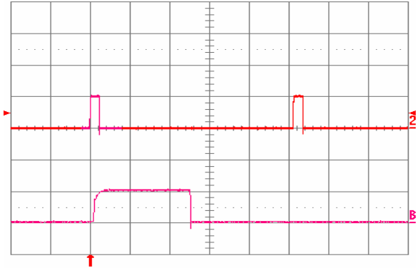
Fig. 29: Load current i_{out2} into a 10 mΩ short circuit on V_{out2} during restart, with V_{out1} open (no load), at V_{in} = 48 V. Ch2 = i_{out2} (20 A/div, 20 ms/div). ChB = i_{out2} (20 A/div, 2 ms/div) is an expansion of the on-time portion of i_{out2} .
