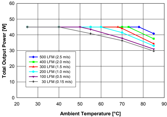
Fig. 8: Available output power for balanced load current ( I_{out1} = I_{out2} ) vs. ambient air temperature and airflow rates for converter with A height pins mounted vertically with V_{in} = 48\text{ V} , air flowing from pin 3 to pin 1 and maximum FET temperature \leq 120^\circ\text{C} .
