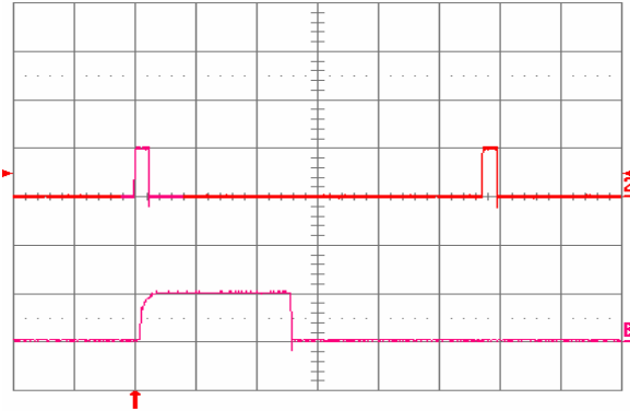
Fig. 28: Load current i_{out1} into a 10 mΩ short circuit on V_{out1} during restart, with V_{out2} open (no load), at V_{in} = 48 V. Ch2 = i_{out1} (20 A/div, 20 ms/div). ChB = i_{out1} (20 A/div, 2 ms/div) is an expansion of the on-time portion of i_{out1} .
