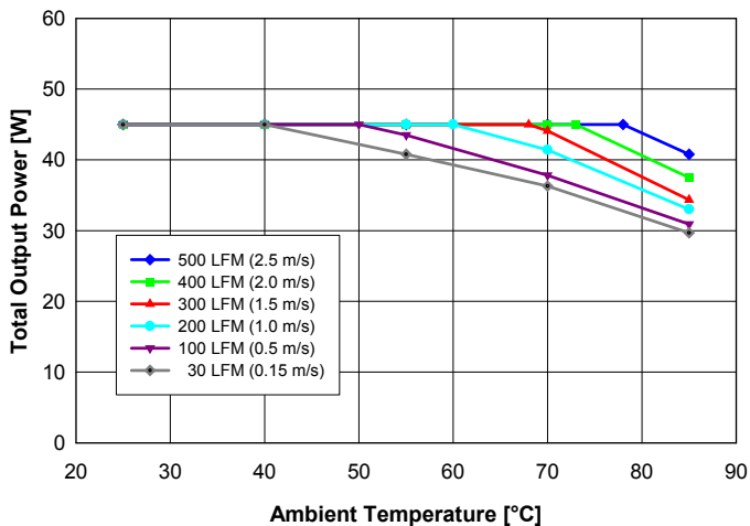
Fig. 1: Available output power vs. ambient air temperature and airflow rates for QD48T012018 converter with A height pins mounted vertically with air flowing from pin 3 to pin 1, MOSFET temperature \leq 120^\circ\text{C} , V_{in} = 48\text{ V} and balanced load on both outputs ( I_{out1} = I_{out2} ).
