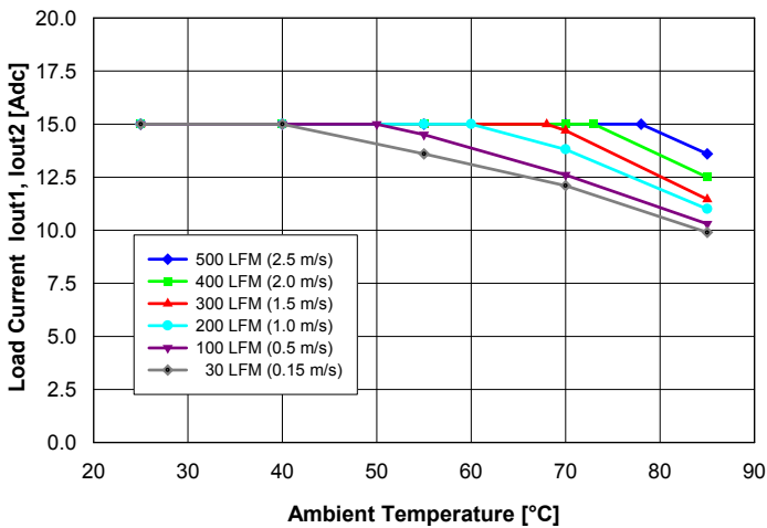
Fig. 10: Available balanced load current ( I_{out1} = I_{out2} ) vs. ambient air temperature and airflow rates for converter with A height pins mounted vertically with V_{in} = 48\text{ V} , air flowing from pin 3 to pin 1 and maximum FET temperature \leq 120^\circ\text{C} .
