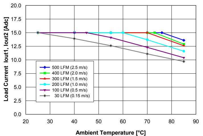
Fig. 11: Available balanced load current ( I_{out1} = I_{out2} ) vs. ambient temperature and airflow rates for converter mounted with A height pins horizontally with V_{in} = 48\text{ V} , air flowing from pin 3 to pin 1 and maximum FET temperature \leq 120^\circ\text{C} .
