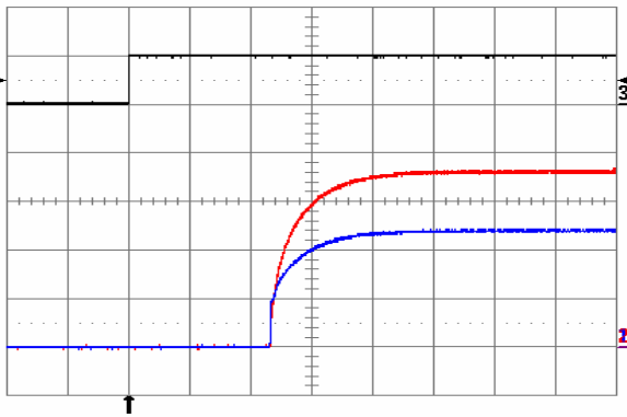
Fig. 18: Turn-on transient waveforms at no load current and V in = 48 V, triggered via ON/OFF pin. Top trace: ON/OFF signal (5 V/div.). Bottom traces: V out1 (blue, 0.5 V/div.), V out2 (red, 0.5 V/div.). Time scale: 1 ms/div.
