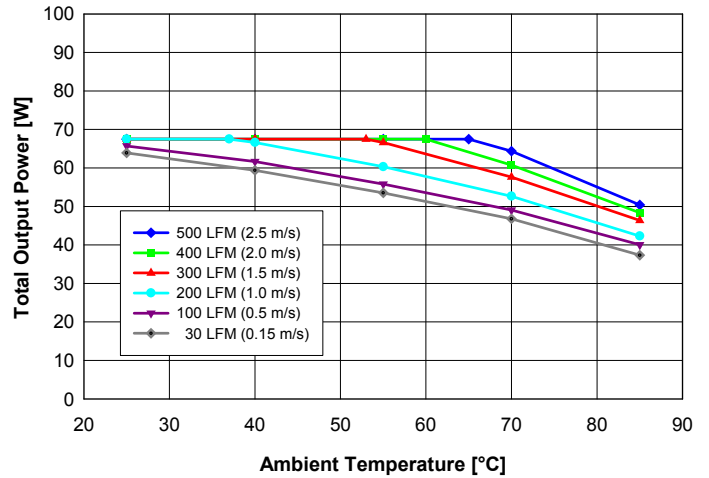
Fig. 9: Available output power for balanced load current (Iout1 = Iout2) vs. ambient air temperature and airflow rates for converter mounted horizontally with Vin = 48 V, air flowing from pin 3 to pin 4 and maximum FET temperature ≤ 120°C.
