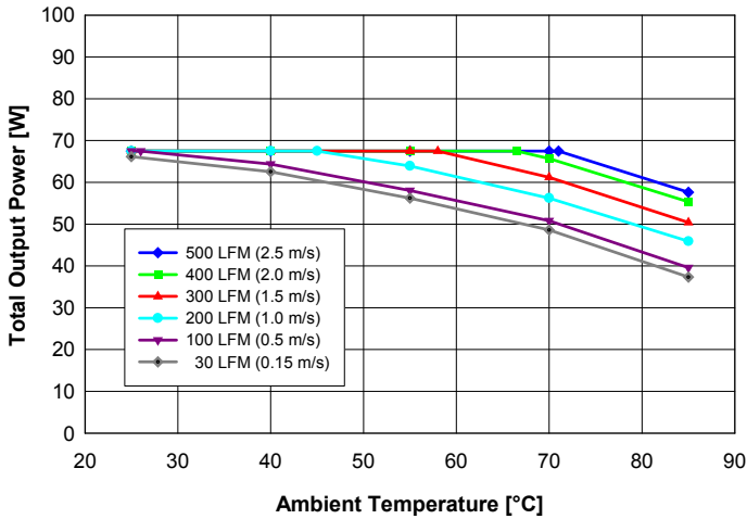
Fig. 8: Available output power for balanced load current (Iout1 = Iout2) vs. ambient air temperature and airflow rates for converter mounted vertically with Vin = 48 V, air flowing from pin 3 to pin 1 and maximum FET temperature ≤ 120°C.
