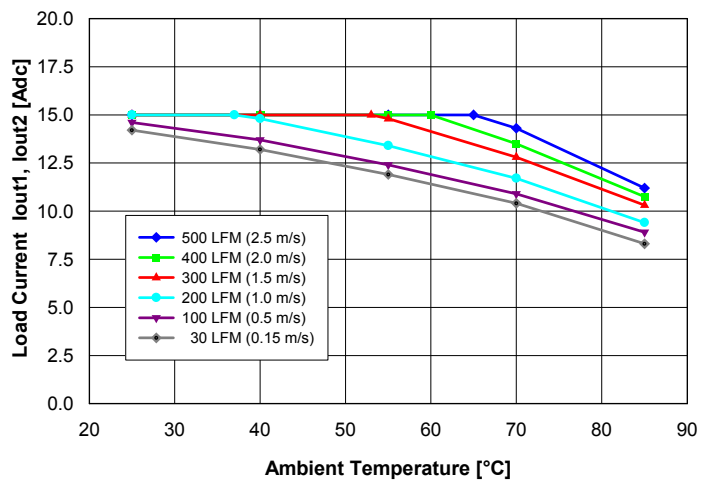
Fig. 11: Available balanced load current (Iout1 = Iout2) vs. ambient temperature and airflow rates for converter mounted horizontally with Vin = 48 V, air flowing from pin 3 to pin 4 and maximum FET temperature ≤ 120°C.
