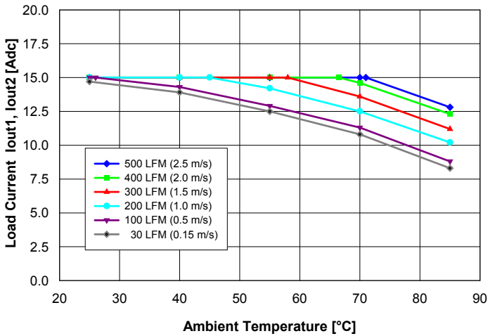
Fig. 10: Available balanced load current (Iout1 = Iout2) vs. ambient air temperature and airflow rates for converter mounted vertically with Vin = 48 V, air flowing from pin 3 to pin 1 and maximum FET temperature ≤ 120°C.
