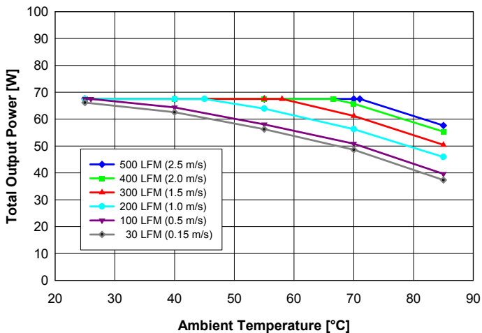
Fig. 1: Available output power vs. ambient air temperature and airflow rates for QD48T012033 converter mounted vertically with air flowing from pin 3 to pin 1, MOSFET temperature \leq 120^{\circ}\text{C} , V_{in} = 48\text{ V} and balanced load on both outputs ( I_{out1} = I_{out2} ).
