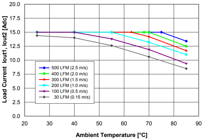
Fig. 10: Available balanced load current ( I_{out1} = I_{out2} ) vs. ambient air temperature and airflow rates for converter with D height pins mounted vertically with V_{in} = 48\text{ V} , air flowing from pin 3 to pin 1 and maximum FET temperature \leq 120^\circ\text{C} .
