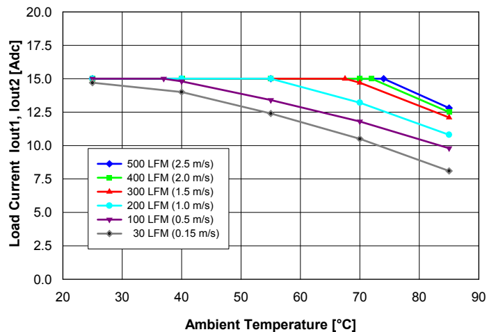
Fig. 11: Available balanced load current ( I_{out1} = I_{out2} ) vs. ambient temperature and airflow rates for converter mounted with D height pins horizontally with V_{in} = 48\text{ V} , air flowing from pin 3 to pin 1 and maximum FET temperature \leq 120^\circ\text{C} .
