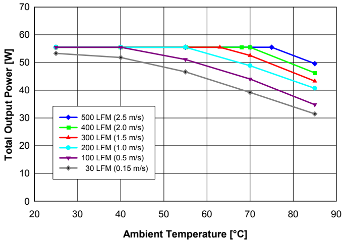
Fig. 8: Available output power for balanced load current ( I_{out1} = I_{out2} ) vs. ambient air temperature and airflow rates for converter with D height pins mounted vertically with V_{in} = 48\text{ V} , air flowing from pin 3 to pin 1 and maximum FET temperature \leq 120^\circ\text{C} .
