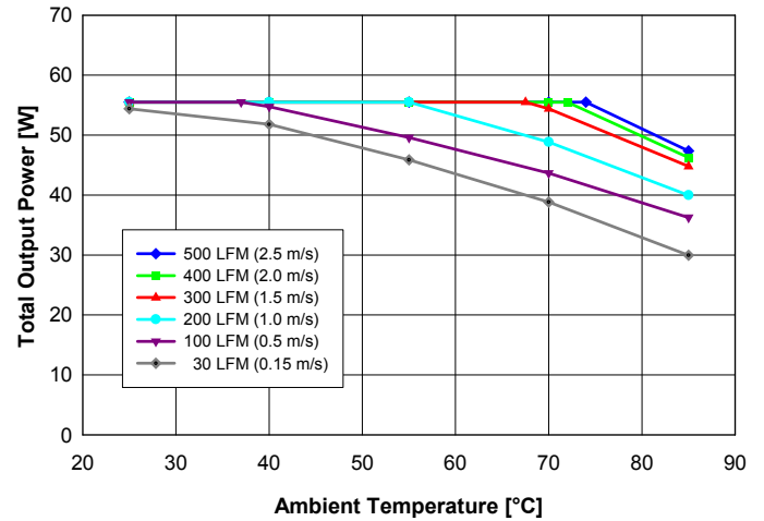
Fig. 9: Available output power for balanced load current ( I_{out1} = I_{out2} ) vs. ambient air temperature and airflow rates for converter with D height pins mounted horizontally with V_{in} = 48\text{ V} , air flowing from pin 3 to pin 1 and maximum FET temperature \leq 120^\circ\text{C} .
