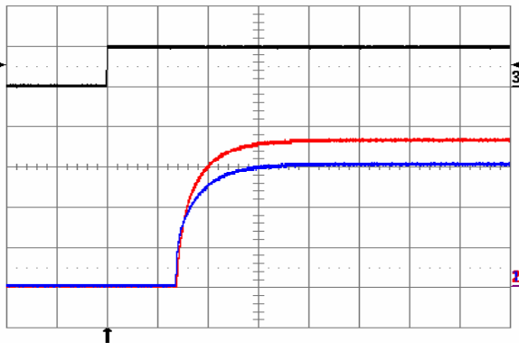
Fig. 18: Turn-on transient waveforms at no load current and V_{in} = 48\text{ V} , triggered via ON/OFF pin. Top trace: ON/OFF signal (5 V/div.). Bottom traces: V_{out1} (blue, 0.5 V/div.), V_{out2} (red, 0.5 V/div.). Time scale: 1 ms/div.
