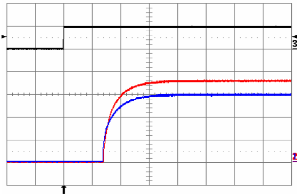
Fig. 19: Turn-on transient waveforms at full rated load current (resistive) and V_{in} = 48\text{ V} , triggered via ON/OFF pin. Top trace: ON/OFF signal (5 V/div.). Bottom traces: V_{out1} (blue, 0.5 V/div.), V_{out2} (red, 0.5 V/div.). Time scale: 1 ms/div.
