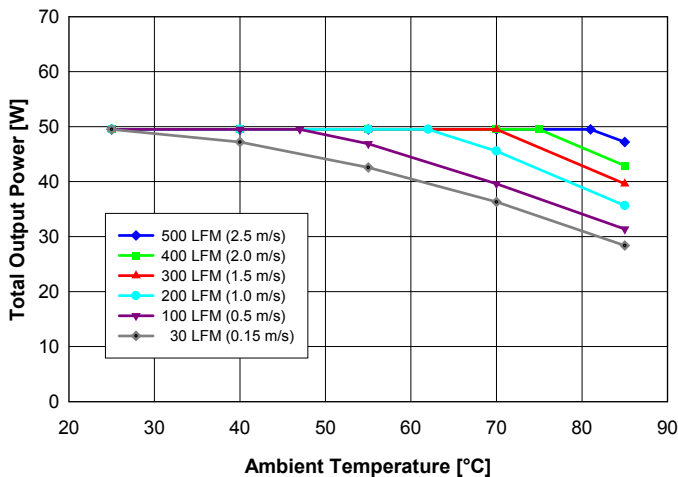
Fig. 1: Available output power vs. ambient air temperature and airflow rates for QD48T015018 converter with D height pins mounted vertically with air flowing from pin 3 to pin 1, MOSFET temperature \leq 120^{\circ}\text{C} , V_{in} = 48\text{ V} and balanced load on both outputs ( I_{out1} = I_{out2} ).
