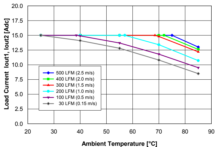
Fig. 11: Available balanced load current ( I_{out1} = I_{out2} ) vs. ambient temperature and airflow rates for converter with D height pins mounted horizontally with V_{in} = 48\text{ V} , air flowing from pin 3 to pin 1 and maximum FET temperature \leq 120^\circ\text{C} .
