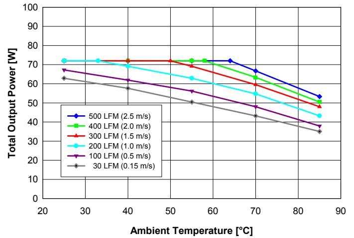
Fig. 9: Available output power for balanced load current ( I_{out1} = I_{out2} ) vs. ambient air temperature and airflow rates for converter with A height pins mounted horizontally with V_{in} = 48 V, air flowing from pin 3 to pin 1 and maximum FET temperature \leq 120^{\circ}\text{C} .
