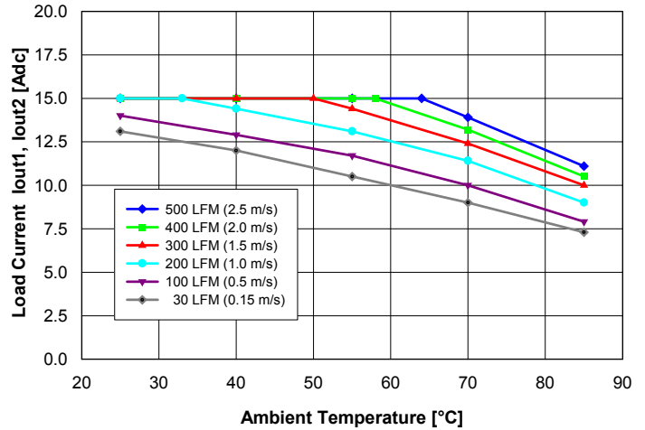
Fig. 11: Available balanced load current ( I_{out1} = I_{out2} ) vs. ambient temperature and airflow rates for converter mounted with A height pins horizontally with V_{in} = 48 V, air flowing from pin 3 to pin 1 and maximum FET temperature \leq 120^{\circ}\text{C} .
