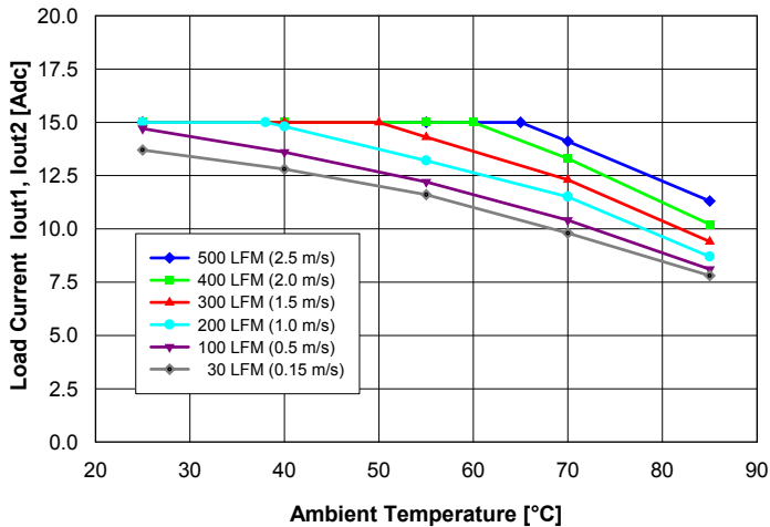
Fig. 10: Available balanced load current ( I_{out1} = I_{out2} ) vs. ambient air temperature and airflow rates for converter with A height pins mounted vertically with V_{in} = 48 V, air flowing from pin 3 to pin 1 and maximum FET temperature \leq 120^{\circ}\text{C} .
