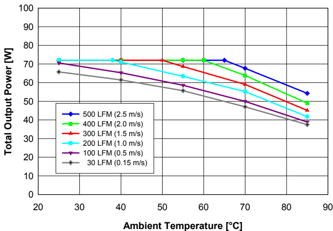
Fig. 1: Available output power vs. ambient air temperature and airflow rates for QD48T015033 converter with A height pins mounted vertically with air flowing from pin 3 to pin 1, MOSFET temperature \leq 120^{\circ}\text{C} , V_{in} = 48\text{ V} and balanced load on both outputs ( I_{out1} = I_{out2} ).
