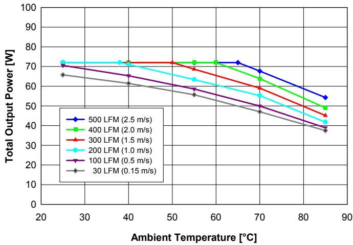
Fig. 8: Available output power for balanced load current ( I_{out1} = I_{out2} ) vs. ambient air temperature and airflow rates for converter with A height pins mounted vertically with V_{in} = 48 V, air flowing from pin 3 to pin 1 and maximum FET temperature \leq 120^{\circ}\text{C} .
