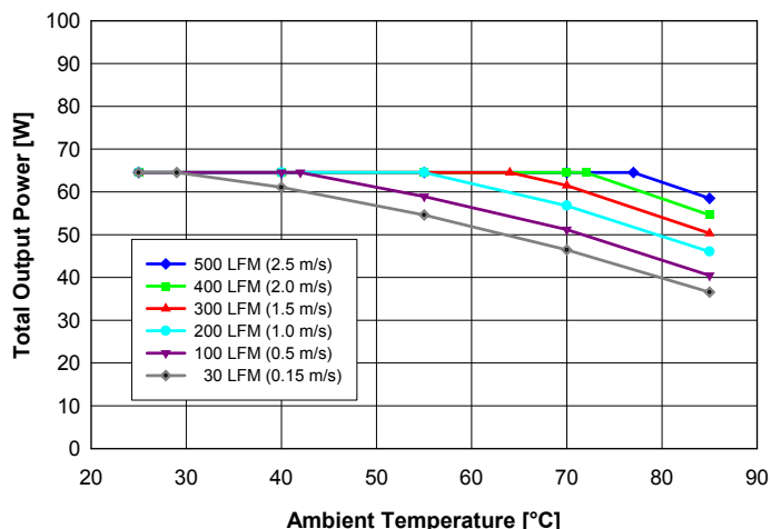
Fig. 1: Available output power vs. ambient air temperature and airflow rates for QD48T018025 converter with D height pins mounted vertically with air flowing from pin 3 to pin 1, MOSFET temperature \leq 120^{\circ}\text{C} , V_{in} = 48\text{ V} and balanced load on both outputs ( I_{out1} = I_{out2} ).
