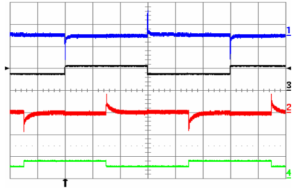
Fig. 25: Output voltage response to both Iout1 and Iout2 (out of phase) load current step-change of 3.75 A (Iout1) and 2.5 A (Iout2) (50%-75%-50%) at V_{in} = 48 V. Ch1 = Vout1 (100 mV/div), Ch2 = Vout2 (100 mV/div), Ch3 = Iout1 (10 A/div.), Ch4 = Iout2 (10 A/div.). Current slew rate: 5 A/ \mu s, C_o = 300 \mu F tantalum + 1 \mu F ceramic. Time scale: 1 ms/div.
