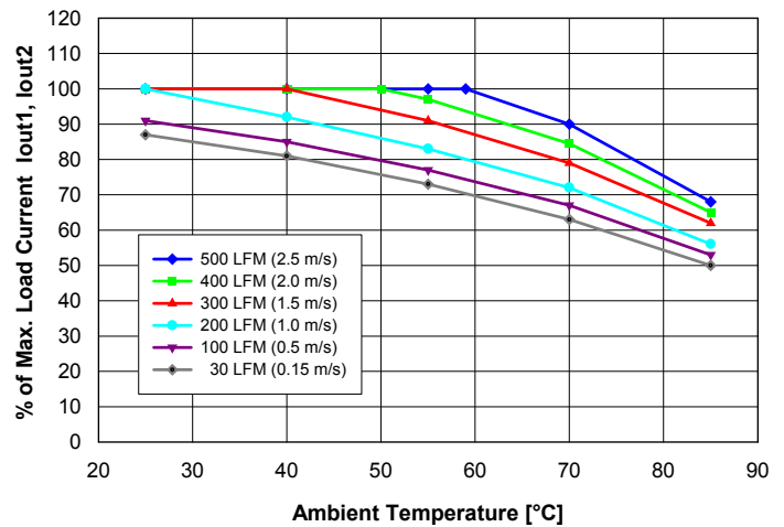
Fig. 11: Available balanced load current ( I_{out1} = 1.5 \cdot I_{out2} ) vs. ambient air temperature and airflow rates for converter mounted horizontally with V_{in} = 48 V, air flowing from pin 3 to pin 4 and maximum FET temperature \leq 120^{\circ}\text{C} .
