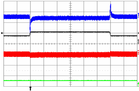
Fig. 20: Output voltage response to Iout1 load current step-change of 3.75 A (50%-75%-50%) at Iout2 = 5 A and Vin = 48 V. Ch1 = Vout1 (50 mV/div), Ch2 = Vout2 (50 mV/div), Ch3 = Iout1 (10 A/div.), Ch4 = Iout2 (10 A/div.). Current slew rate: 0.1 A/ \mu s, Co = 10 \mu F tantalum + 1 \mu F ceramic. Time scale: 0.5 ms/div.
