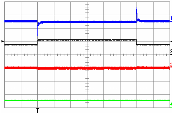
Fig. 22: Output voltage response to Iout1 load current step-change of 3.75 A (50%-75%-50%) at Iout2 = 5 A and Vin = 48 V. Ch1 = Vout1 (100 mV/div), Ch2 = Vout2 (100 mV/div), Ch3 = Iout1 (10 A/div.), Ch4 = Iout2 (10 A/div.). Current slew rate: 5 A/ \mu s, Co = 300 \mu F tantalum + 1 \mu F ceramic. Time scale: 0.5 ms/div.
