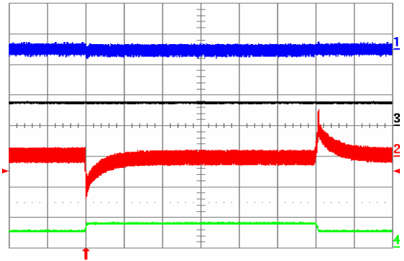
Fig. 21: Output voltage response to Iout2 load current step-change of 2.5 A (50%-75%-50%) at Iout1 = 7.5 A and Vin = 48 V. Ch1 = Vout1 (50 mV/div), Ch2 = Vout2 (50 mV/div), Ch3 = Iout1 (10 A/div.), Ch4 = Iout2 (10 A/div.). Current slew rate: 0.1 A/ \mu s, Co = 10 \mu F tantalum + 1 \mu F ceramic. Time scale: 0.5 ms/div.
