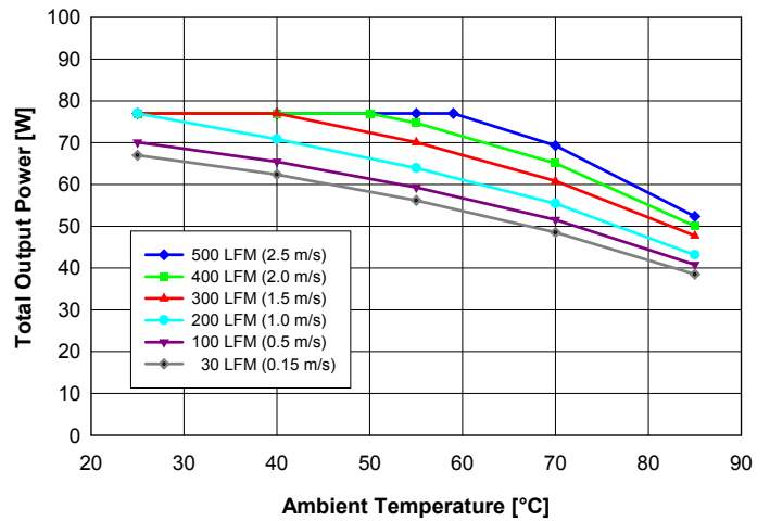
Fig. 9: Available output power for balanced load current ( I_{out1} = 1.5 \cdot I_{out2} ) vs. ambient air temperature and airflow rates for converter mounted horizontally with V_{in} = 48 V, air flowing from pin 3 to pin 4 and maximum FET temperature \leq 120^{\circ}\text{C} .
