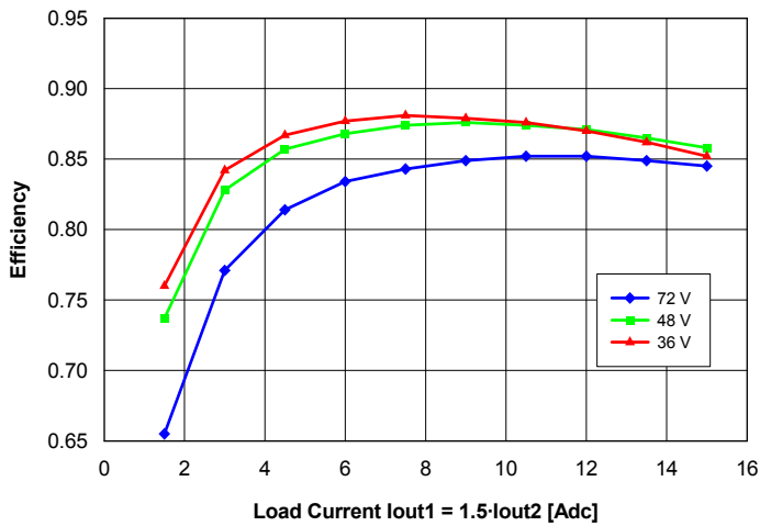
Fig. 16: Efficiency vs. balanced load current ( I_{out1} = 1.5 \cdot I_{out2} ) and input voltage for converter mounted vertically with air flowing from pin 3 to pin 1 at a rate of 300 LFM (1.5 m/s) and T_a = 25^\circ\text{C} .
