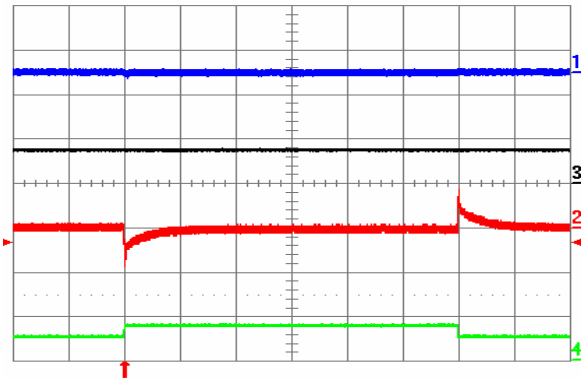
Fig. 23: Output voltage response to Iout2 load current step-change of 2.5 A (50%-75%-50%) at Iout1 = 7.5 A and Vin = 48 V. Ch1 = Vout1 (100 mV/div), Ch2 = Vout2 (100 mV/div), Ch3 = Iout1 (10 A/div.), Ch4 = Iout2 (10 A/div.). Current slew rate: 5 A/ \mu s, Co = 300 \mu F tantalum + 1 \mu F ceramic. Time scale: 0.5 ms/div.
