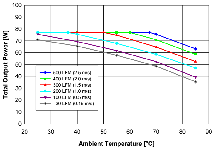
Fig. 1: Available output power vs. ambient air temperature and airflow rates for QD48T018050 converter mounted vertically with air flowing from pin 3 to pin 1, MOSFET temperature \leq 120^{\circ}\text{C} , V_{in} = 48\text{ V} and balanced load on both outputs ( I_{out1} = 1.5 \cdot I_{out2} ).
