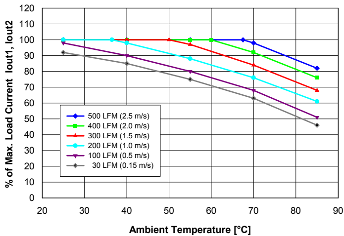
Fig. 10: Available balanced load current ( I_{out1} = 1.5 \cdot I_{out2} ) vs. ambient air temperature and airflow rates for converter mounted vertically with V_{in} = 48 V, air flowing from pin 3 to pin 1 and maximum FET temperature \leq 120^{\circ}\text{C} .
