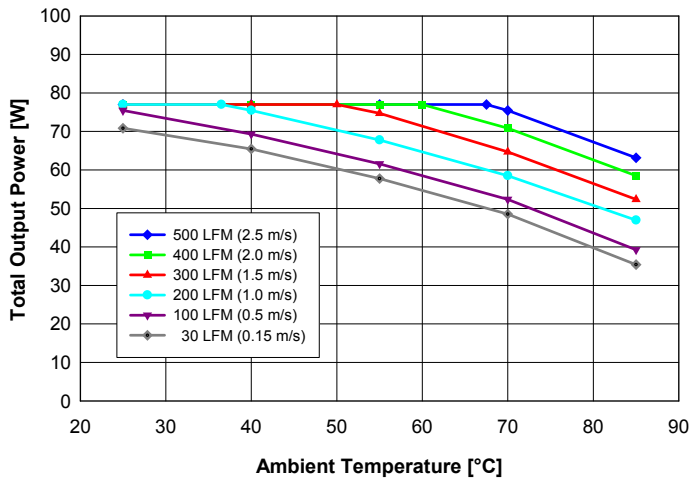
Fig. 8: Available output power for balanced load current ( I_{out1} = 1.5 \cdot I_{out2} ) vs. ambient air temperature and airflow rates for converter mounted vertically with V_{in} = 48 V, air flowing from pin 3 to pin 1 and maximum FET temperature \leq 120^{\circ}\text{C} .
