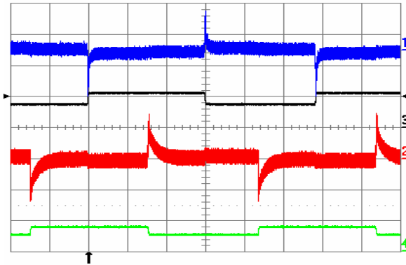
Fig. 24: Output voltage response to both Iout1 and Iout2 (out of phase) load current step-change of 3.75 A (Iout1) and 2.5 A (Iout2) (50%-75%-50%) at V_{in} = 48 V. Ch1 = Vout1 (50 mV/div), Ch2 = Vout2 (50 mV/div), Ch3 = Iout1 (10 A/div.), Ch4 = Iout2 (10 A/div.). Current slew rate: 0.1 A/ \mu s, C_o = 10 \mu F tantalum + 1 \mu F ceramic. Time scale: 1 ms/div.
