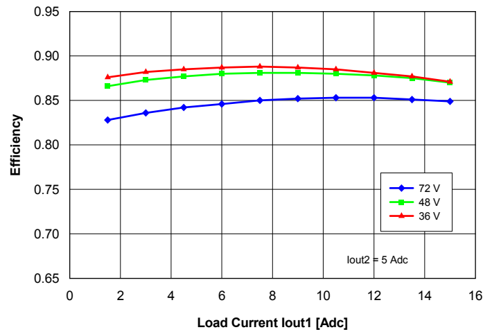
Fig. 13: Efficiency vs. load current Iout1 and input voltage for converter mounted horizontally with air flowing from pin 3 to pin 4 at a rate of 300 LFM (1.5 m/s), for Iout2 = 5 A and Ta = 25°C.
