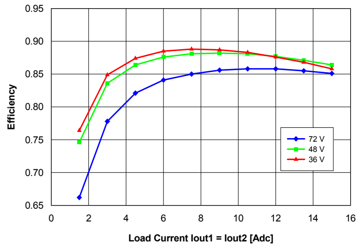
Fig. 17: Efficiency vs. balanced load current ( I_{out1}/I_{out2} = \text{const.} ) and input voltage for converter mounted horizontally with air flowing from pin 3 to pin 4 at a rate of 300 LFM (1.5 m/s) and T_a = 25^\circ\text{C} .
