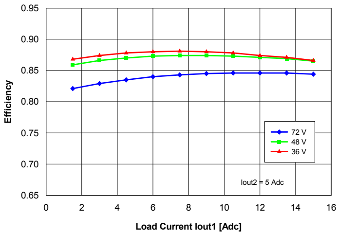
Fig. 12: Efficiency vs. load current Iout1 and input voltage for converter mounted vertically with air flowing from pin 3 to pin 1 at a rate of 300 LFM (1.5 m/s), for Iout2 = 5 A and Ta = 25°C.
