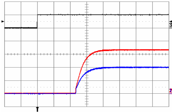
Fig. 18: Turn-on transient waveforms at no load current and V_{in} = 48\text{ V} , triggered via ON/OFF pin. Top trace: ON/OFF signal (5 V/div.). Bottom traces: V_{out1} (blue, 1 V/div.), V_{out2} (red, 1 V/div.). Time scale: 1 ms/div.
