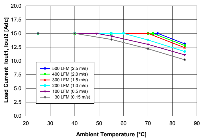
Fig. 11: Available balanced load current (I out1 = I out2 ) vs. ambient temperature and airflow rates for converter mounted horizontally with V in = 48 V, air flowing from pin 3 to pin 1 and maximum FET temperature ≤ 120°C.
