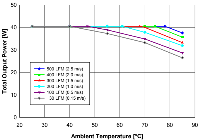
Fig. 1: Available output power vs. ambient air temperature and airflow rates for QD48S012015 converter mounted vertically with air flowing from pin 3 to pin 1, MOSFET temperature \leq 120^{\circ}\text{C} , V_{in} = 48\text{ V} and balanced load on both outputs ( I_{out1} = I_{out2} ).
