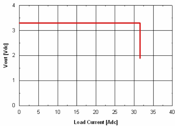
Fig. 15: Output voltage vs. load current showing typical current limit threshold and converter shutdown point. Input voltage has almost no effect on current limit characteristic.
