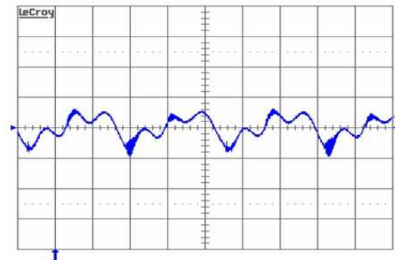
Fig. 11: Output voltage ripple (20 mV/div.) at full rated load current into a resistive load with C_o = 10 \mu F tantalum + 1 \mu F ceramic and V_{in} = 36 V. Time scale: 1 \mu s/div.
