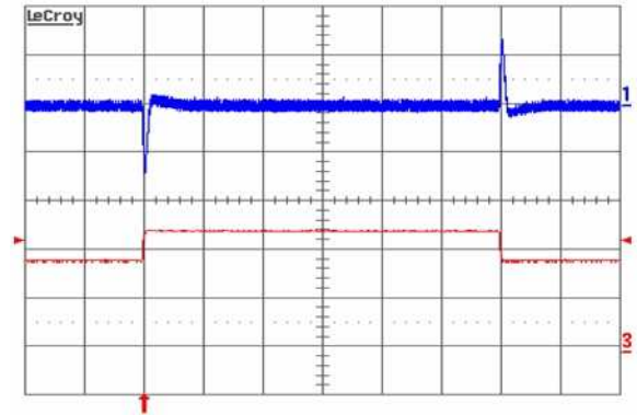
Fig. 10: Output voltage response to load current step-change (18.75 A – 25 A – 18.75 A) at V_{in} = 36 V. Top trace: output voltage (100 mV/div.). Bottom trace: load current (10 A/div.). Current slew rate: 1 A/ \mu s. C_o = 1 \mu F ceramic + 10 \mu F tantalum. Time scale: 0.2 ms/div.
