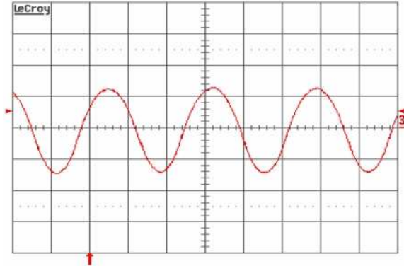
Fig. 13: Input reflected ripple current, i_c (100 mA/div.), measured at input terminals at full rated load current and V_{in} = 36 V. Refer to Fig. 12 for test setup. Time scale: 1 \mu s/div.
