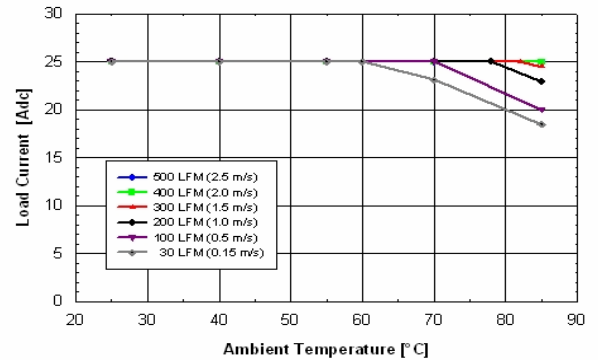
Fig. 2 : Available load current vs. ambient air temperature and airflow rates for converter with G height pins mounted vertically with air flowing from pin 1 to pin 3, MOSFET temperature \leq 125\text{ }^{\circ}\text{C} , V_{in} = 48\text{ V} .
