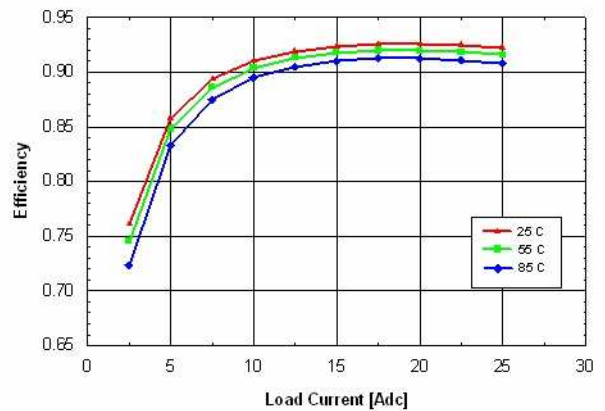
Fig. 4 : Efficiency vs. load current and ambient temperature for converter mounted vertically with V_{in} = 36\text{ V} and air flowing from pin 1 to pin 3 at a rate of 200 LFM (1.0 m/s).
