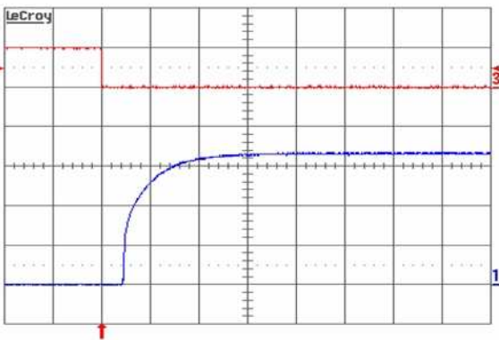
Fig. 7: Turn-on transient at full rated load current (resistive) with no output capacitor at V_{in} = 36\text{ V} , triggered via ON/OFF pin. Top trace: ON/OFF signal (5 V/div.). Bottom trace: output voltage (1 V/div.). Time scale: 2 ms/div.
