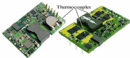
Fig. H: Location of the thermocouples for thermal testing.
