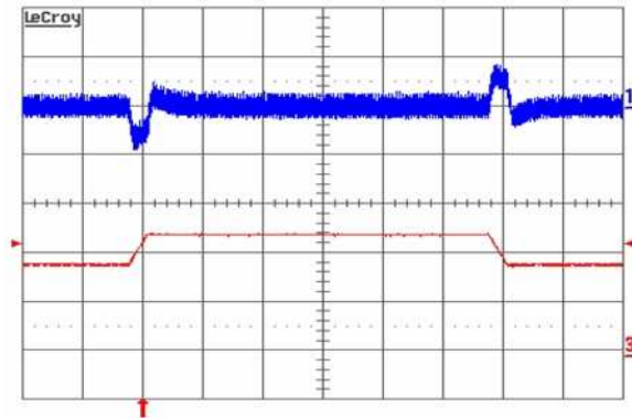
Fig. 9: Output voltage response to load current step-change (18.75 A – 25 A – 18.75 A) at V_{in} = 36 V. Top trace: output voltage (50 mV/div.). Bottom trace: load current (10 A/div.). Current slew rate: 0.1 A/ \mu s. C_o = 1 \mu F ceramic + 10 \mu F tantalum. Time scale: 0.2 ms/div.
