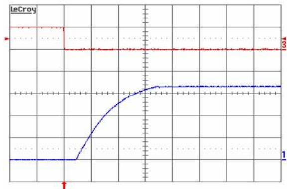
Fig. 8: Turn-on transient at full rated load current (resistive) plus 20,000 \mu\text{F} at V_{in} = 36\text{ V} , triggered via ON/OFF pin. Top trace: ON/OFF signal (5 V/div.). Bottom trace: output voltage (1 V/div.). Time scale: 2 ms/div.
