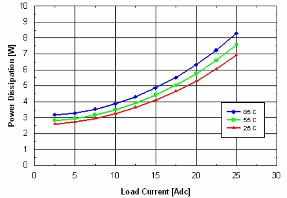
Fig. 6: Power dissipation vs. load current and ambient temperature for converter mounted vertically with V_{in} = 36\text{ V} and air flowing from pin 1 to pin 3 at a rate of 200 LFM (1.0 m/s).
