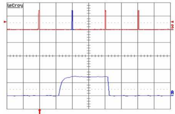
Fig. 16: Load current (top trace, 20 A/div., 100 ms/div.) into a 10 m\Omega short circuit during restart, at V_{in} = 36 V. Bottom trace (20 A/div., 2 ms/div.) is an expansion of the on-time portion of the top trace.
