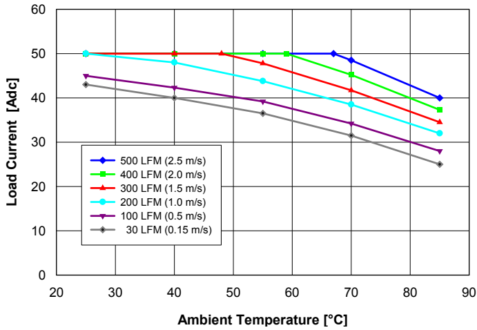
Fig. 1: Available load current vs. ambient air temperature and airflow rates for QM48T50018 converter with B height pins mounted vertically with air flowing from pin 3 to pin 1, MOSFET temperature \leq 120^{\circ}\text{C} , V_{in} = 48\text{ V} .
