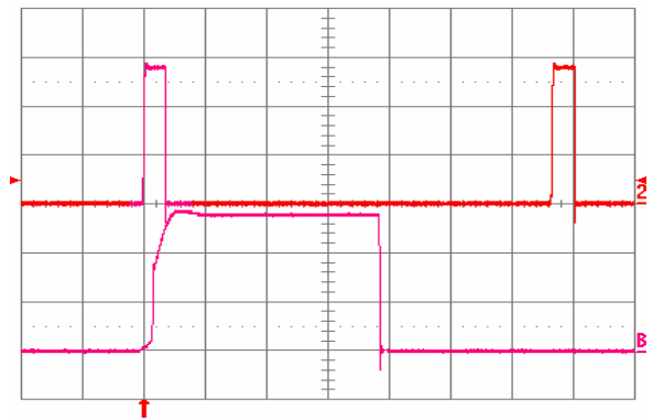
Fig. 13: Load current (top trace, 20 A/div, 20 ms/div) into a 10 m \Omega short circuit during restart, at V_{in} = 48 V. Bottom trace (20 A/div, 2 ms/div) is an expansion of the on-time portion of the top trace.
