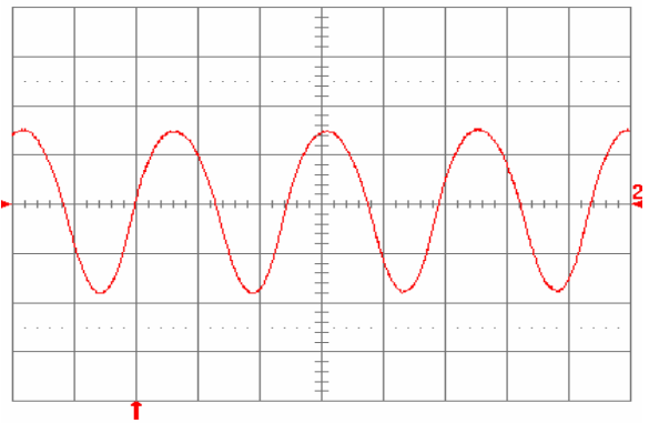
Fig. 11: Input reflected ripple current, i_c (100 mA/div), measured at input terminals at full rated load current and V_{in} = 48 V. Refer to Fig. 9 for test setup. Time scale: 1 \mu s/div.
