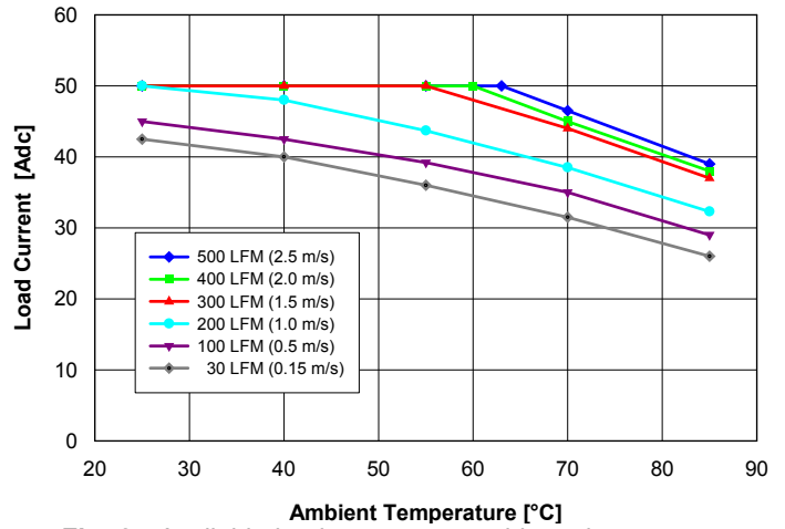
Fig. 2: Available load current vs. ambient air temperature and airflow rates for QM48T50018 converter with B height pins mounted horizontally with air flowing from pin 3 to pin 1, MOSFET temperature \leq 120^{\circ}\text{C} , V_{in} = 48\text{ V} .
