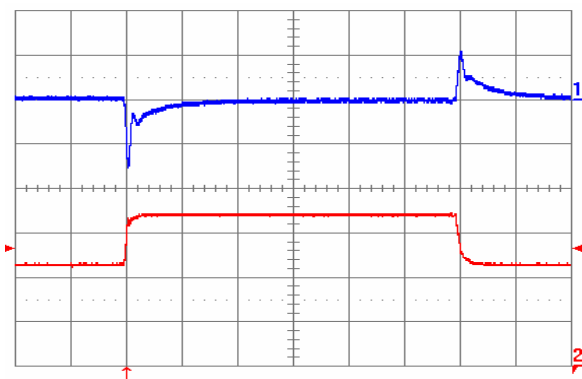
Fig. 7: Output voltage response to load current step-change (22.5 A – 33.75 A – 22.5 A) at V_{in} = 48\text{ V} . Top trace: output voltage (100 mV/div.). Bottom trace: load current (10 A/div.). Current slew rate: 1 A/ \mu\text{s} . C_o = 470\ \mu\text{F} tantalum + 1 \mu\text{F} ceramic. Time scale: 0.2 ms/div.
