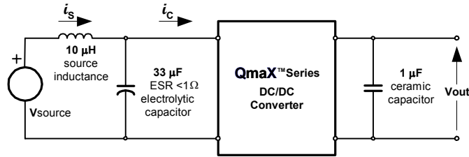
Fig. 9: Test Set-up for measuring input reflected ripple currents, i_c and i_s .
