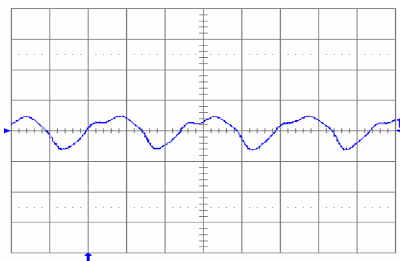
Fig. 8: Output voltage ripple (20 mV/div.) at full rated load current into a resistive load with C_o = 10\ \mu\text{F} tantalum + 1 \mu\text{F} ceramic and V_{in} = 48\text{ V} . Time scale: 1 \mu\text{s} /div.
