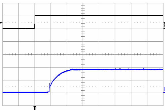
Fig. 6: Turn-on transient at full rated load current (resistive) plus 40,000 \mu\text{F} at V_{in} = 48\text{ V} , triggered via ON/OFF pin. Top trace: ON/OFF signal (5 V/div.). Bottom trace: output voltage (1 V/div.). Time scale: 2 ms/div.
