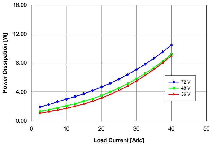
Fig. 1.0V.5: Power dissipation vs. load current and input voltage for converter mounted vertically with air flowing from pin 3 to pin 1 at a rate of 300 LFM (1.5 m/s) and T_a = 25\text{ }^{\circ}\text{C} .
