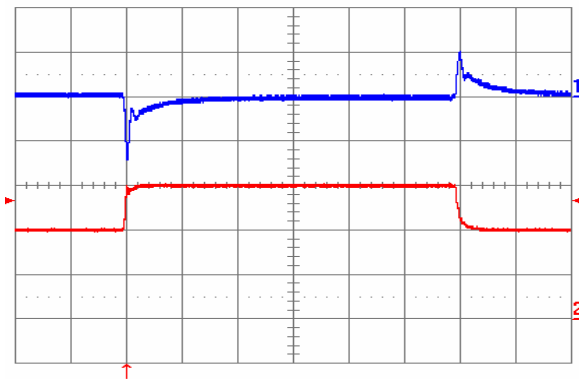
Fig. 2.5V.9: Output voltage response to load current step-change (20 A – 30 A – 20 A) at V_{in} = 48 V. Top trace: output voltage (100 mV/div.). Bottom trace: load current (10 A/div.). Current slew rate: 1 A/ \mu s. C_o = 470 \mu F tantalum + 1 \mu F ceramic. Time scale: 0.2 ms/div.
