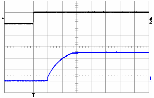
Fig. 10: Turn-on transient at full rated load current (resistive) plus 10,000 \mu F at V_{in} = 48 V, triggered via ON/OFF pin. Top trace: ON/OFF signal (5 V/div.). Bottom trace: output voltage (2 V/div.). Time scale: 2 ms/div.
