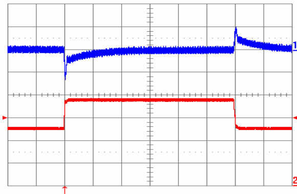
Fig. 11: Output voltage response to load current step-change (12.5 A – 18.75 A – 12.5 A) at V_{in} = 48 V. Top trace: output voltage (100 mV/div.). Bottom trace: load current (5 A/div.). Current slew rate: 1 A/ \mu s. C_o = 470 \mu F tantalum + 1 \mu F ceramic. Time scale: 0.2 ms/div.
