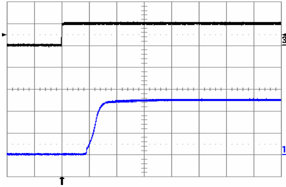
Fig. 9: Turn-on transient at full rated load current (resistive) with no output capacitor at V_{in} = 48 V, triggered via ON/OFF pin. Top trace: ON/OFF signal (5 V/div.). Bottom trace: output voltage (2 V/div.). Time scale: 2 ms/div.
