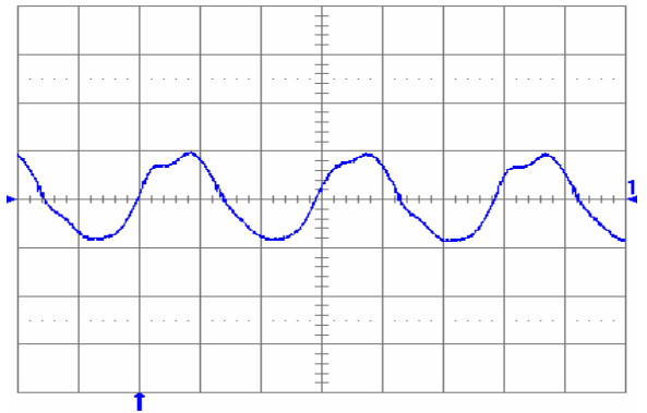
Fig. 12: Output voltage ripple (20 mV/div.) at full rated load current into a resistive load with C_o = 10 \mu F tantalum + 1 \mu F ceramic and V_{in} = 48 V. Time scale: 1 \mu s/div.
