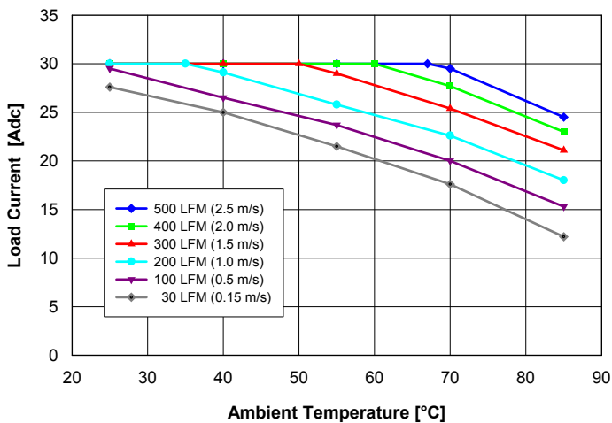
Fig. 1: Available load current vs. ambient air temperature and air-flow rates for Q48T30033 converter mounted vertically with air flowing from pin 3 to pin 1, MOSFET temperature \leq 120^{\circ}\text{C} , V_{in} = 54\text{ V} .
