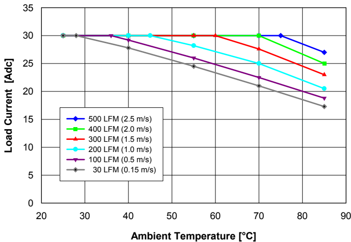
Fig. 1: Available load current vs. ambient air temperature and air-flow rates for Q48T30025 converter mounted vertically with air flowing from pin 3 to pin 1, MOSFET temperature \leq 120^{\circ}\text{C} , V_{in} = 54\text{ V} .
