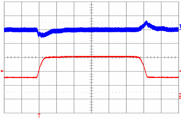
Fig. 20: Output voltage response to load current step-change (7.5 A – 15 A – 7.5 A) at V_{in} = 48\text{ V} . Top trace: output voltage (100 mV/div.). Bottom trace: load current (5 A/div.). Current slew rate: 0.1 A/ \mu\text{s} . C_o = 1\text{ }\mu\text{F} ceramic. Time scale: 0.2 ms/div.
