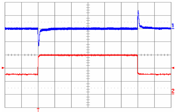
Fig. 21: Output voltage response to load current step-change (7.5 A – 15 A – 7.5 A) at V_{in} = 48\text{ V} . Top trace: output voltage (100 mV/div.). Bottom trace: load current (5 A/div.). Current slew rate: 5 A/ \mu\text{s} . C_o = 450\text{ }\mu\text{F} tantalum + 1 \mu\text{F} ceramic. Time scale: 0.2 ms/div.
