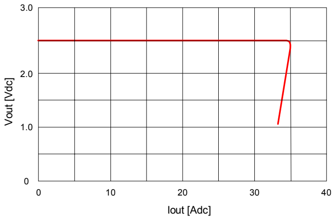
Fig. 26: Output voltage vs. load current showing current limit point and converter shutdown point. Input voltage has almost no effect on current limit characteristic.
