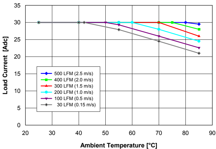
Fig. 1: Available load current vs. ambient air temperature and air-flow rates for Q48T30015 converter mounted vertically with air flowing from pin 3 to pin 1, MOSFET temperature \leq 120^{\circ}\text{C} , V_{in} = 54\text{ V} .
