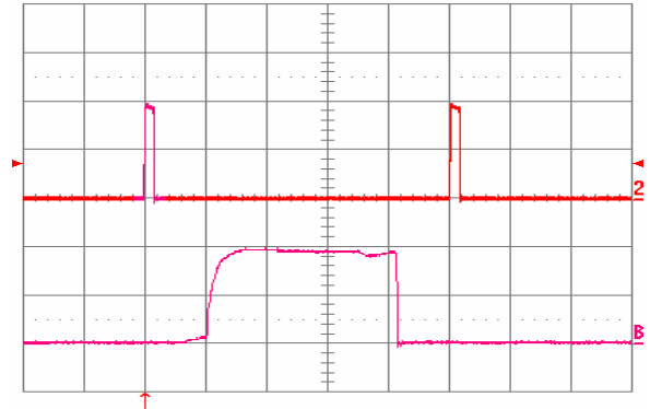
Fig. 27: Load current (top trace, 20 A/div, 20 ms/div) into a 10 mΩ short circuit during restart, at Vin = 48 V. Bottom trace (20 A/div, 1 ms/div) is an expansion of the on-time portion of the top trace.
