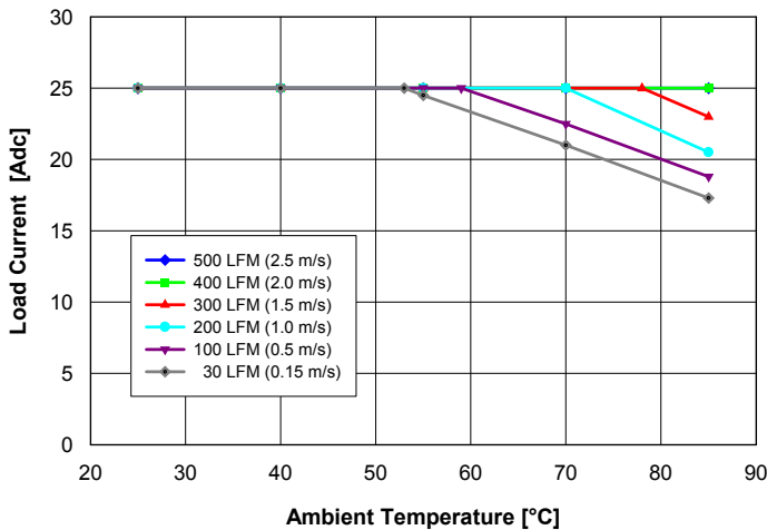
Fig. 1: Available load current vs. ambient air temperature and air-flow rates for Q48T25025 converter mounted vertically with air flowing from pin 3 to pin 1, MOSFET temperature \leq 120^{\circ}\text{C} , V_{in} = 54\text{ V} .
