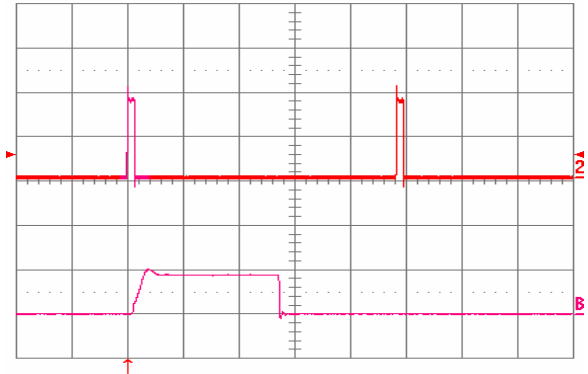
Fig. 27: Load current (top trace, 20 A/div, 20 ms/div) into a 10 mΩ short circuit during restart, at V_{in} = 48 V. Bottom trace (40 A/div, 1 ms/div) is an expansion of the on-time portion of the top trace.
