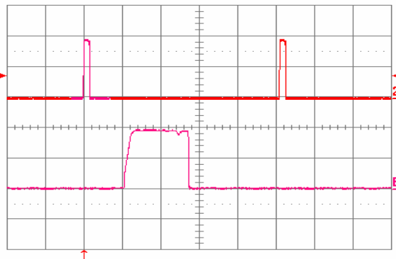
Fig. 27: Load current (top trace, 20 A/div, 20 ms/div) into a 10 mΩ short circuit during restart, at V_{in} = 48 V. Bottom trace (20 A/div, 1 ms/div) is an expansion of the on-time portion of the top trace.
