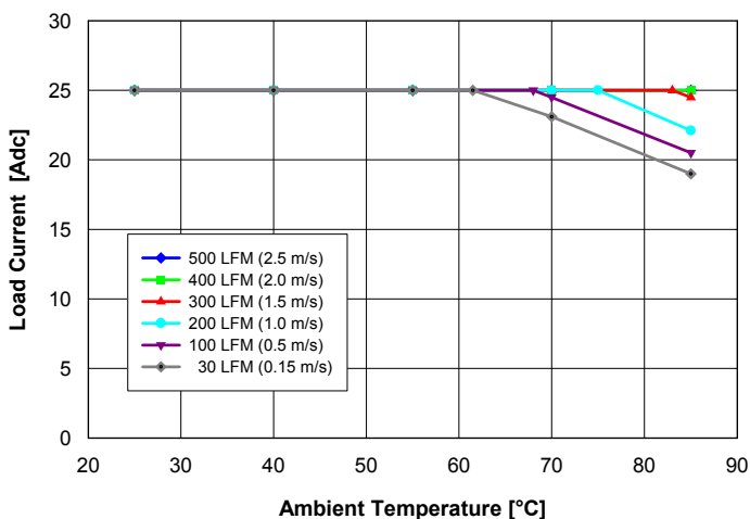
Fig. 1: Available load current vs. ambient air temperature and air flow rates for Q48T25020 converter mounted vertically with air flowing from pin 3 to pin 1, MOSFET temperature \leq 120^{\circ}\text{C} , V_{in} = 54\text{ V} .
