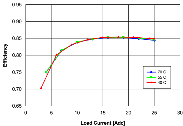
Fig. 17: Efficiency vs. load current and ambient temperature for converter mounted horizontally with V_{in} = 54\text{ V} and air flowing from pin 3 to pin 4 at a rate of 200 LFM (1.0 m/s).
