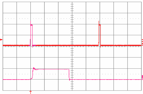
Fig. 27: Load current (top trace, 20 A/div, 20 ms/div) into a 10 mΩ short circuit during restart, at V_{in} = 48 V. Bottom trace (40 A/div, 1 ms/div) is an expansion of the on-time portion of the top trace.
