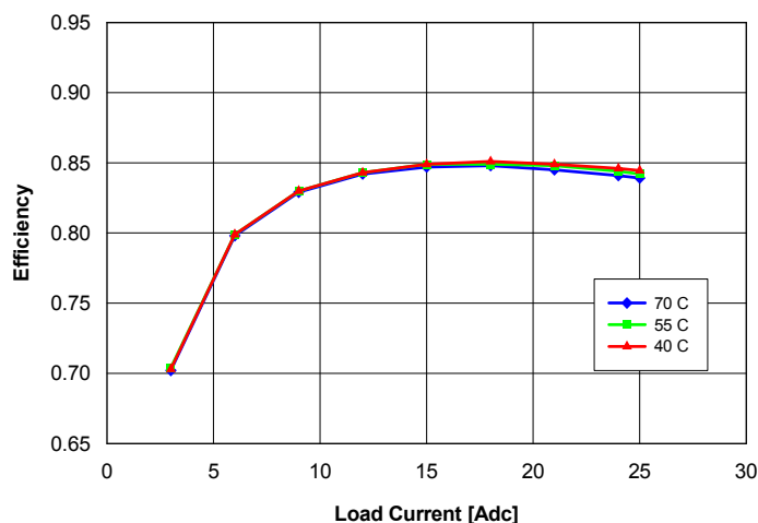
Fig. 15: Efficiency vs. load current and ambient temperature for converter mounted vertically with V_{in} = 54\text{ V} and air flowing from pin 3 to pin 1 at a rate of 200 LFM (1.0 m/s).
