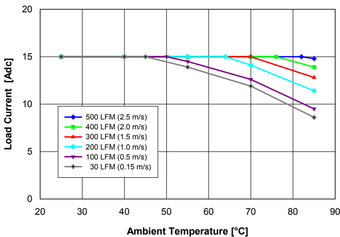
Fig. 1: Available load current vs. ambient air temperature and air-flow rates for Q48T15050 converter mounted vertically with air flowing from pin 3 to pin 1, MOSFET temperature \leq 120^{\circ}\text{C} , V_{in} = 54\text{ V} .
